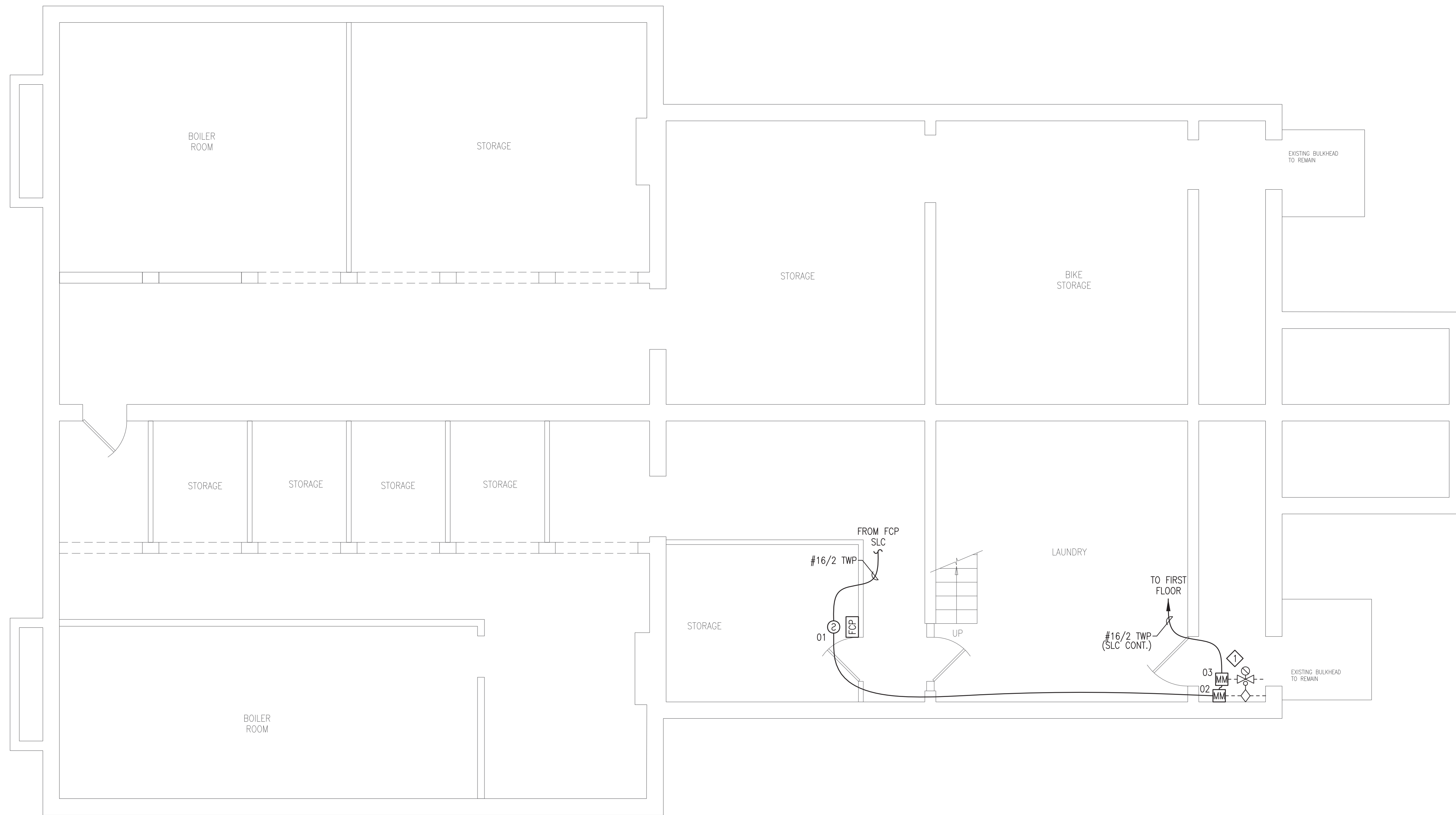
BASEMENT FIRE ALARM PLAN SCALE: 1/4"=1'-0"
