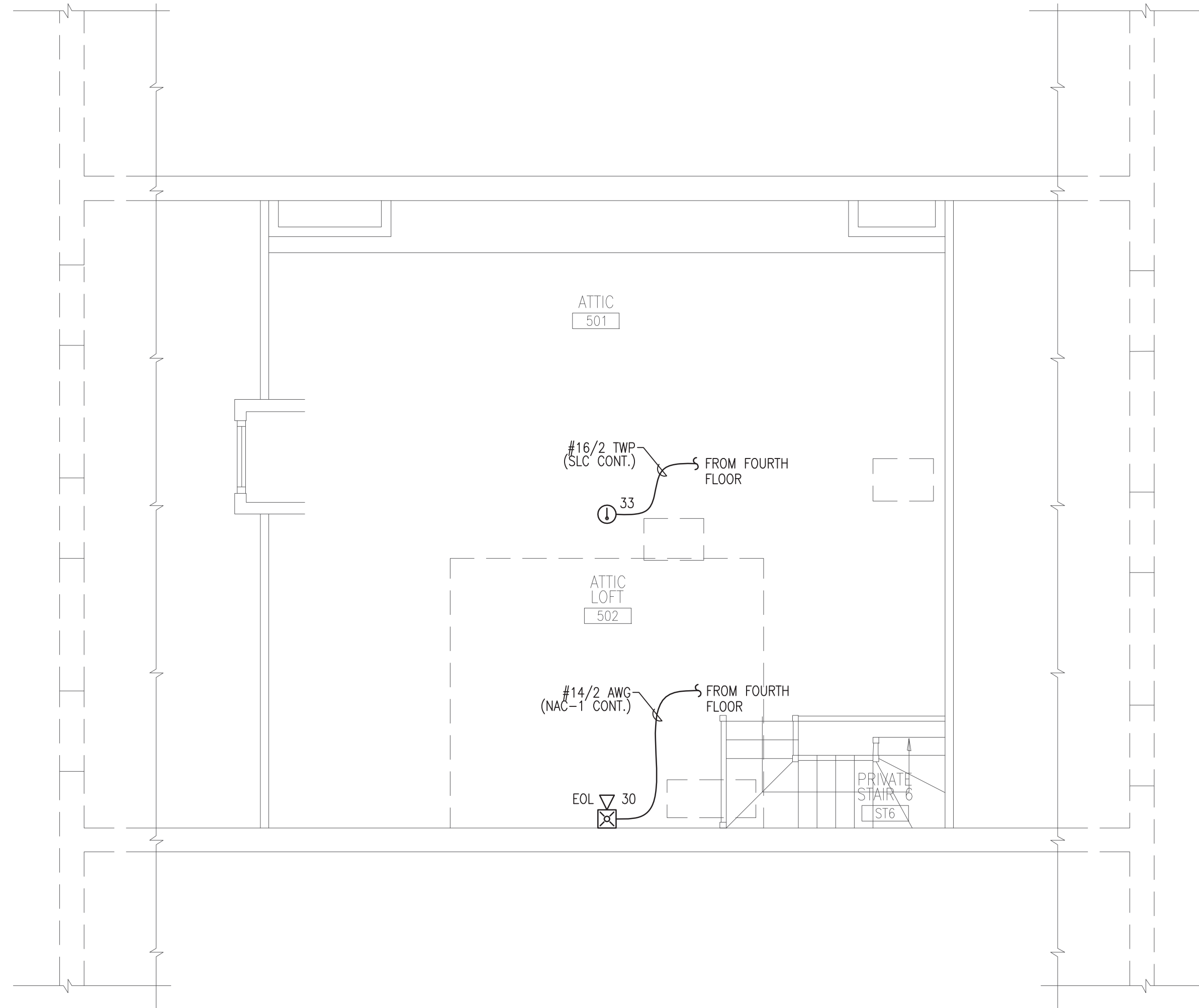
FIFTH FLOOR/ATTIC FIRE ALARM PLAN SCALE: 1/4"=1'-0"
