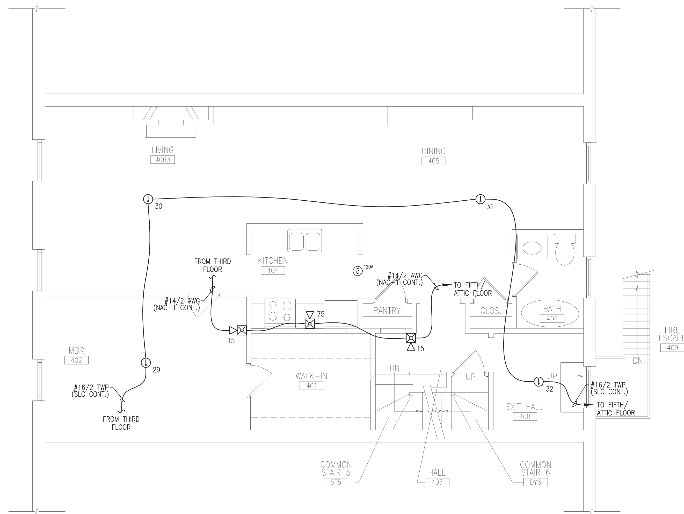
FOURTH FLOOR FIRE ALARM PLAN SCALE: 1/4"=1'-0"
