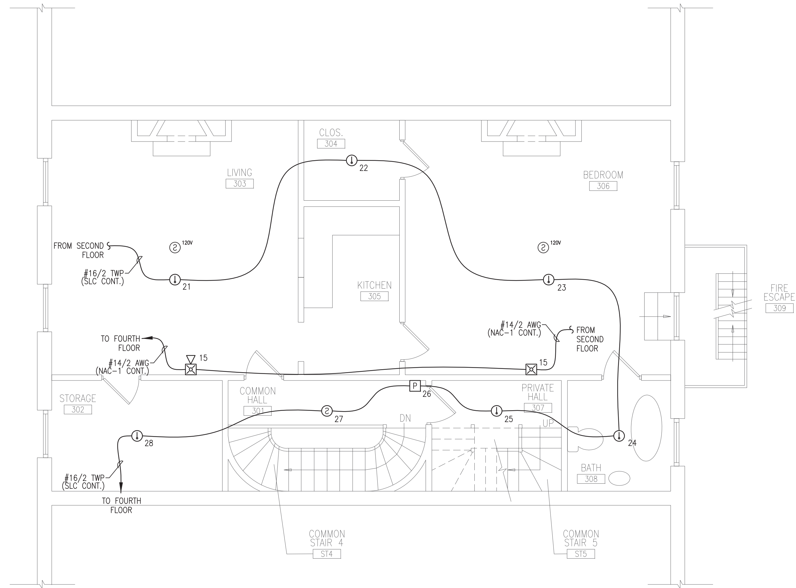
THIRD FLOOR FIRE ALARM PLAN SCALE: 1/4"=1'-0"
