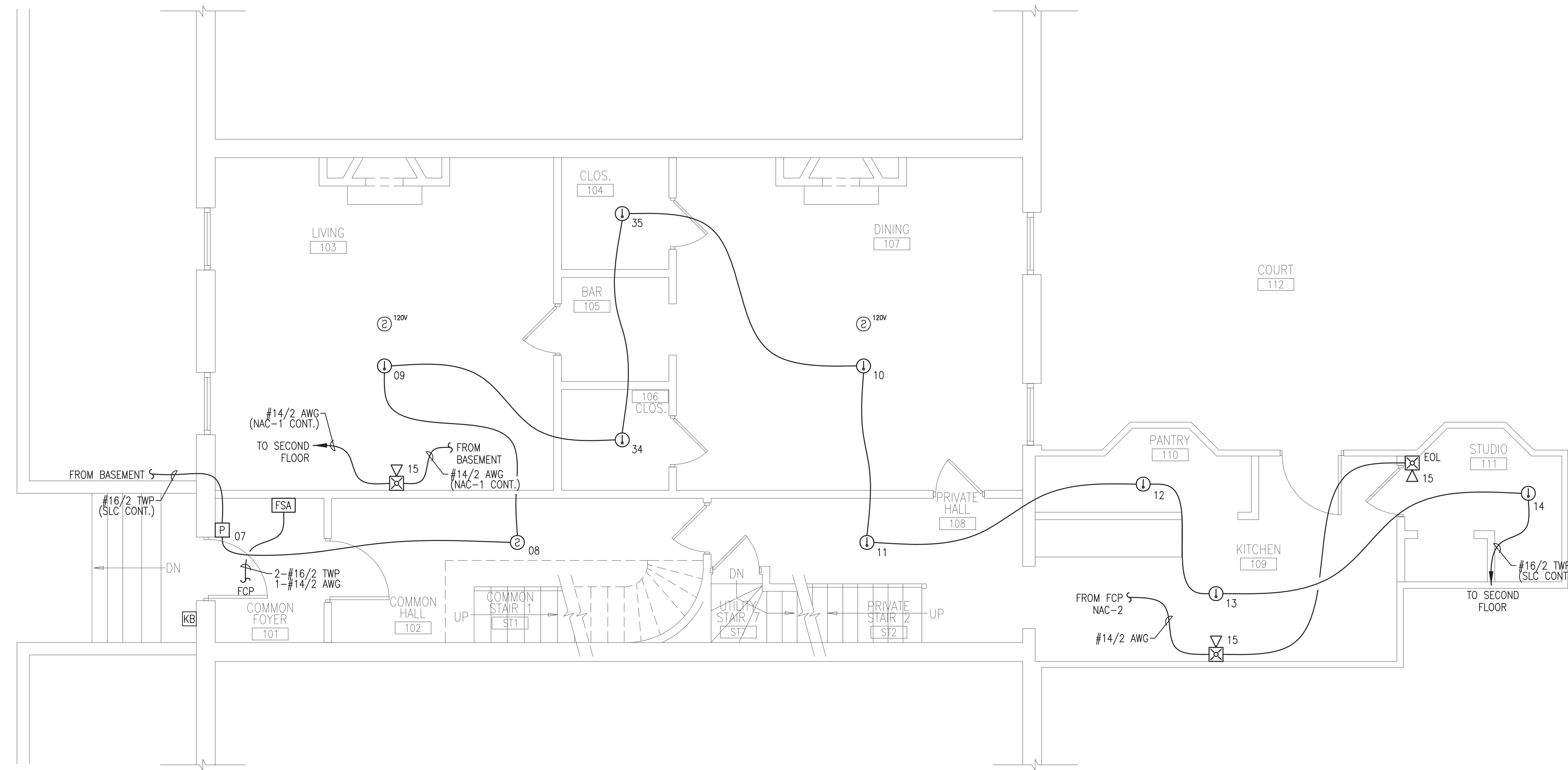
FIRST FLOOR FIRE ALARM PLAN SCALE: 1/4"=1'-0"
