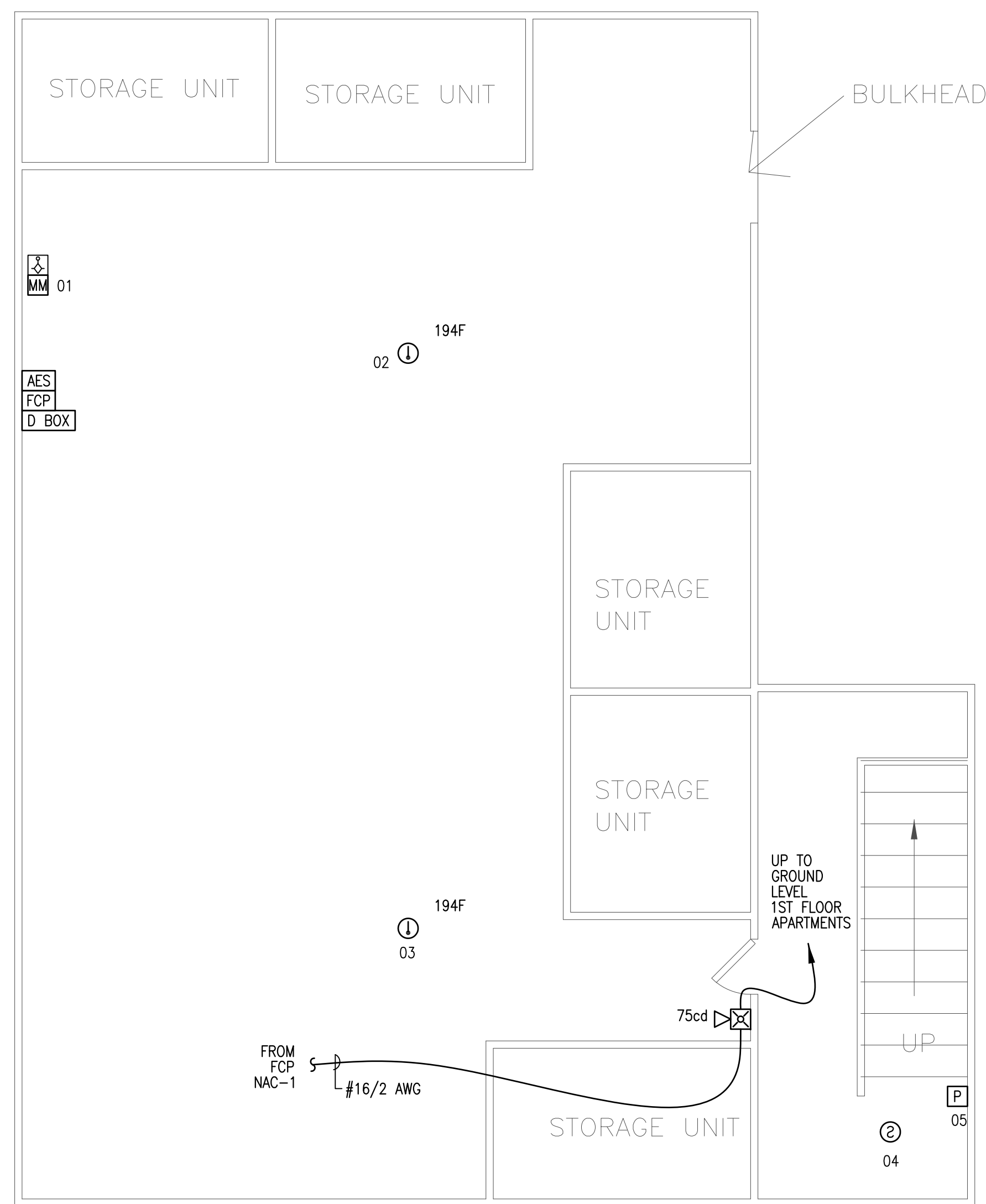
BASEMENT LEVEL FIRE ALARM PLAN SCALE: 1/4"=1'-0"
