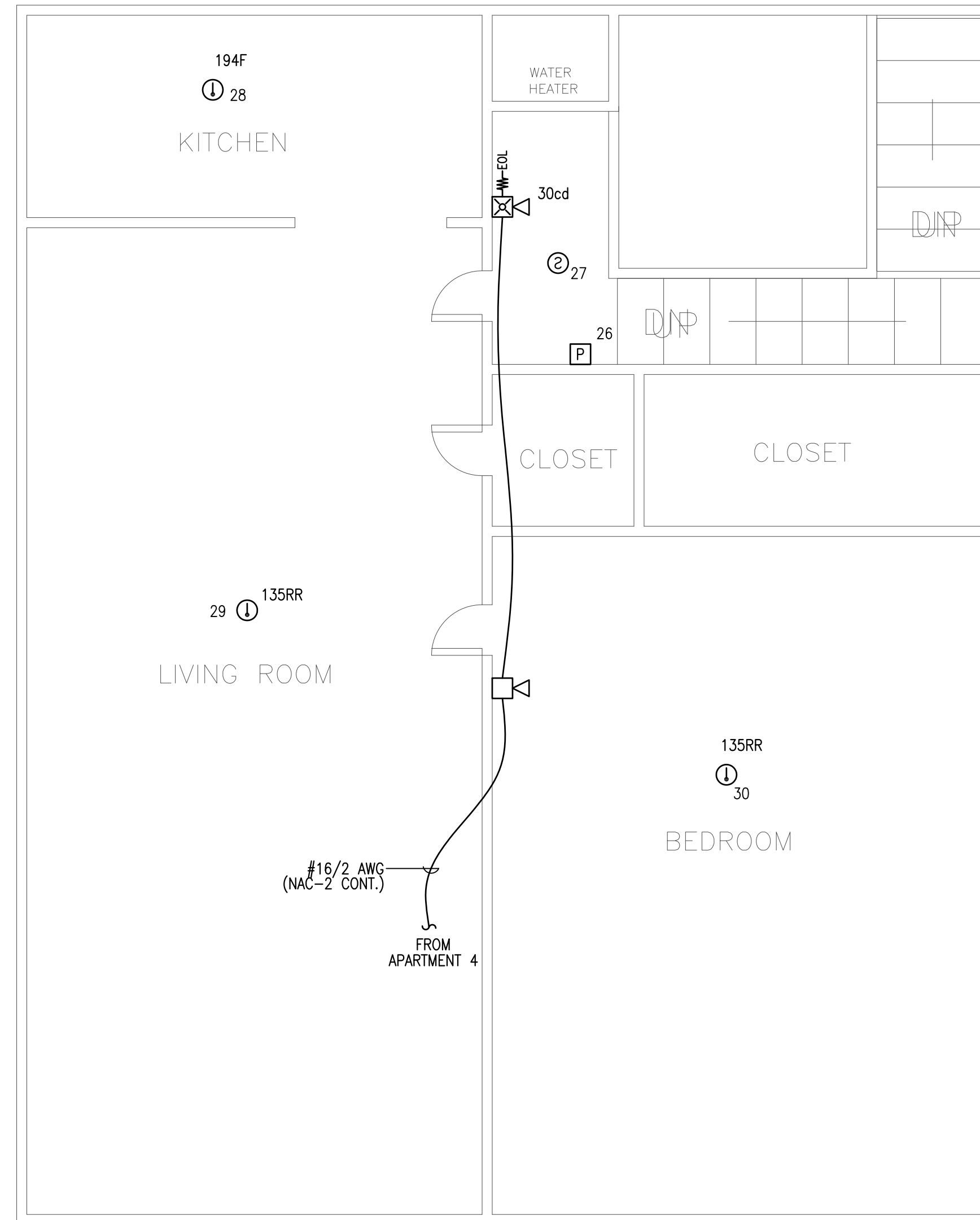
FIFTH FLOOR APARTMENT 5 FIRE ALARM PLAN SCALE: 1/4"=1'-0"
