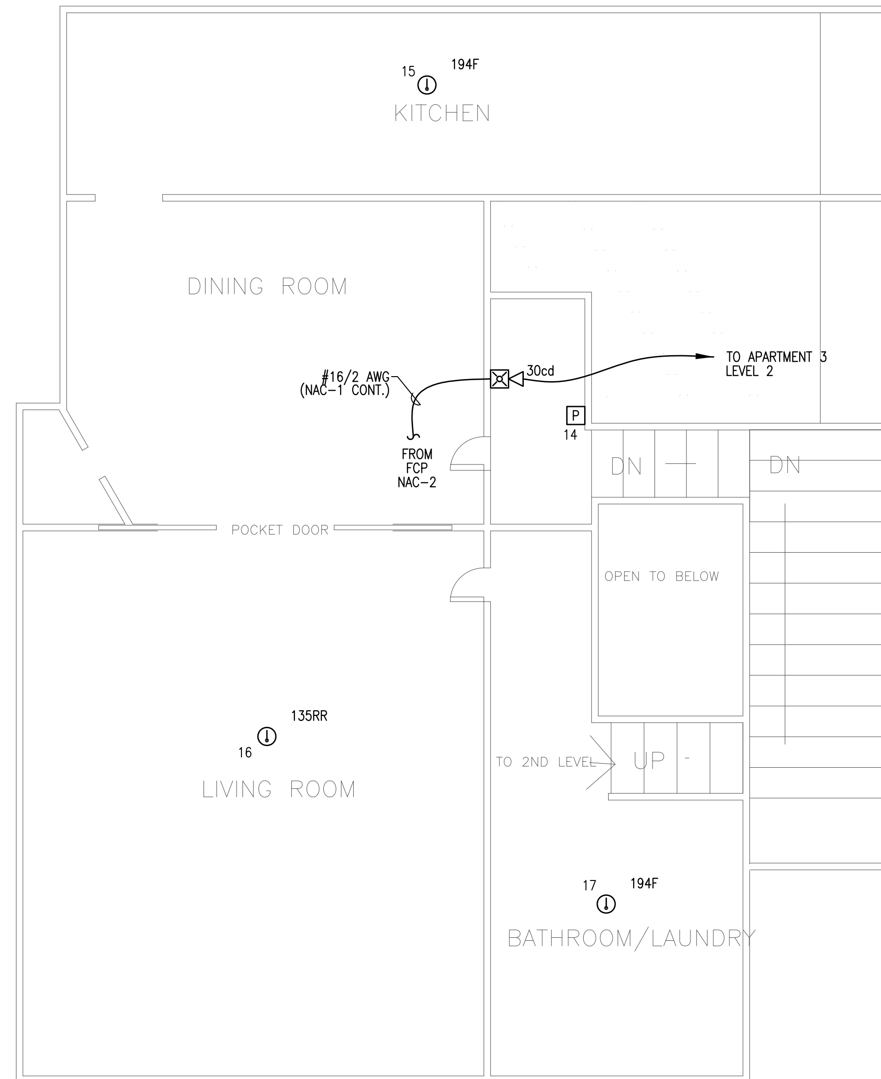
SECOND FLOOR LEVEL 1 FIRE ALARM PLAN SCALE: 1/4"=1'-0"
