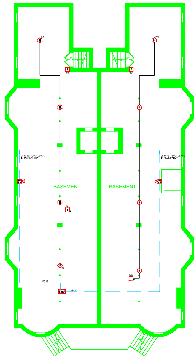
FIRE ALARM SYSTEM LAYOUT – BASEMENT
