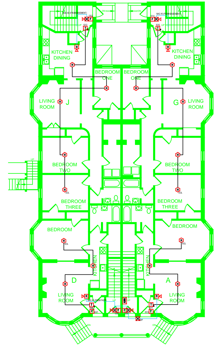
FIRE ALARM SYSTEM LAYOUT – FIRST FLOOR
