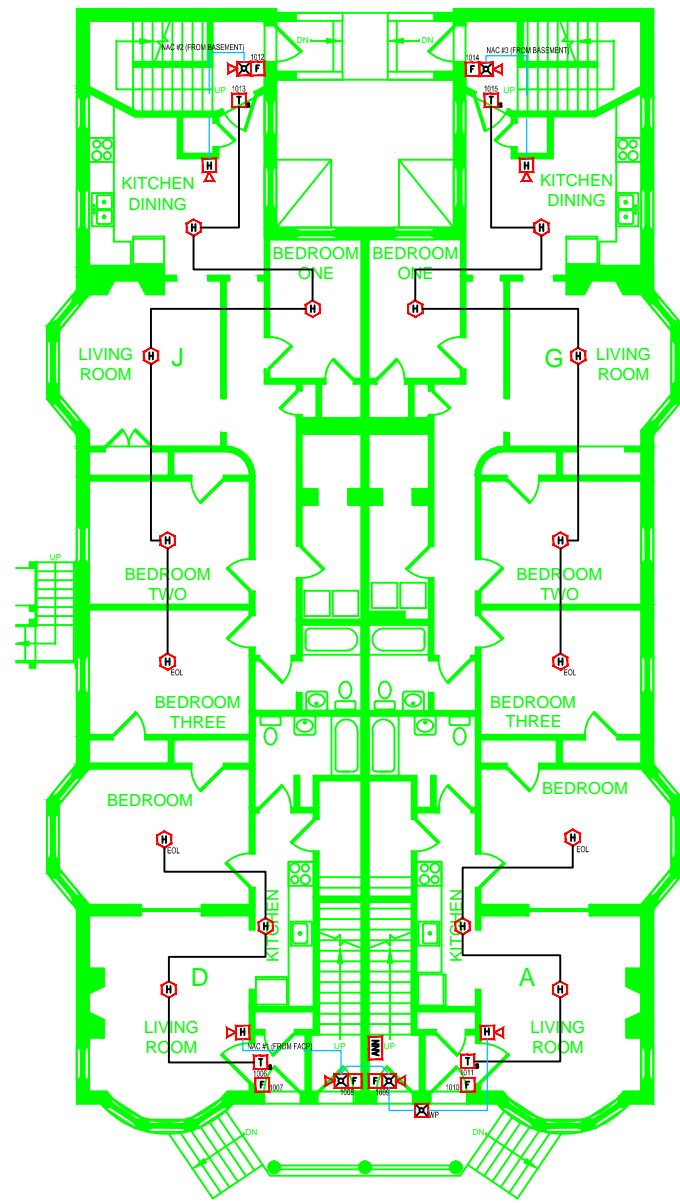
FIRE ALARM SYSTEM LAYOUT – FIRST FLOOR
