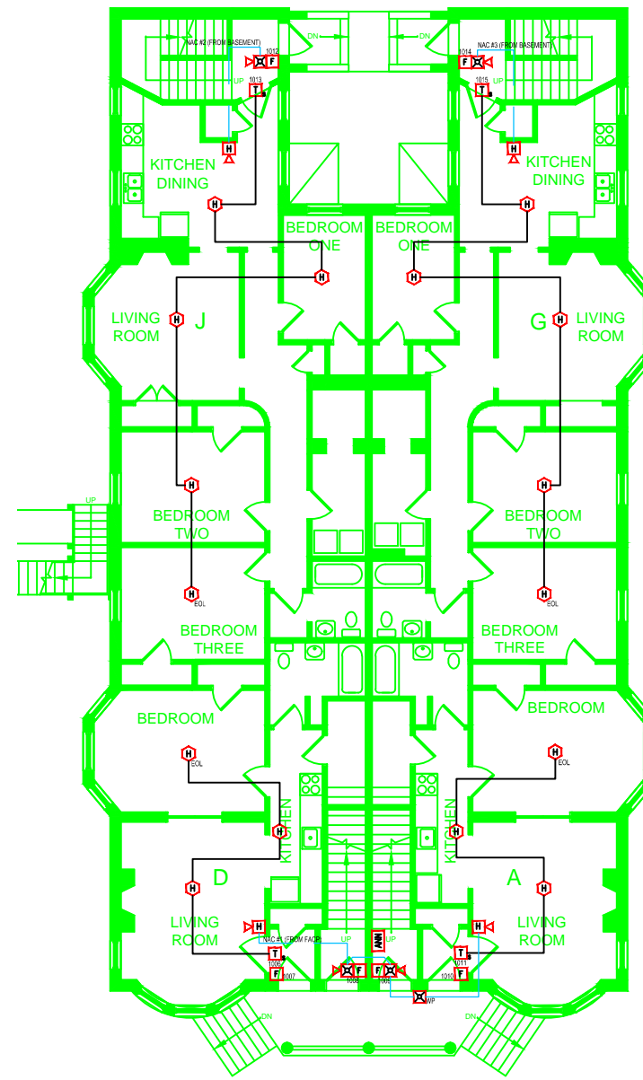
FIRE ALARM SYSTEM LAYOUT – FIRST FLOOR
