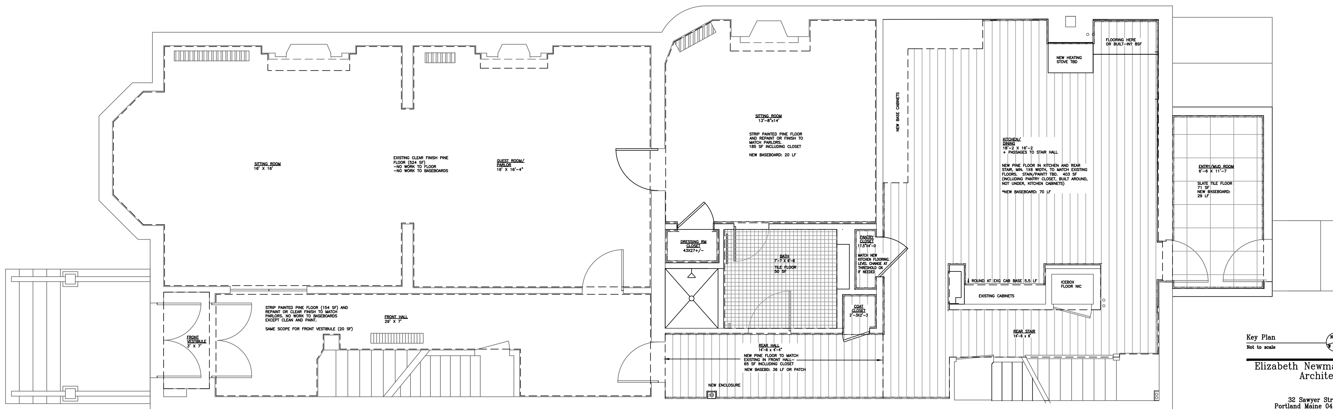
1 FIRST FLOOR FLOORING PLAN 1/4"=1'-0" 0 1 2 3 4 5 10 15
