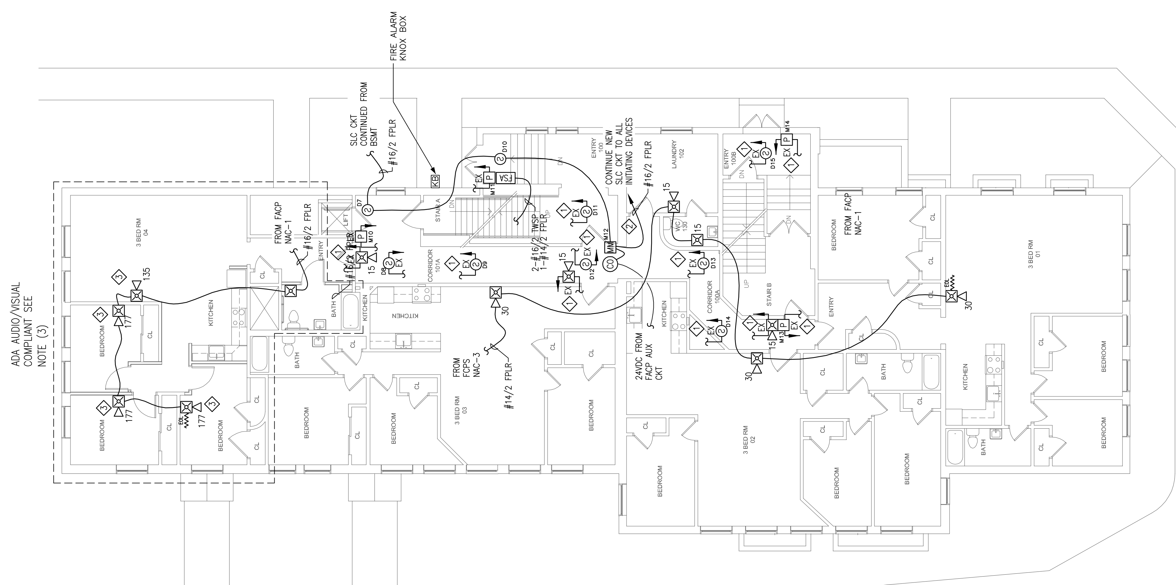
1ST FLOOR FIRE ALARM PLAN SCALE: 1/8"=1'-0"
