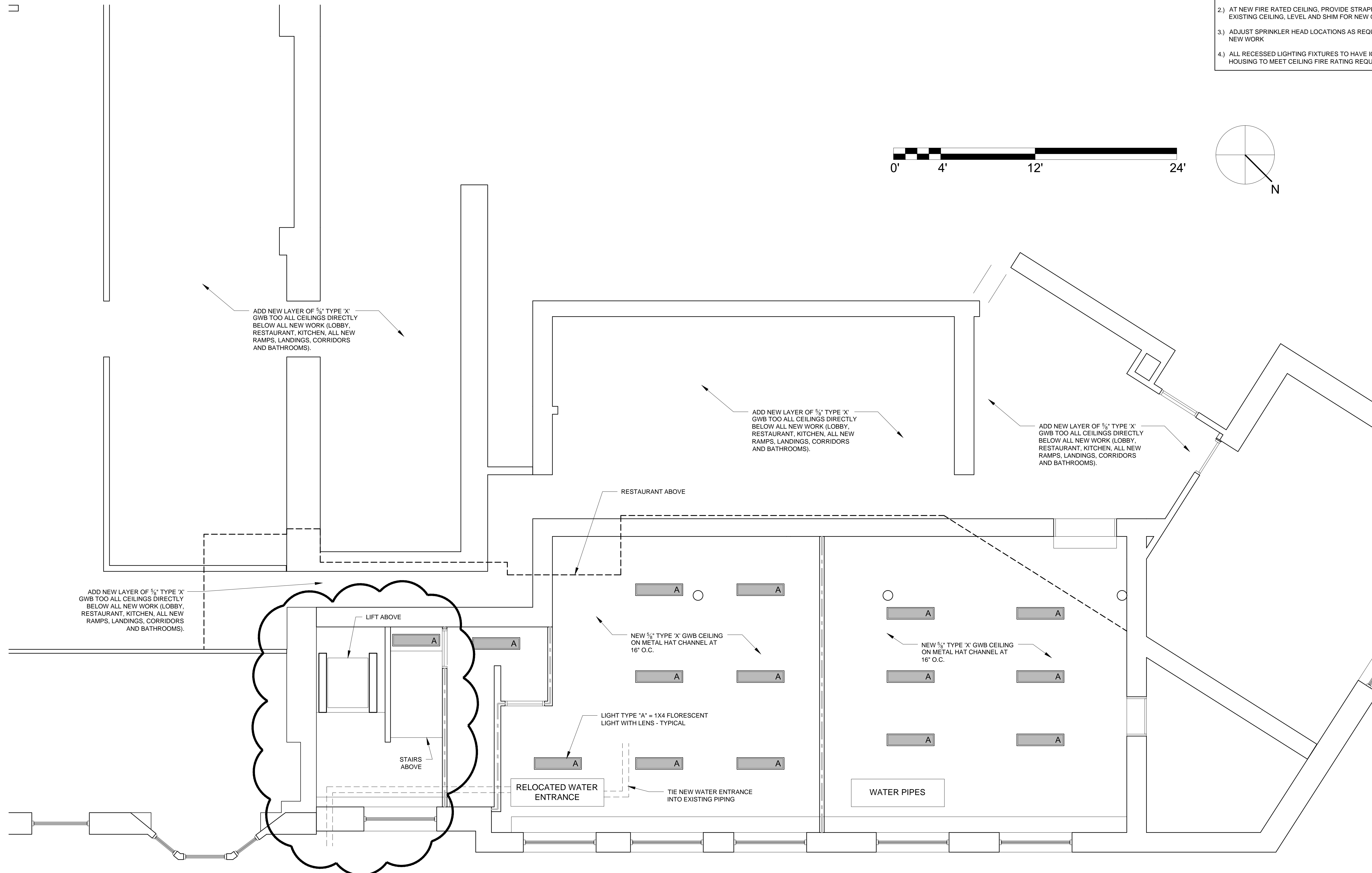
1 BASEMENT REFLECTED CEILING PLAN 1/4" = 1'-0"
