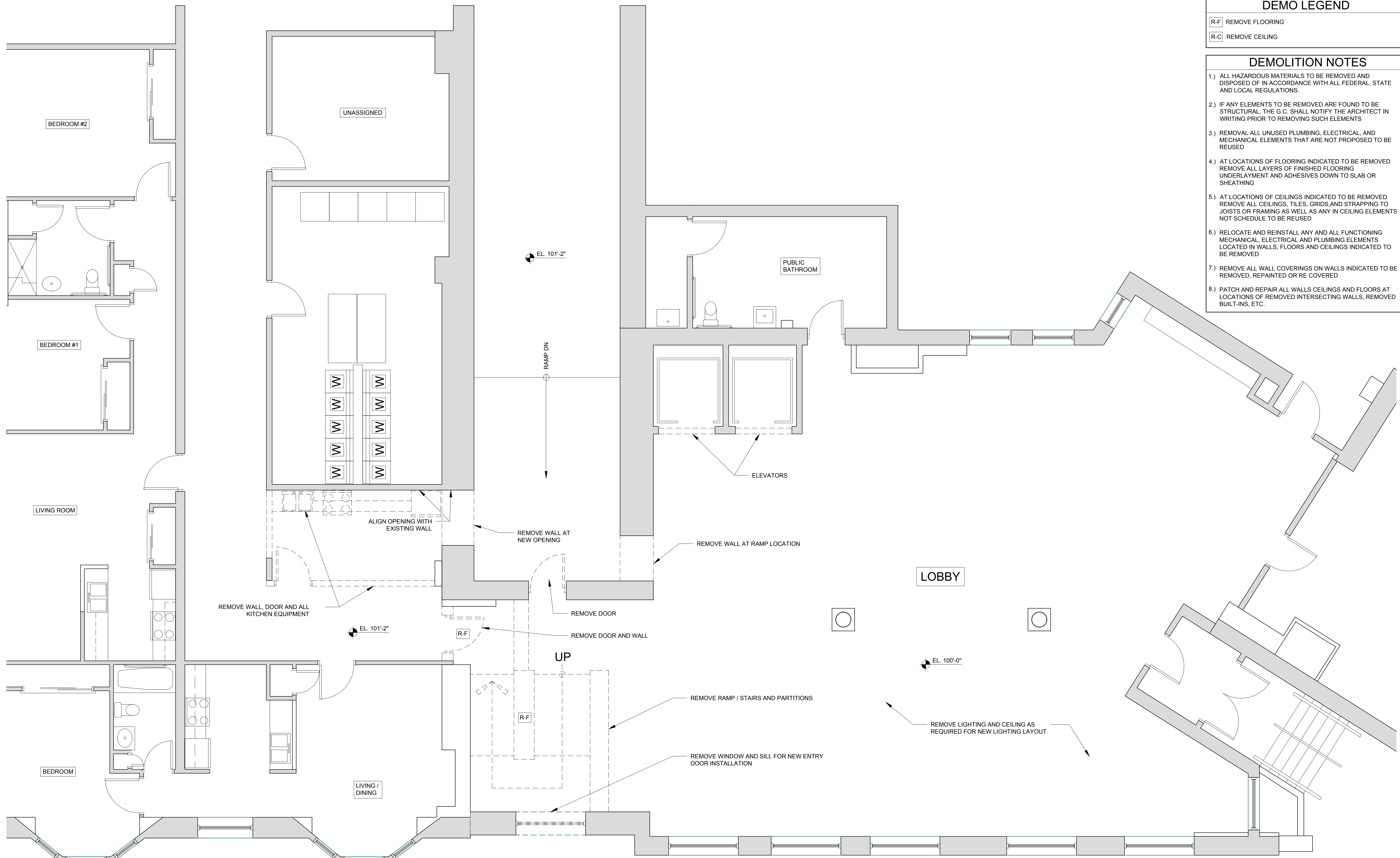
1 FIRST FLOOR DEMO PLAN 1/4" = 1'-0"
