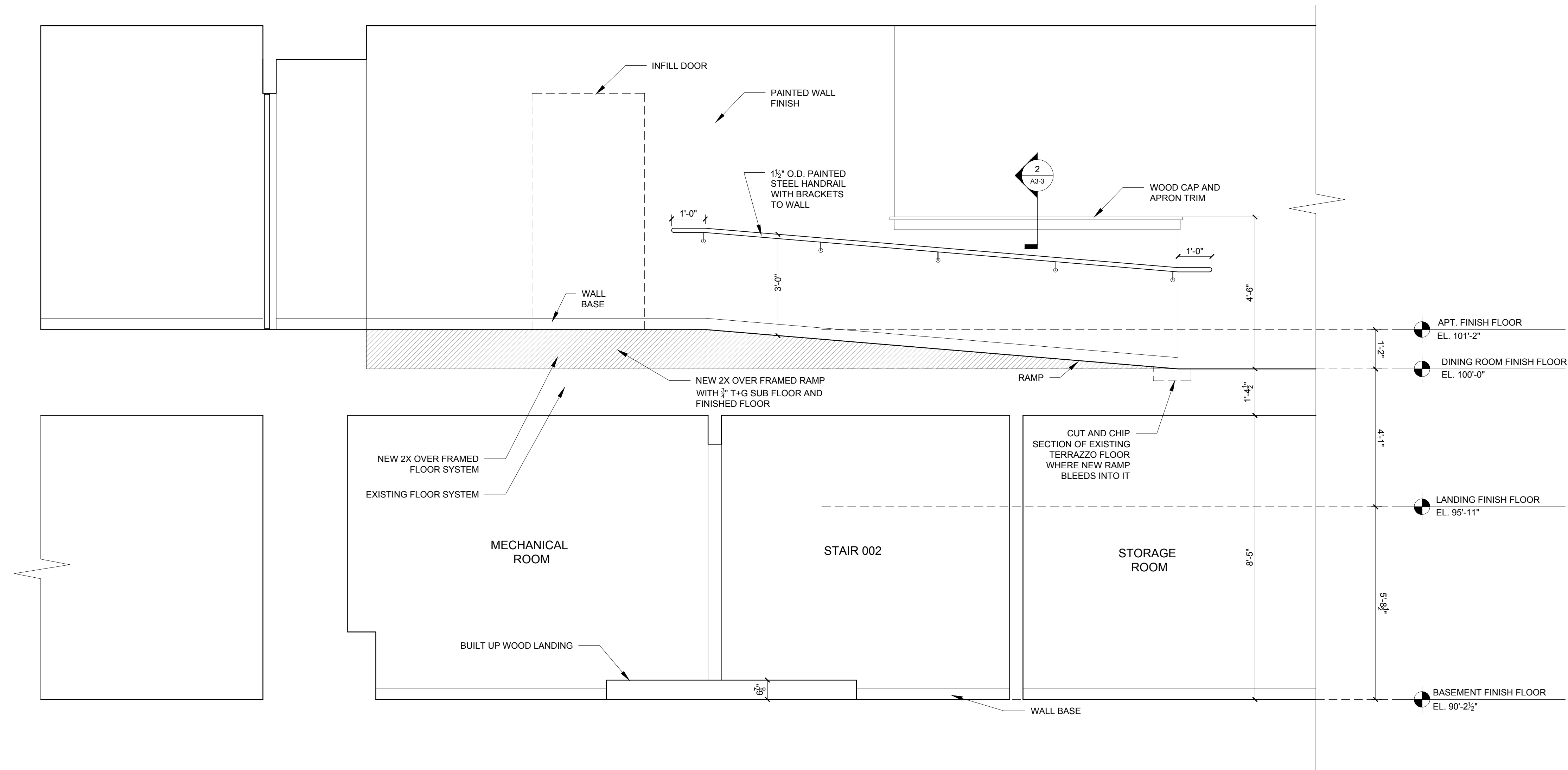
1 SECTION AT BASEMENT LANDING 1/2" = 1'-0"
