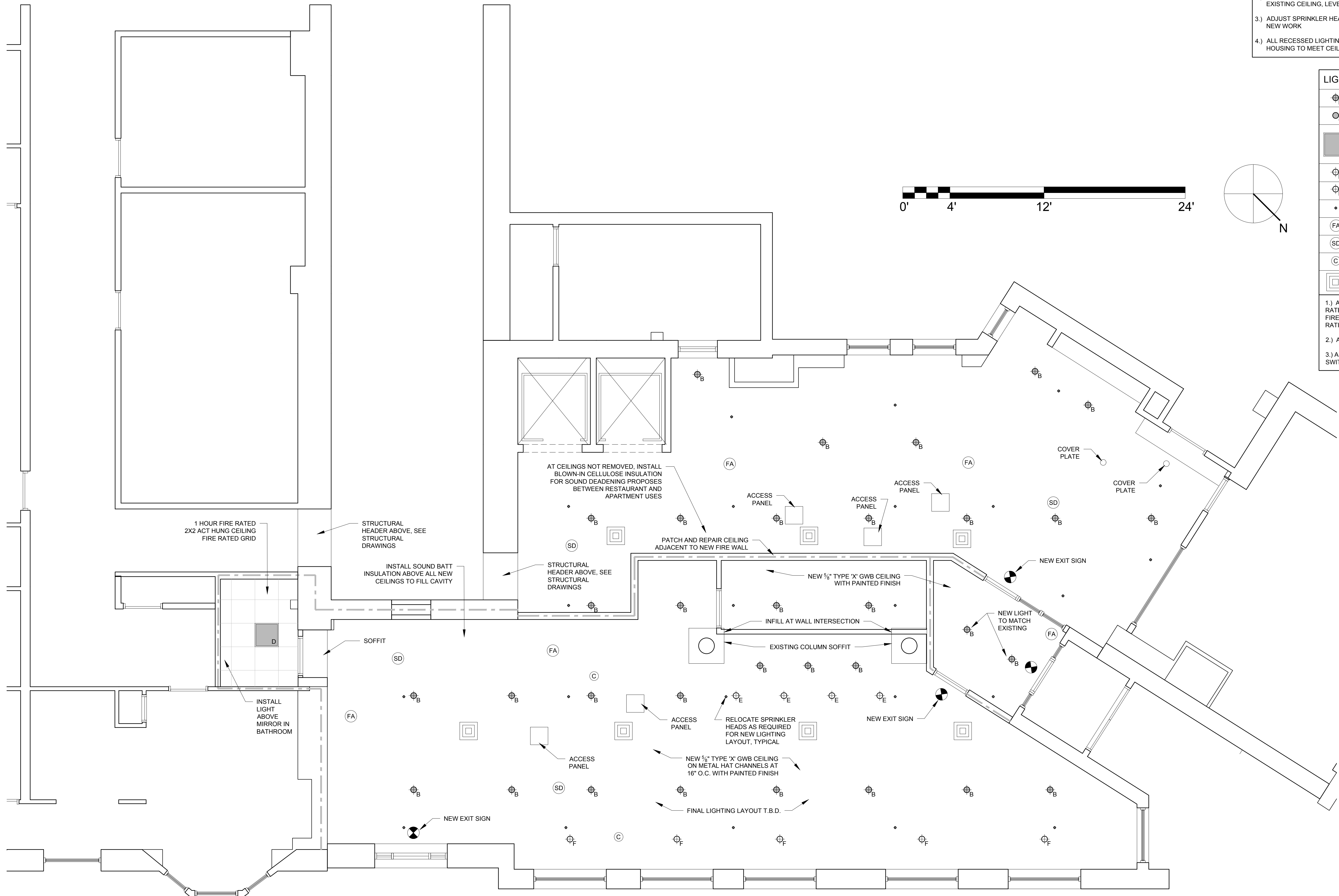
1 FIRST FLOOR REFLECTED CEILING PLAN 1/4" = 1'-0"
