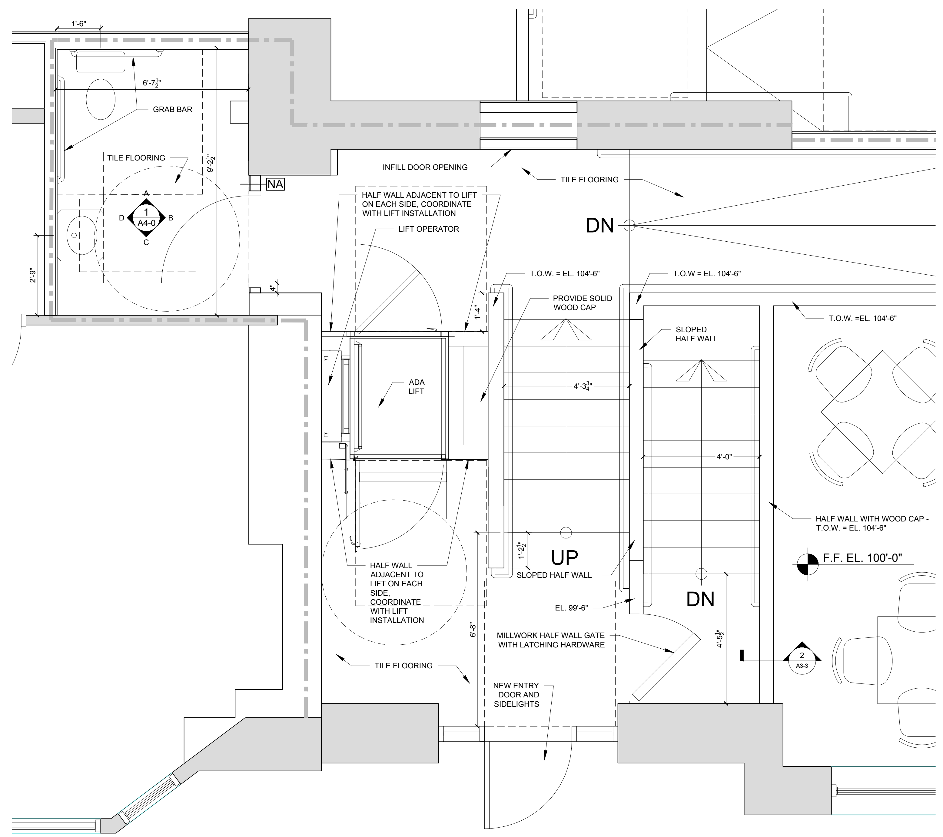
1 ENLARGED PLAN 1/2" = 1'-0"
