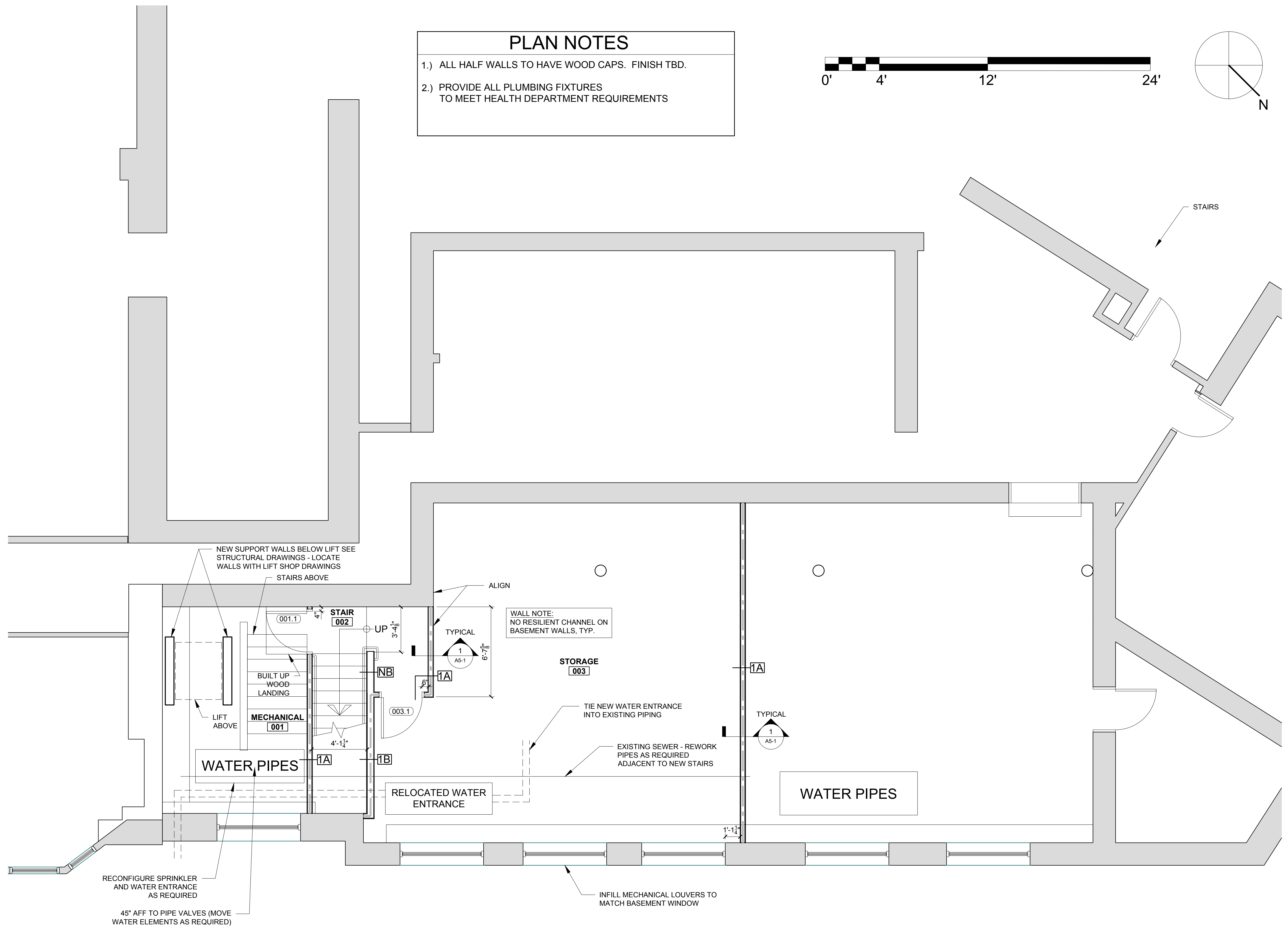
1 BASEMENT FLOOR PLAN 1/4" = 1'-0"
