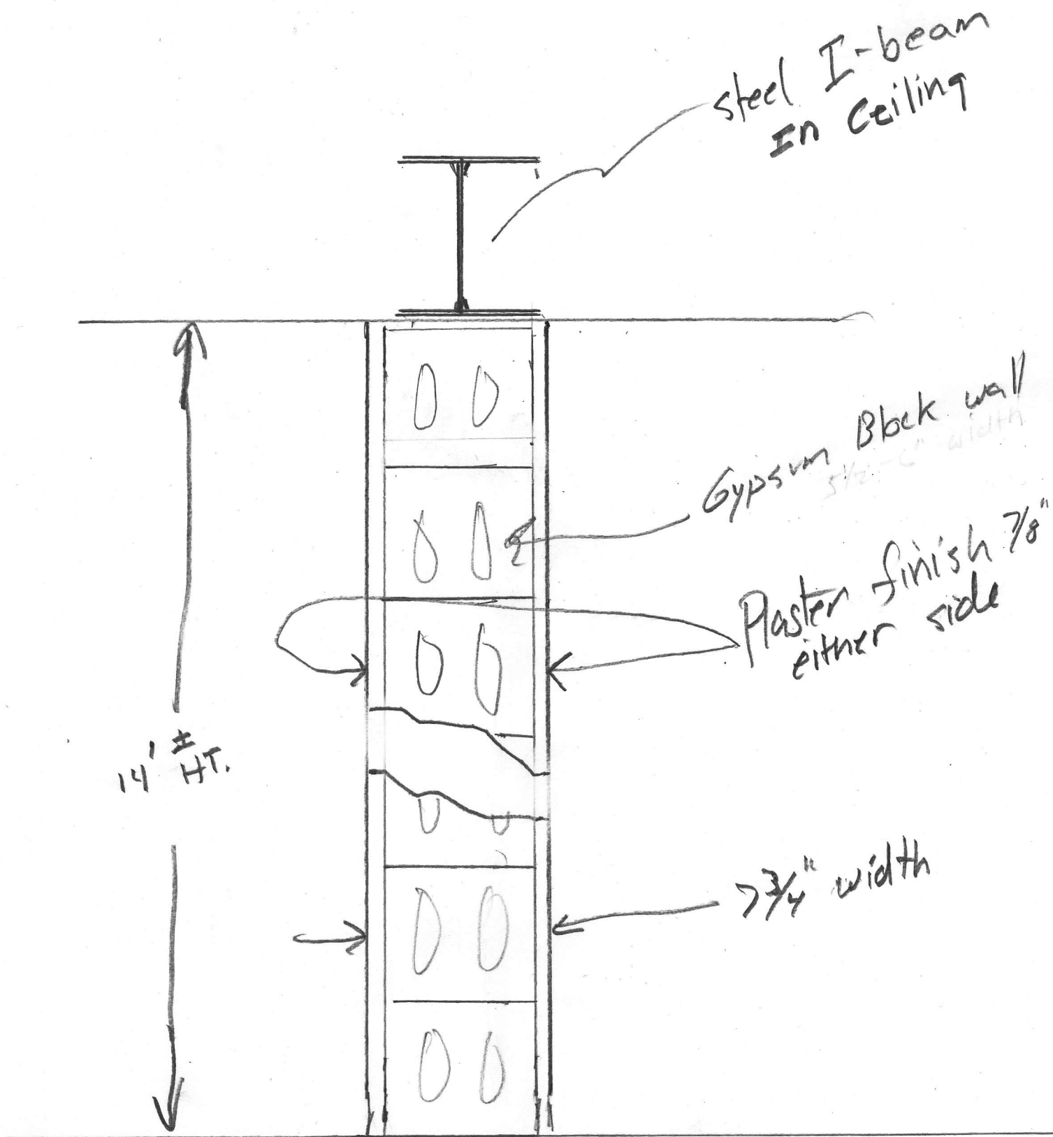
Elevation plan of wall
