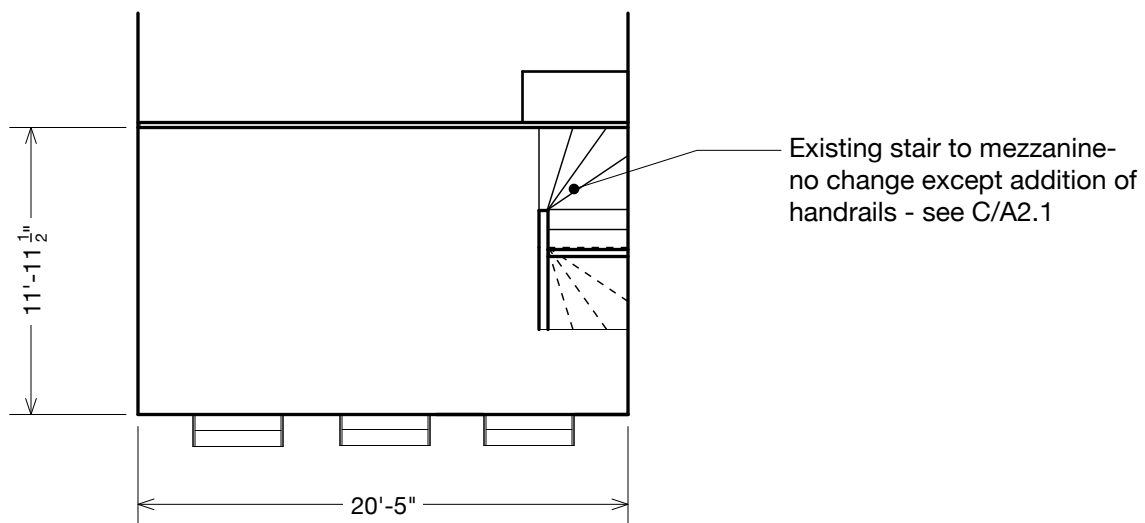
Existing Mezzanine Plan
