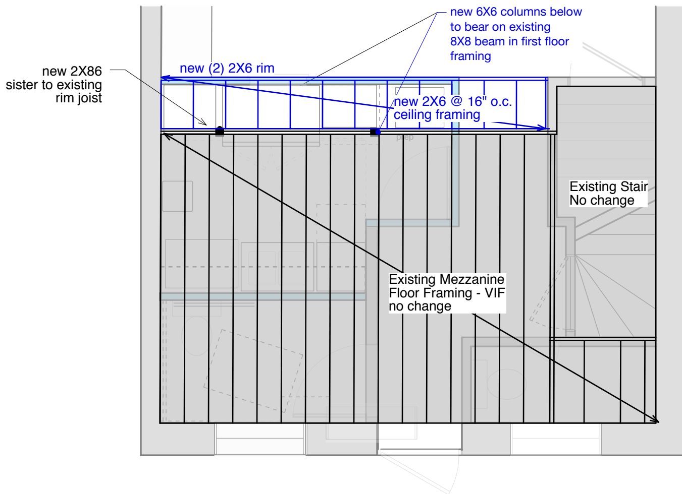
Mezzanine Framing
