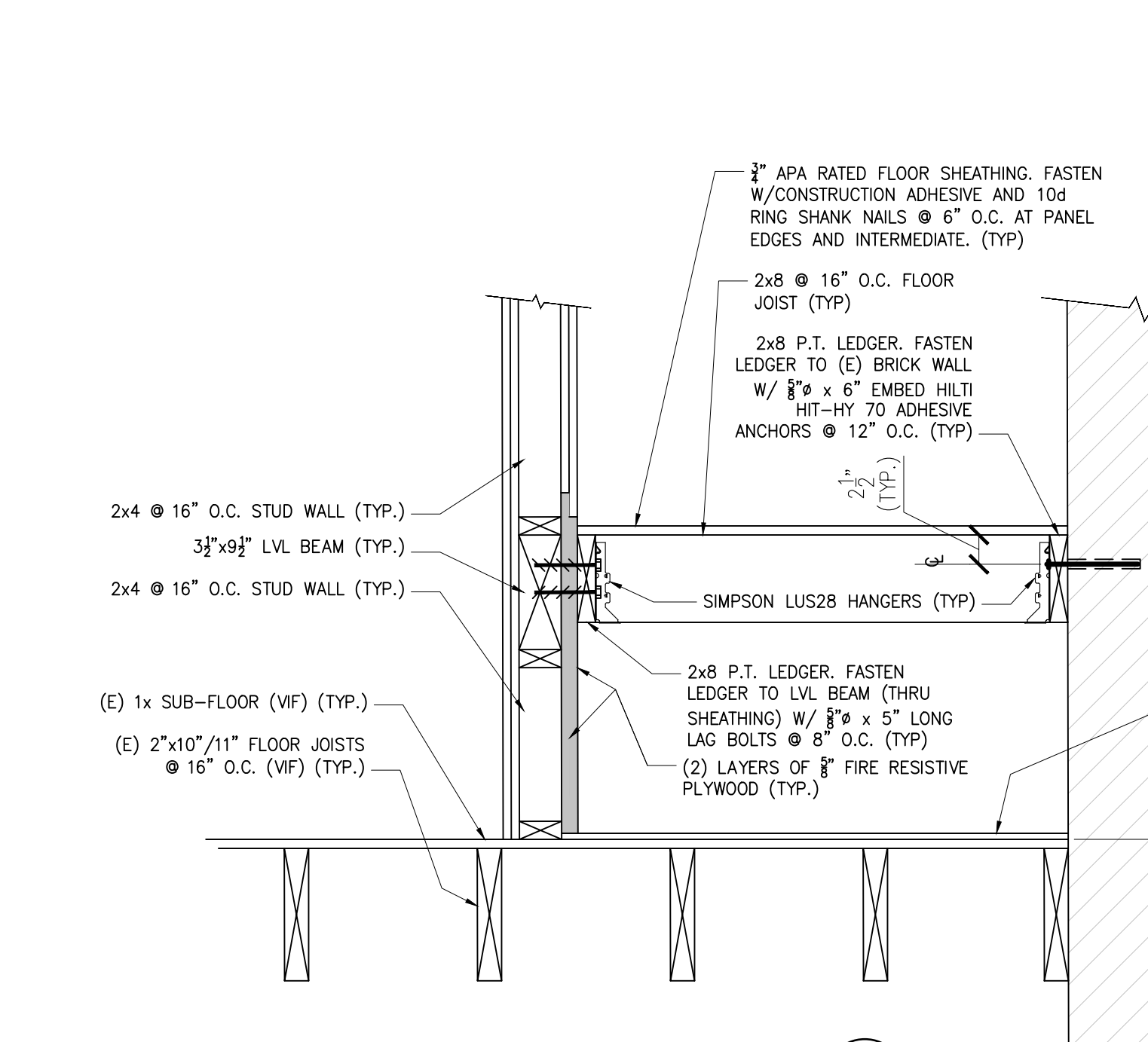
SECTION 3 1" = 1'-0"
