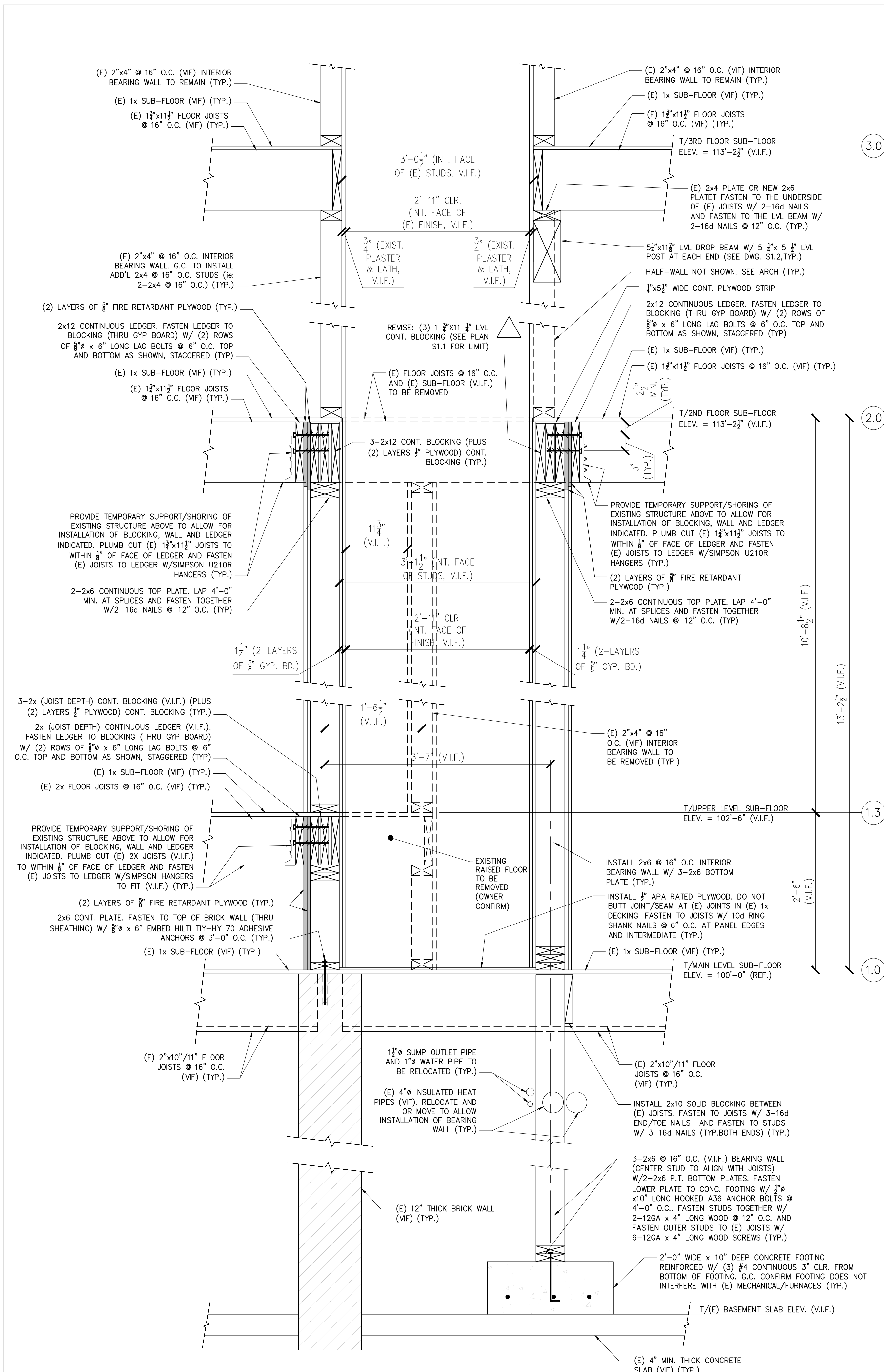
SECTION 1 1" = 1'-0"
