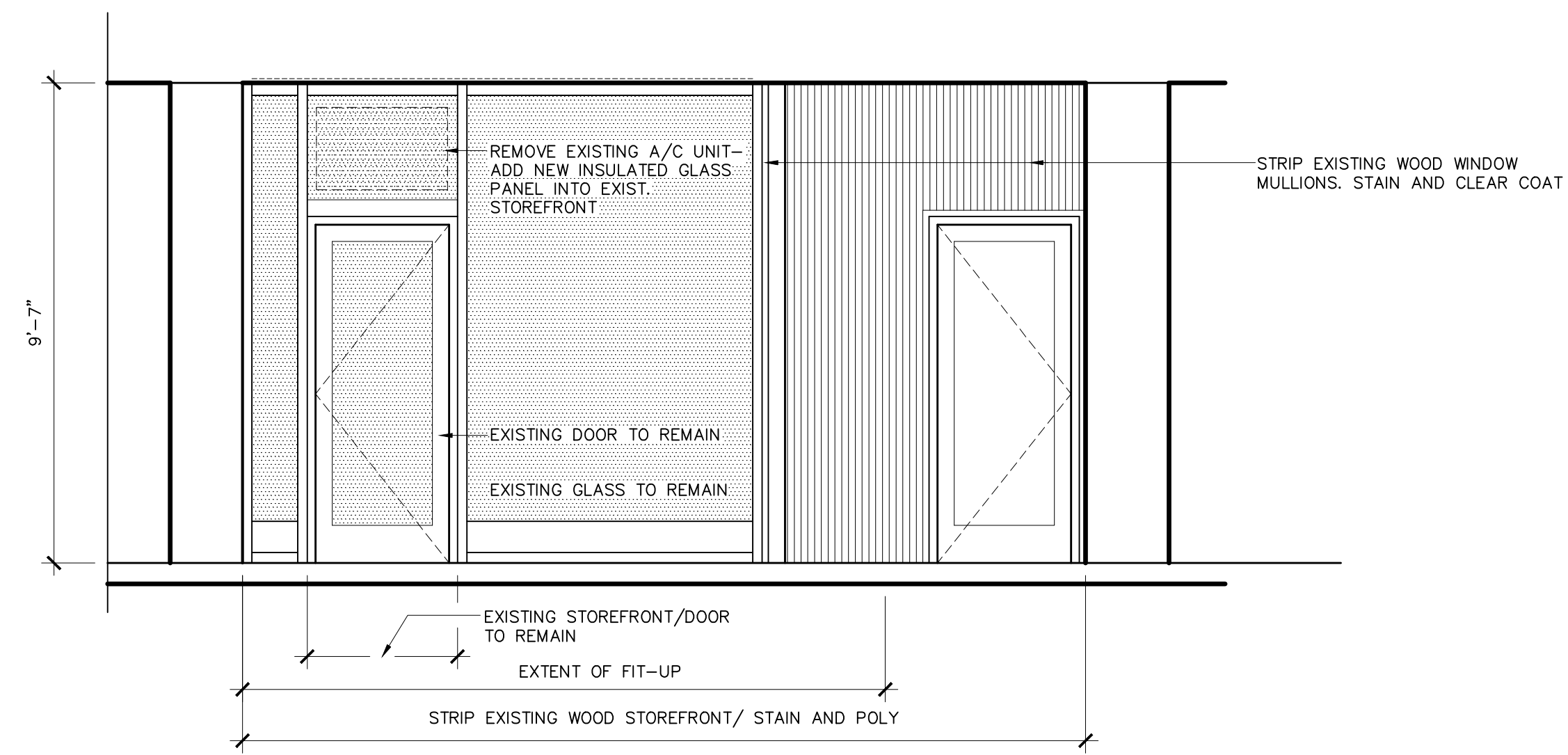
1 SIDEWALK VIEW OF ENTRANCE STOREFRONT SCALE: 3/8" = 1'-0" = 1'-0"
