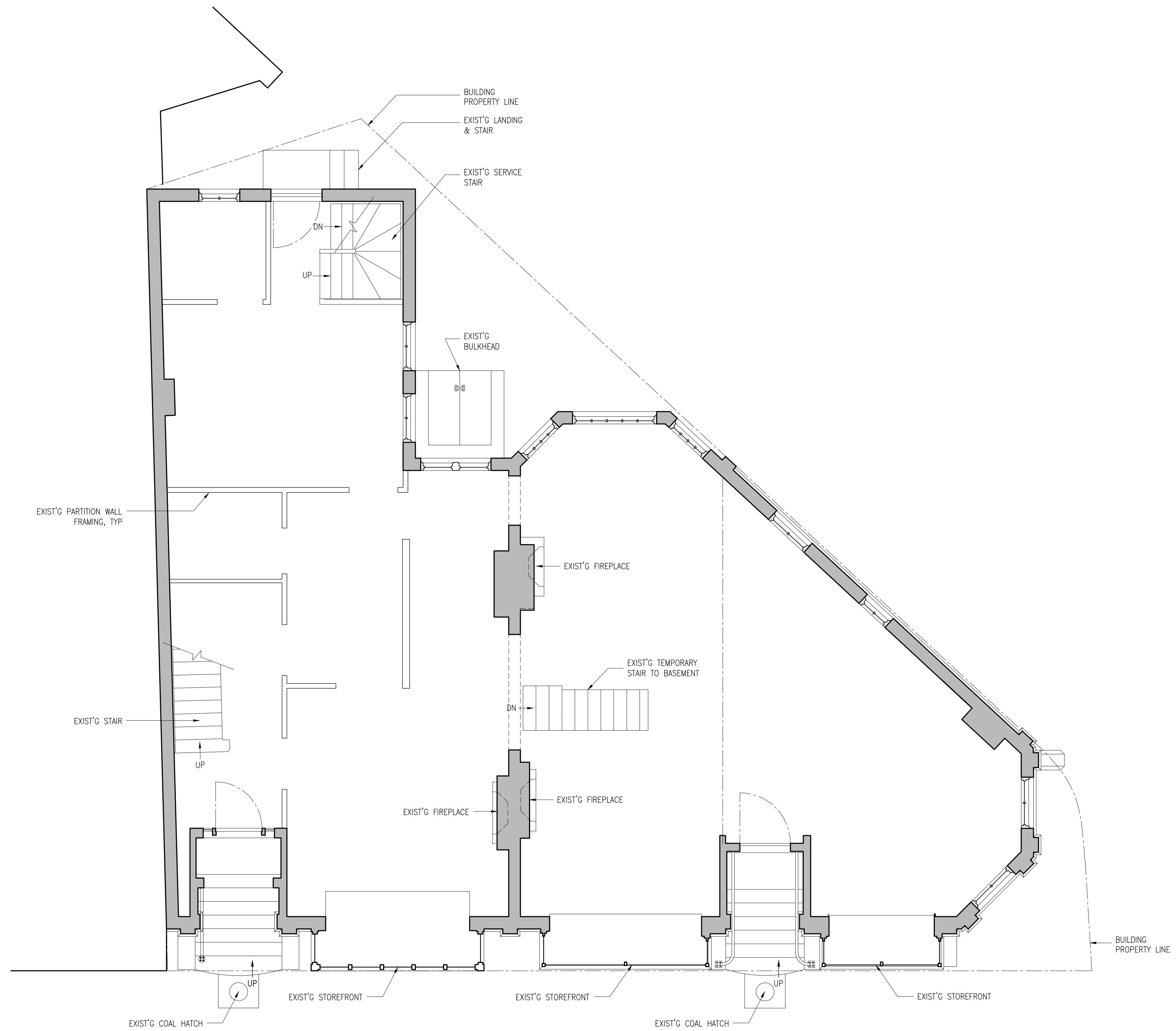
1 1ST FLOOR EXISTING PLAN A-051 1/4" = 1'-0"
