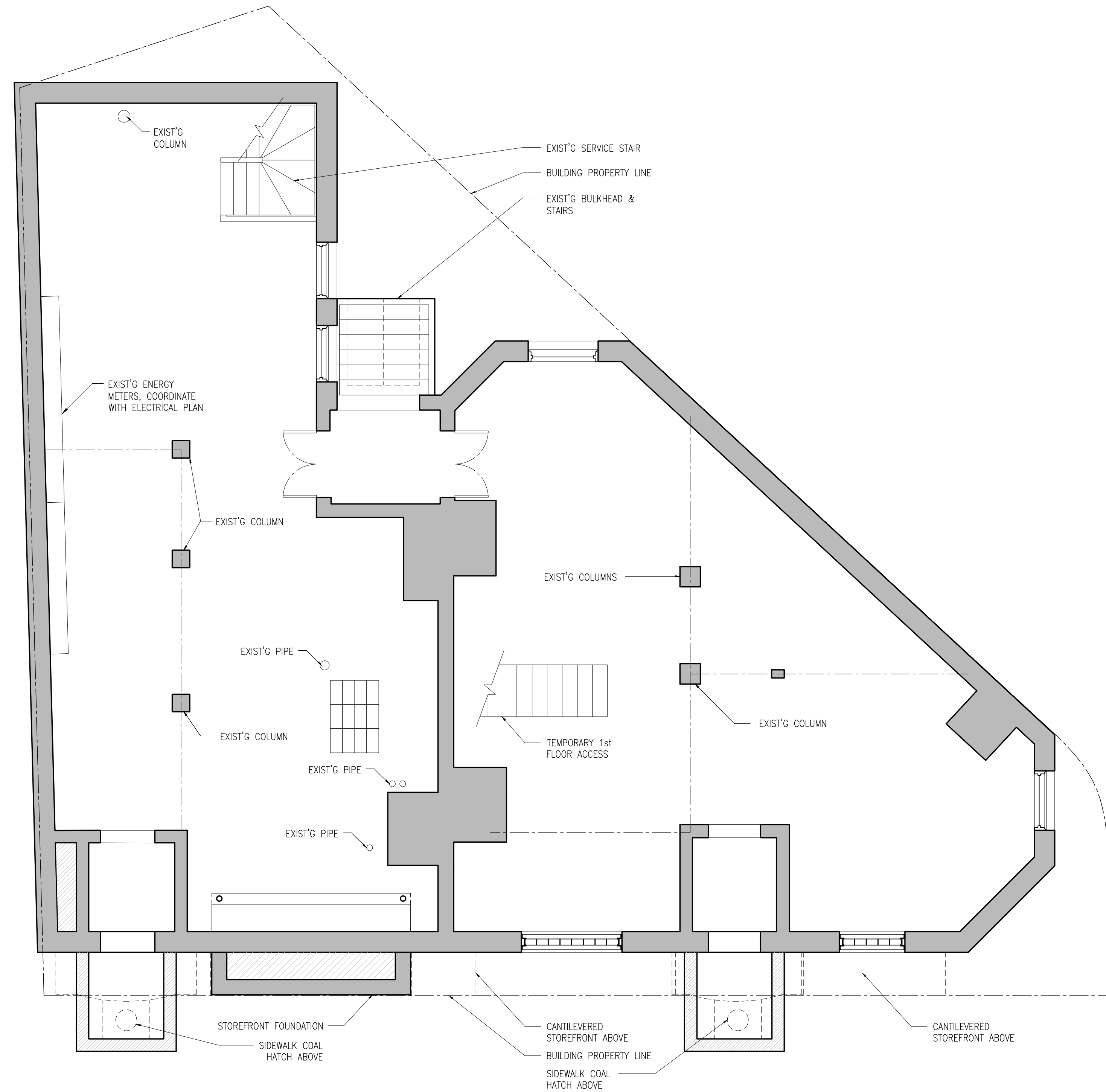
1 BASEMENT EXISTING PLAN A-050 1/4" = 1'-0"
