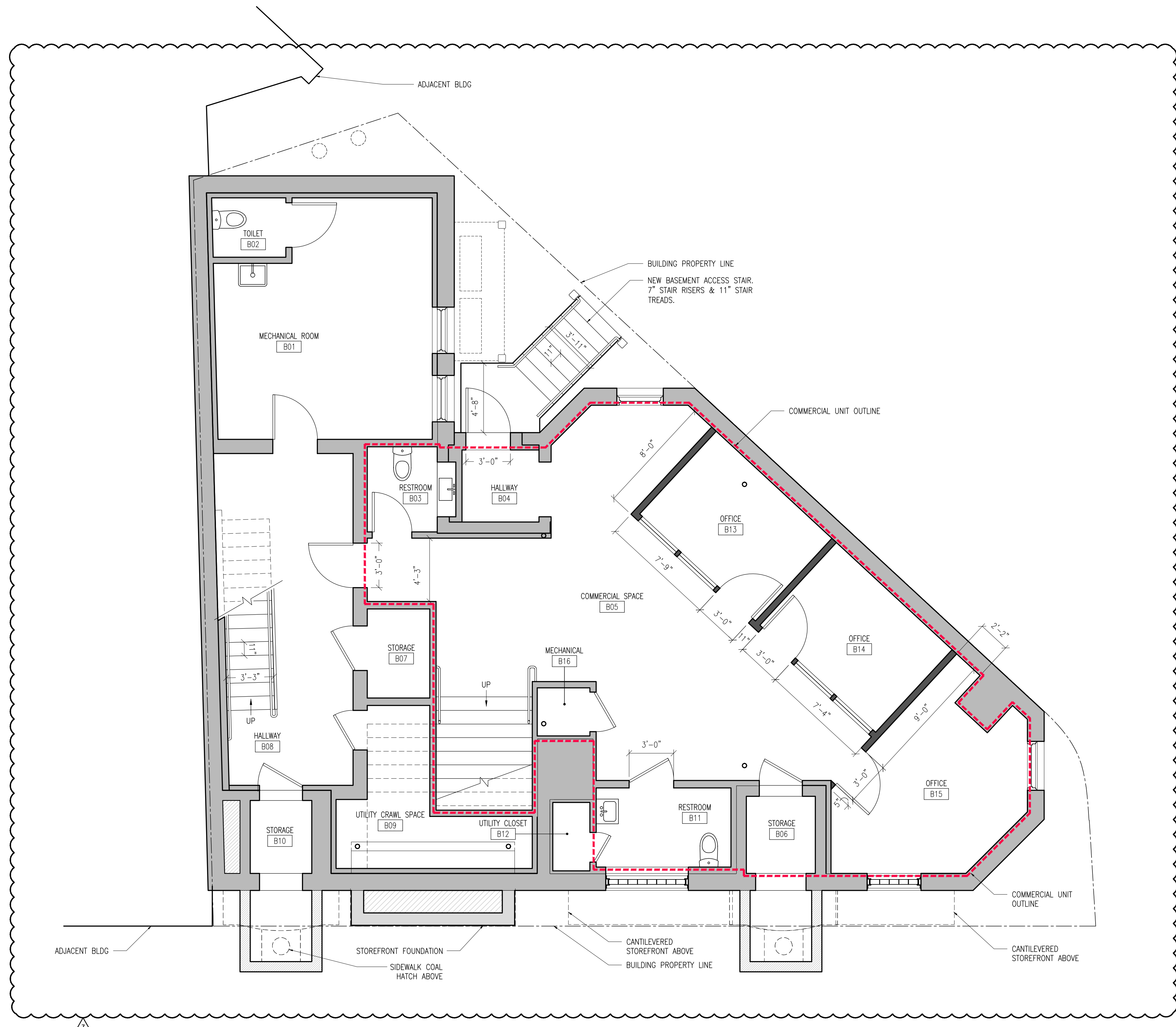
1 A-100 BASEMENT PLAN 1/4" = 1'-0"
