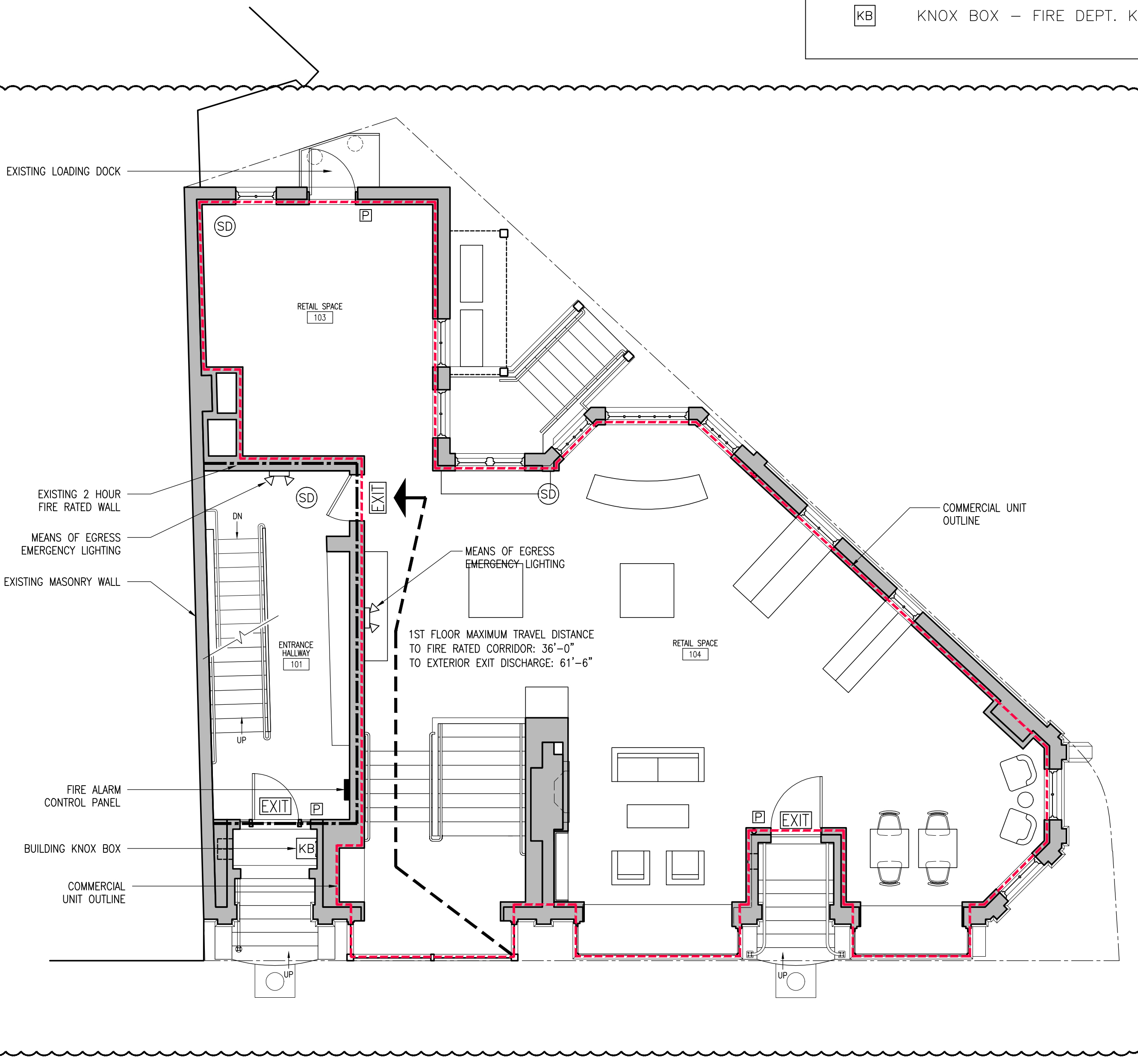
2 1ST FLOOR LIFE SAFETY PLAN A-005 3/16" = 1'-0"
