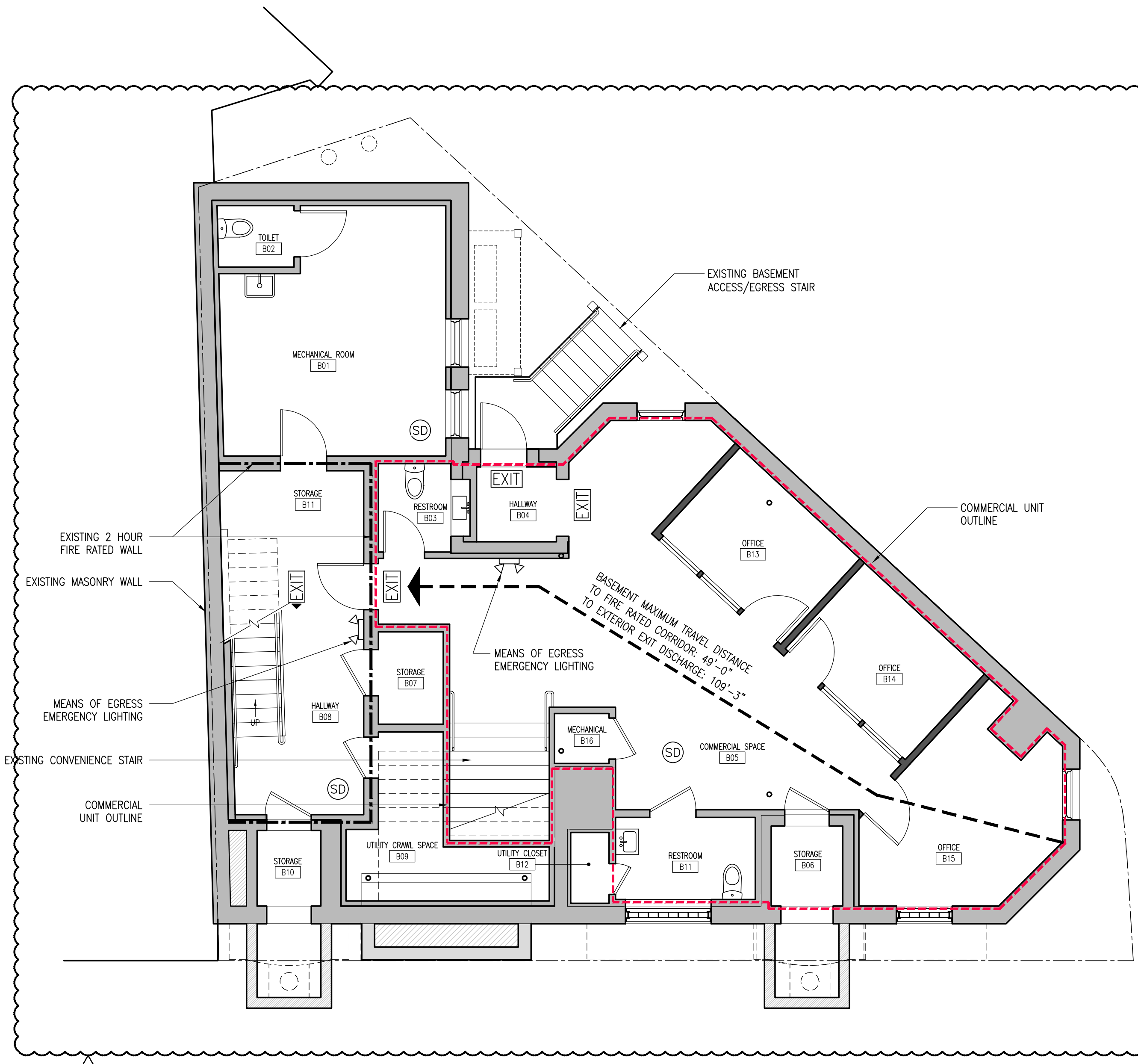
1 BASEMENT LIFE SAFETY PLAN A-005 3/16" = 1'-0"
