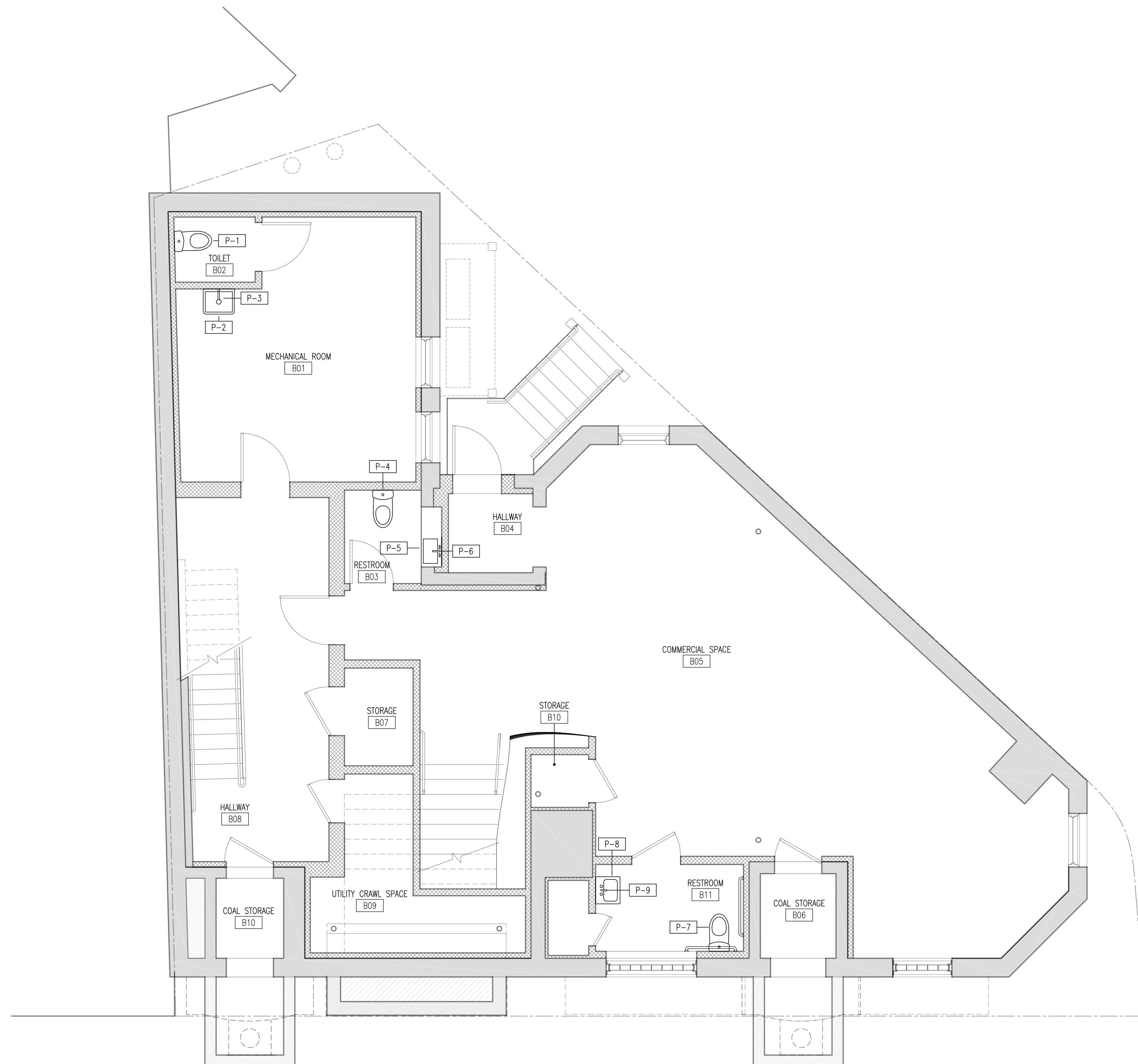
1 BASEMENT PLUMBING & FIXTURE PLAN P-100 1/4" = 1'-0"
