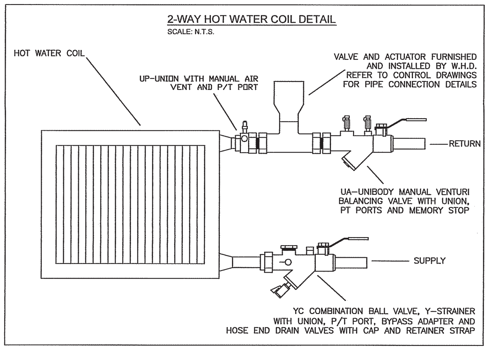
2-WAY HOT WATER COIL DETAIL SCALE: NTS
