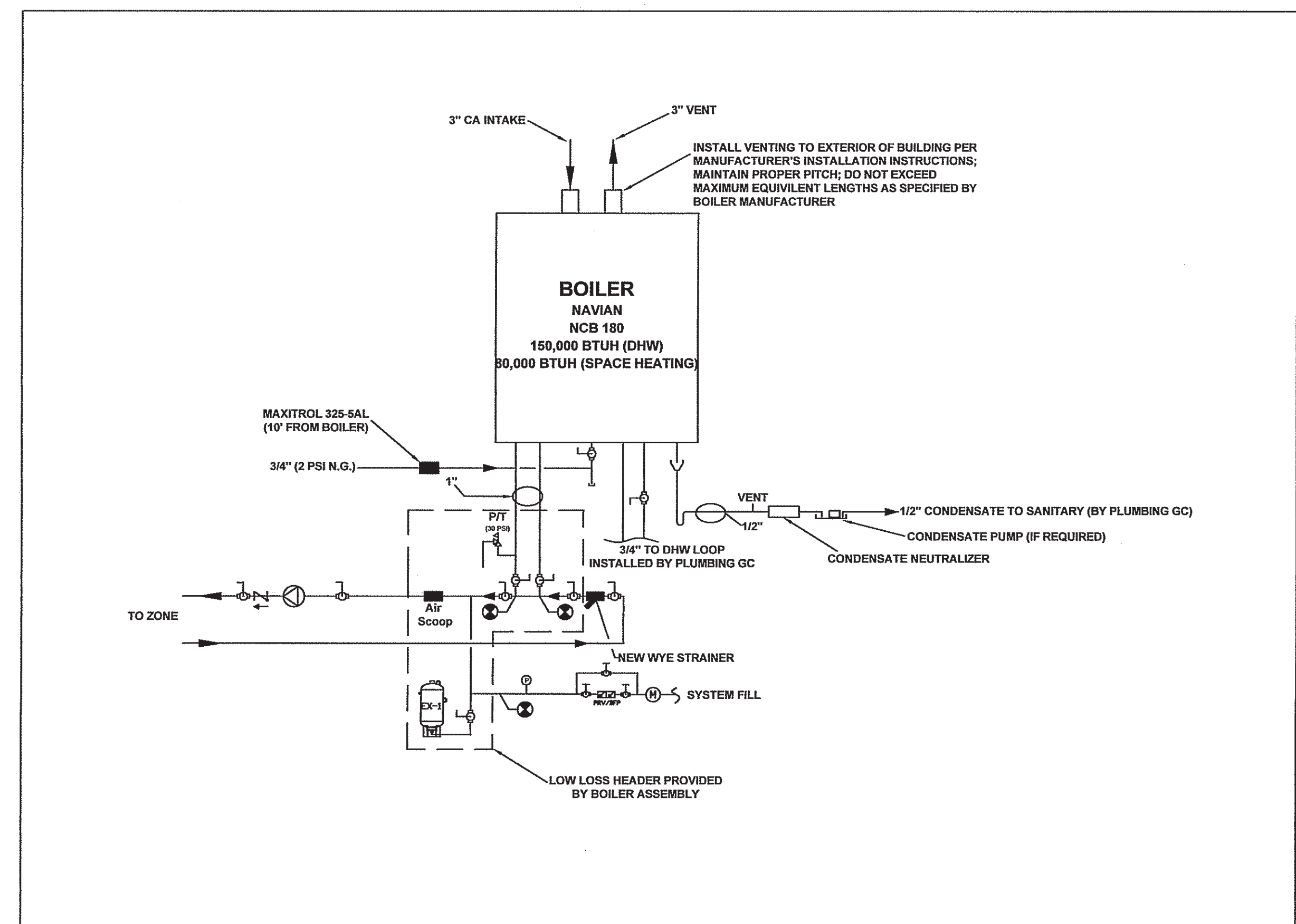
BOILER DETAIL SCALE: NTS
