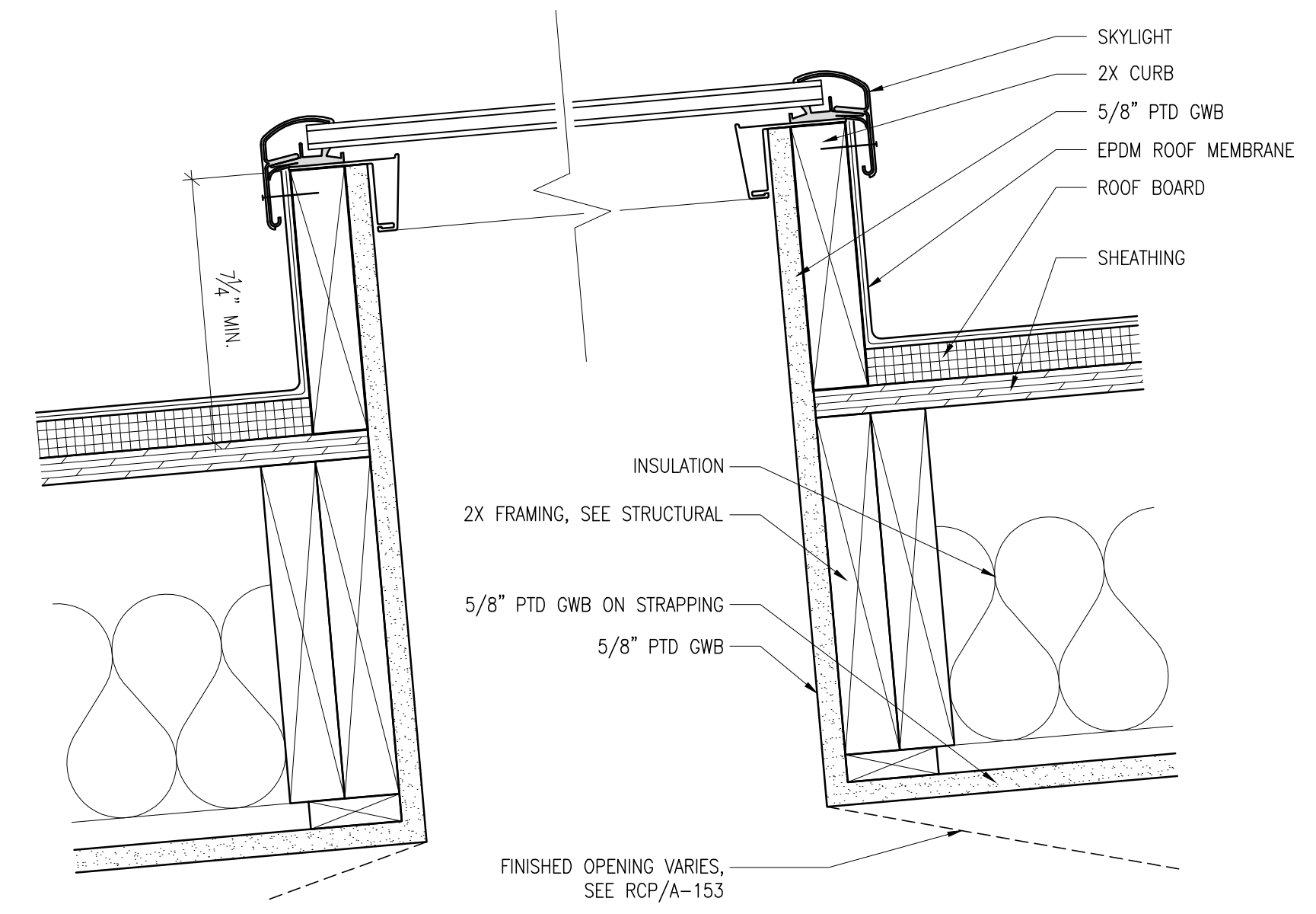
2 FIXED SKYLIGHT VERTICAL CROSS SECTION 3" = 1'-0"
