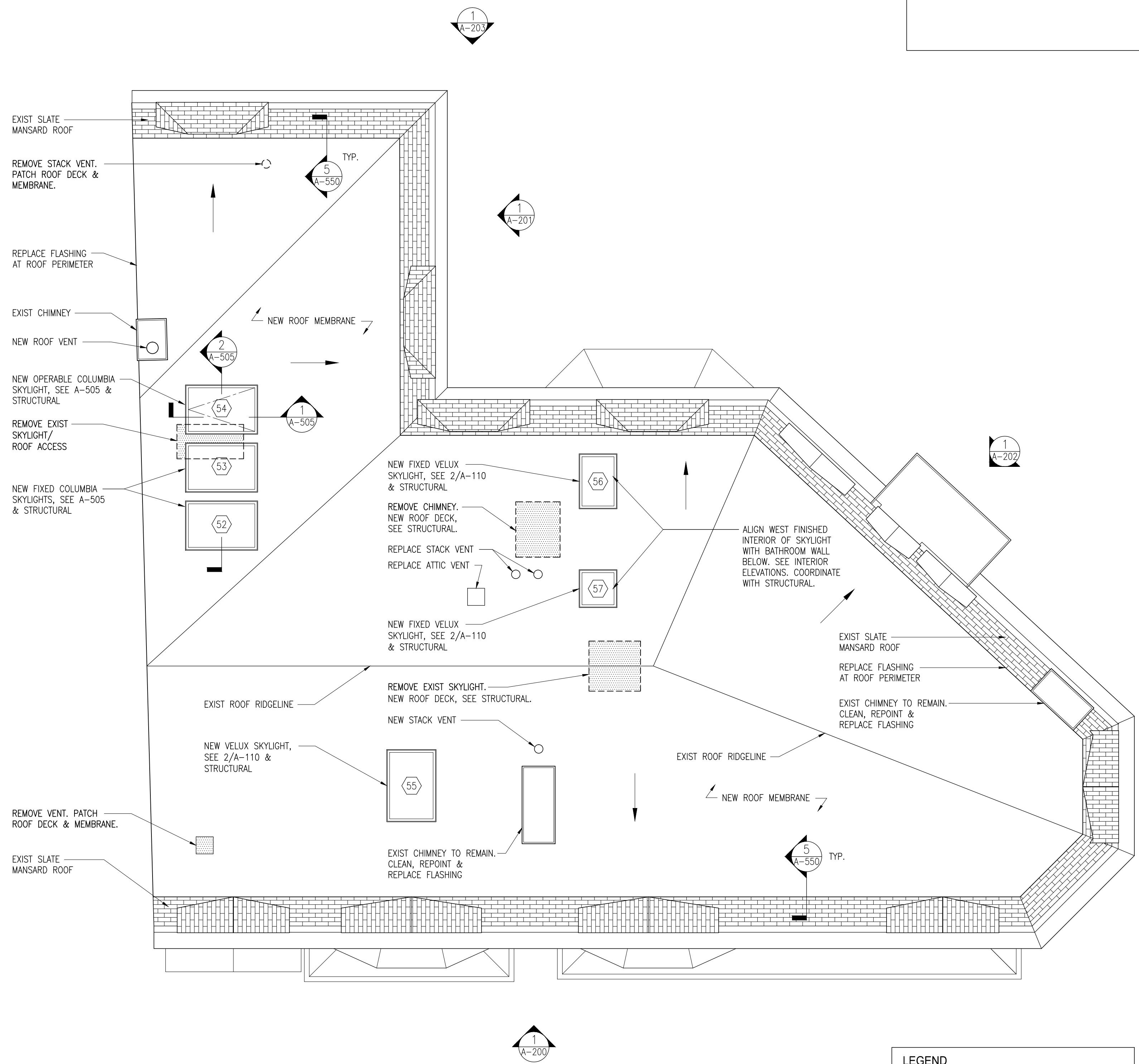
1 ROOF PLAN 1/4" = 1'-0"
