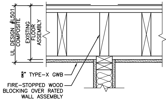
CEILING TYPE 1
