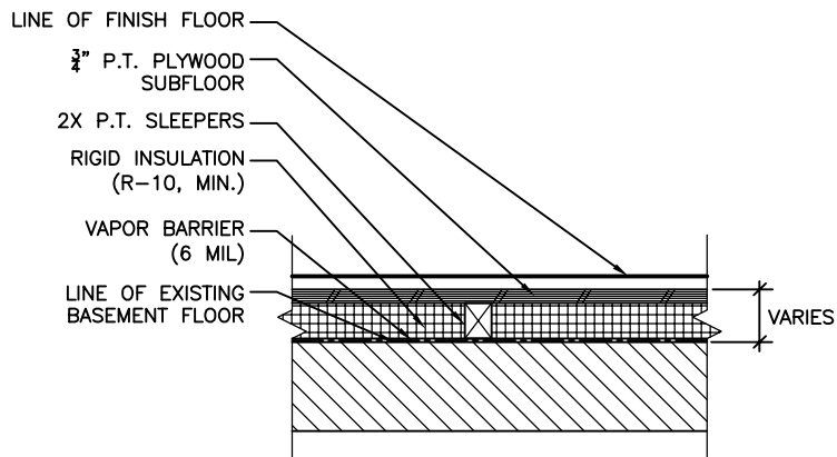
FLOOR TYPE 1
