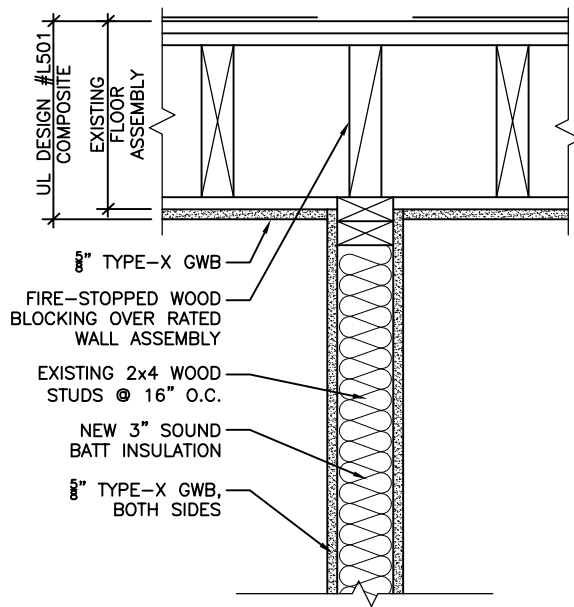
WALL TYPE 2
