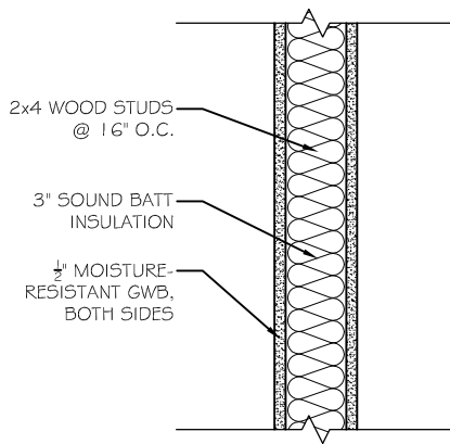
WALL TYPE 1
