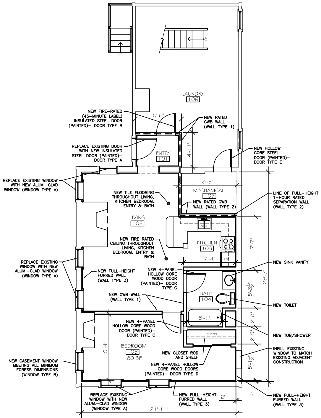
1. FLOOR PLAN
