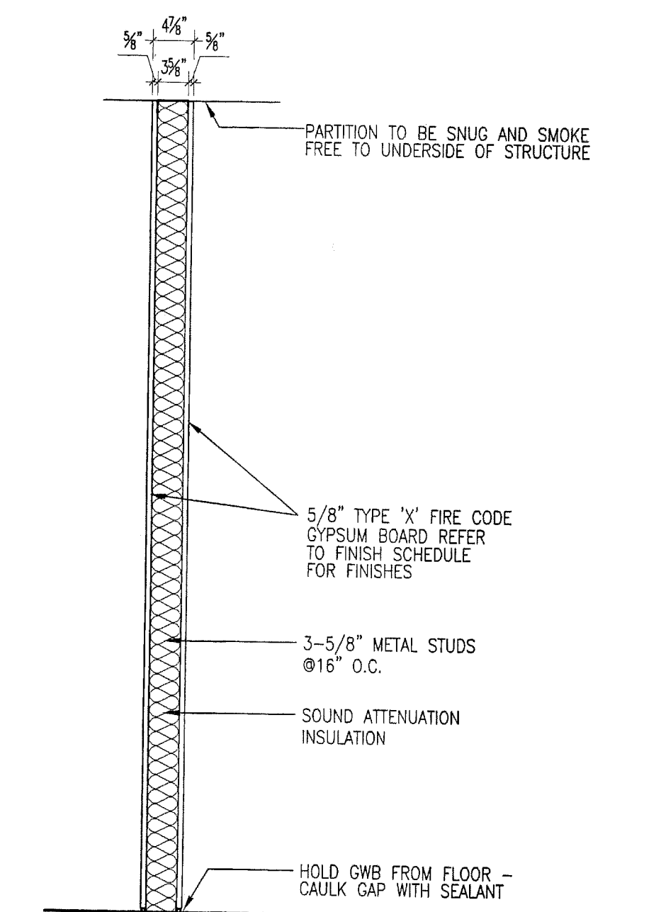
W 6 WALL DETAIL (NON RATED) SCALE 3/4"=1'-0"
