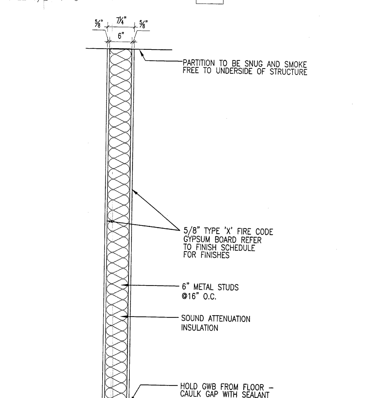
W 7 WALL DETAIL (NON RATED) SCALE 3/4"=1'-0"
