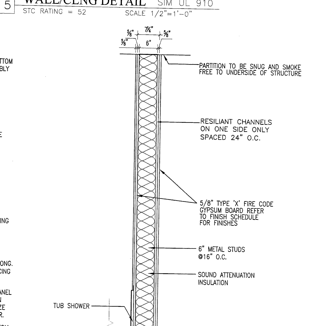
W10 WALL DETAIL (1 HR RATED) U.L. DES. U419 STC: 56 SCALE 3/4"=1'-0"
