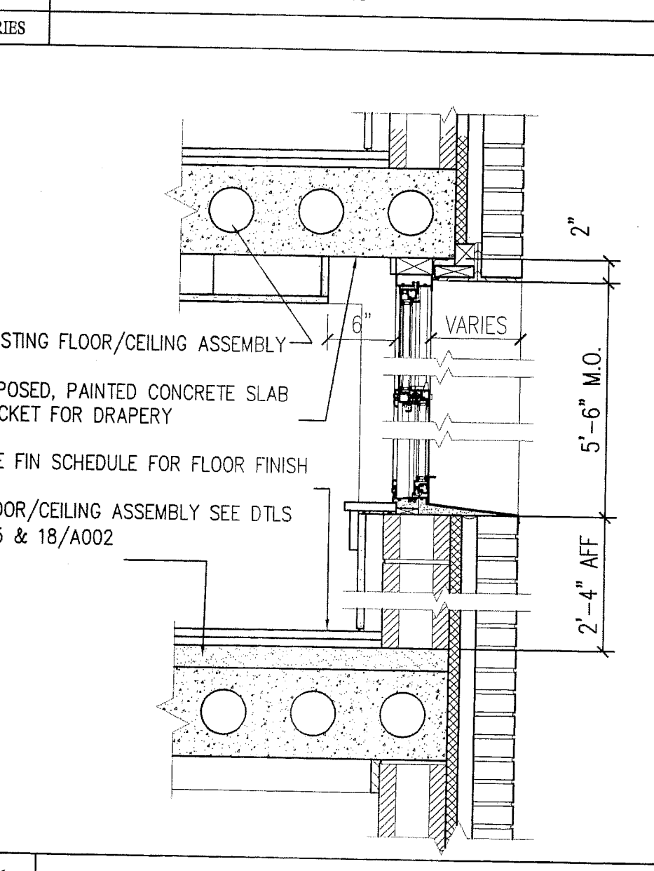
A1 HEAD AND JAMB DETAILS 3/4"=1'-0"
