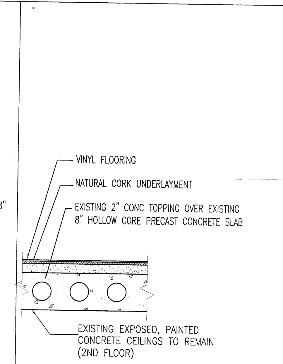
A18 FLOOR/CLNG ASSEMBLY 1/2"=1'-0" IIC RATING +41-58 DB 3 HR RATED PER ICC PFC-4833
