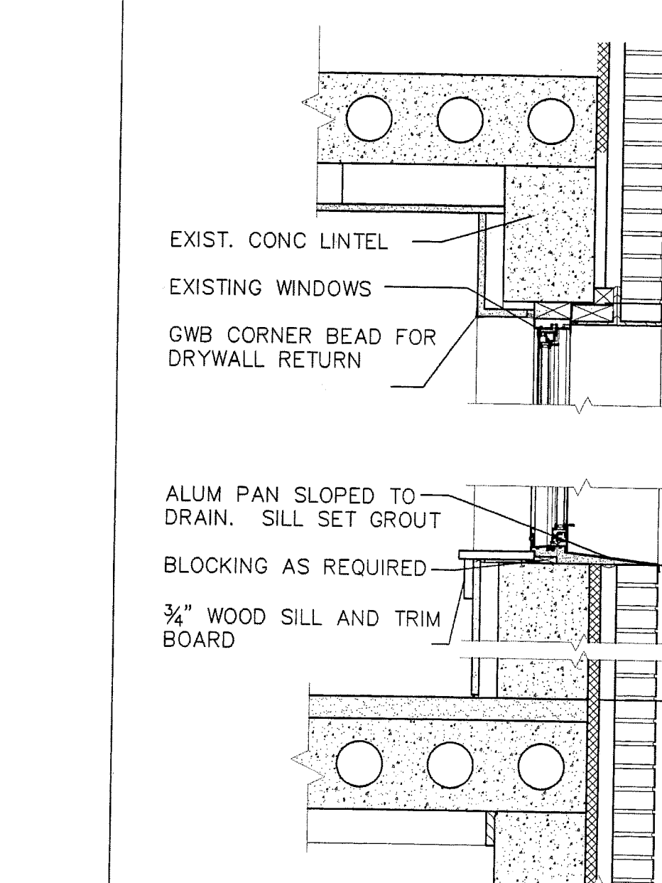
A9 HEAD AND JAMB DETAILS 3/4"=1'-0"
