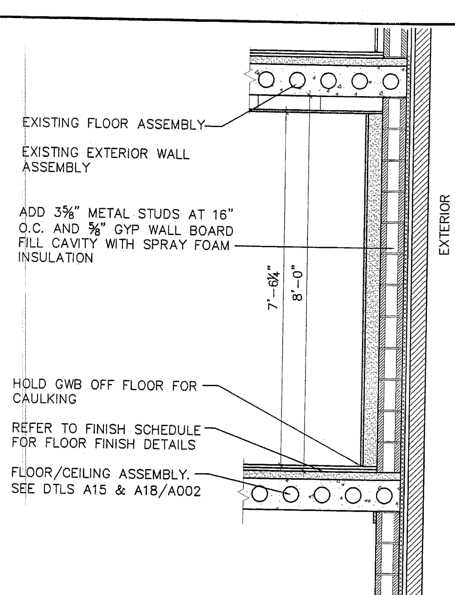
W 2 WALL DETAIL (NON RATED) SCALE 1/2"=1'-0"
