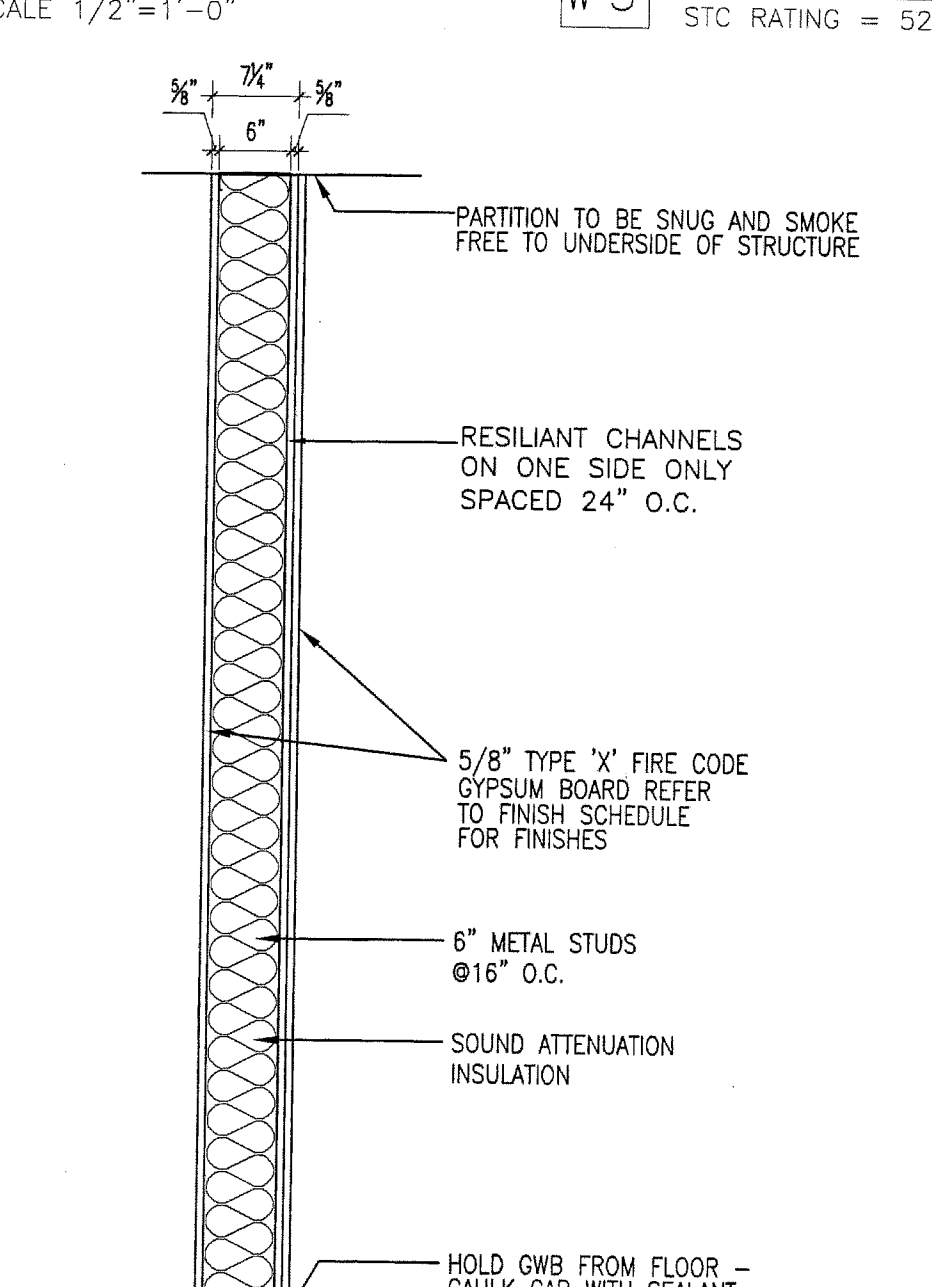
W 8 WALL DETAIL (1 HR RATED) U.L. DES. U419 STC: 56 SCALE 3/4"=1'-0"
