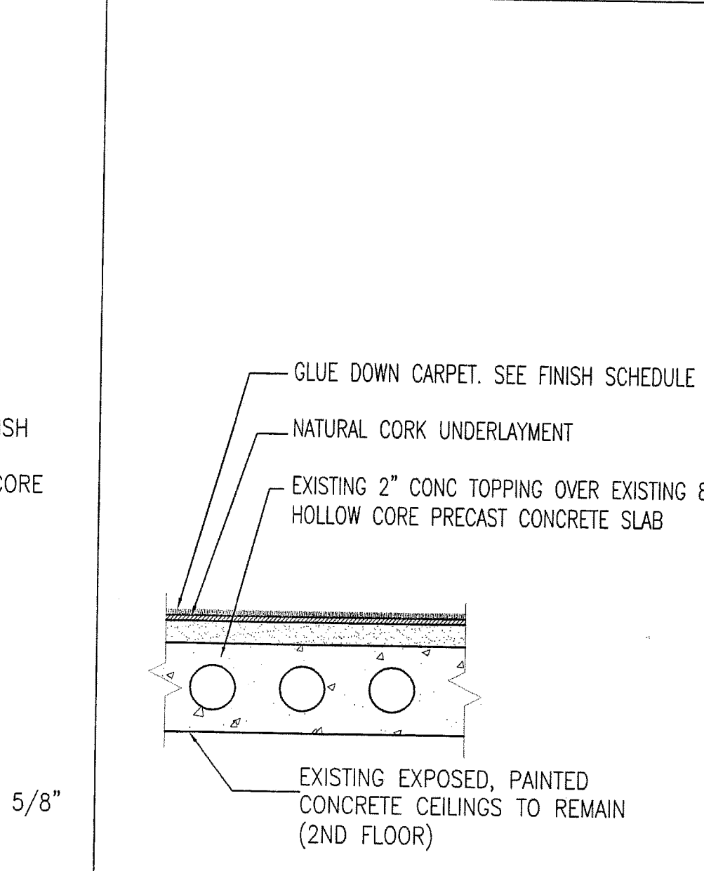
A15 FLOOR/CLNG ASSEMBLY 1/2"=1'-0" IIC RATED +41-76 DB 3 HR RATED PER ICC PFC-4833
