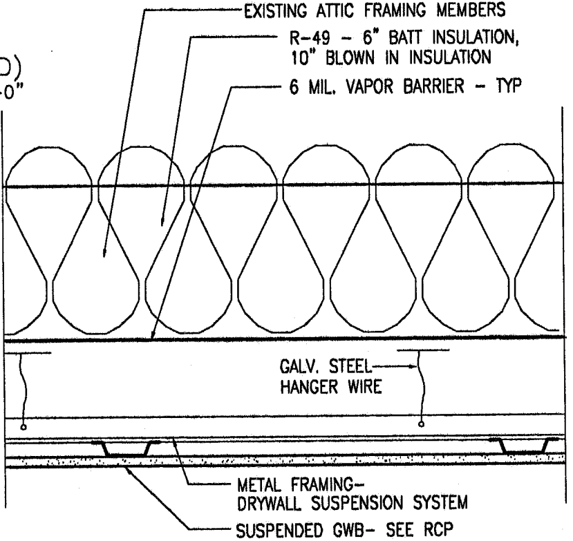
C3 CEILING ASSEMBLY- THIRD FLOOR
