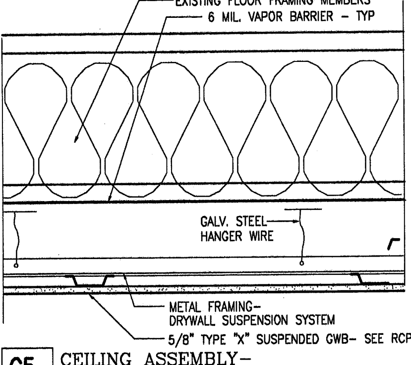
C5 CEILING ASSEMBLY- 1 HOUR RATED C5A CEILING ASSEMBLY- NOT RATED
