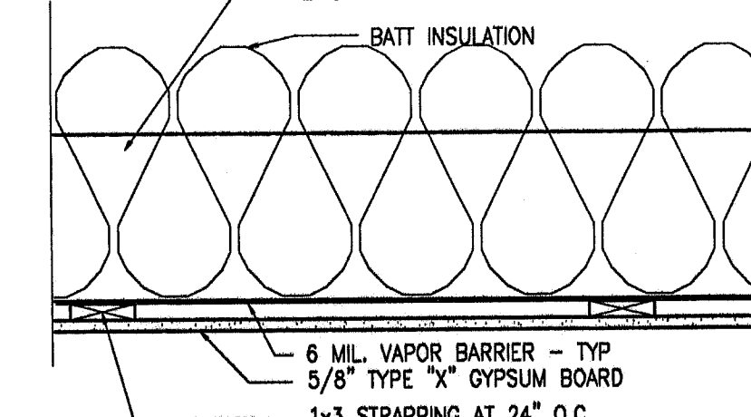
C8 CEILING ASSEMBLY-BASEMENT MECH. & STORAGE ROOMS 1 HOUR RATED-
