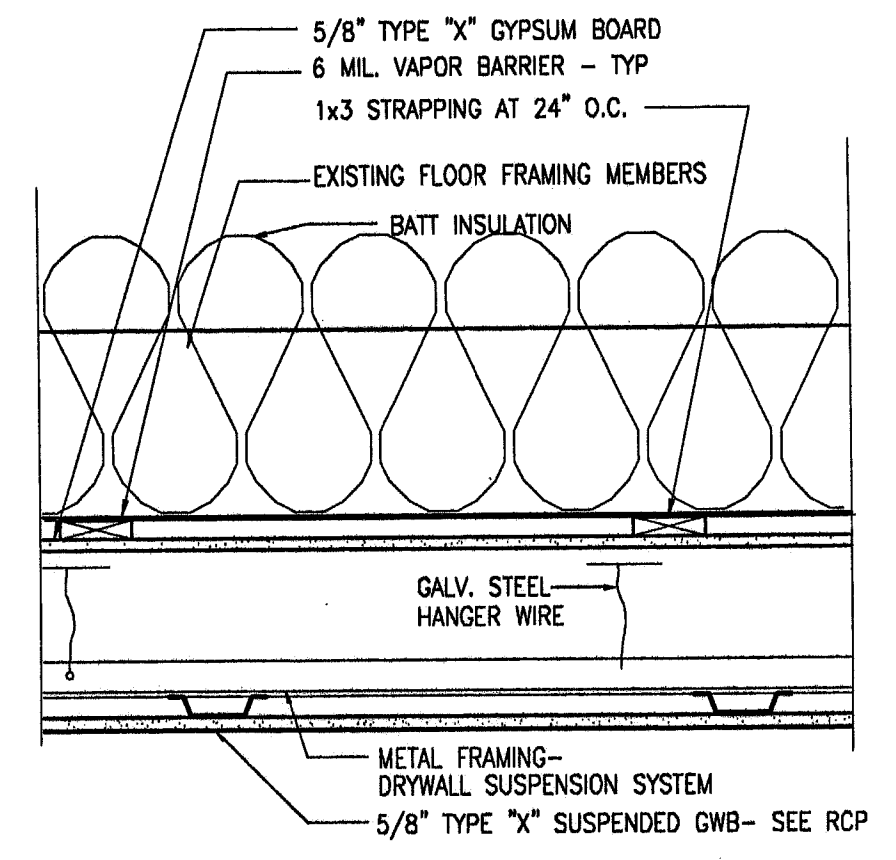
C1 CEILING ASSEMBLY- 1 HR RATED WITH ACT CEILING 1 HOUR RATED-
