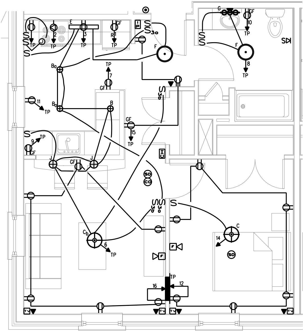
UNIT 201 1B-5 SCALE: 1/4" = 1'-0" UNIT 301 SIMILAR
