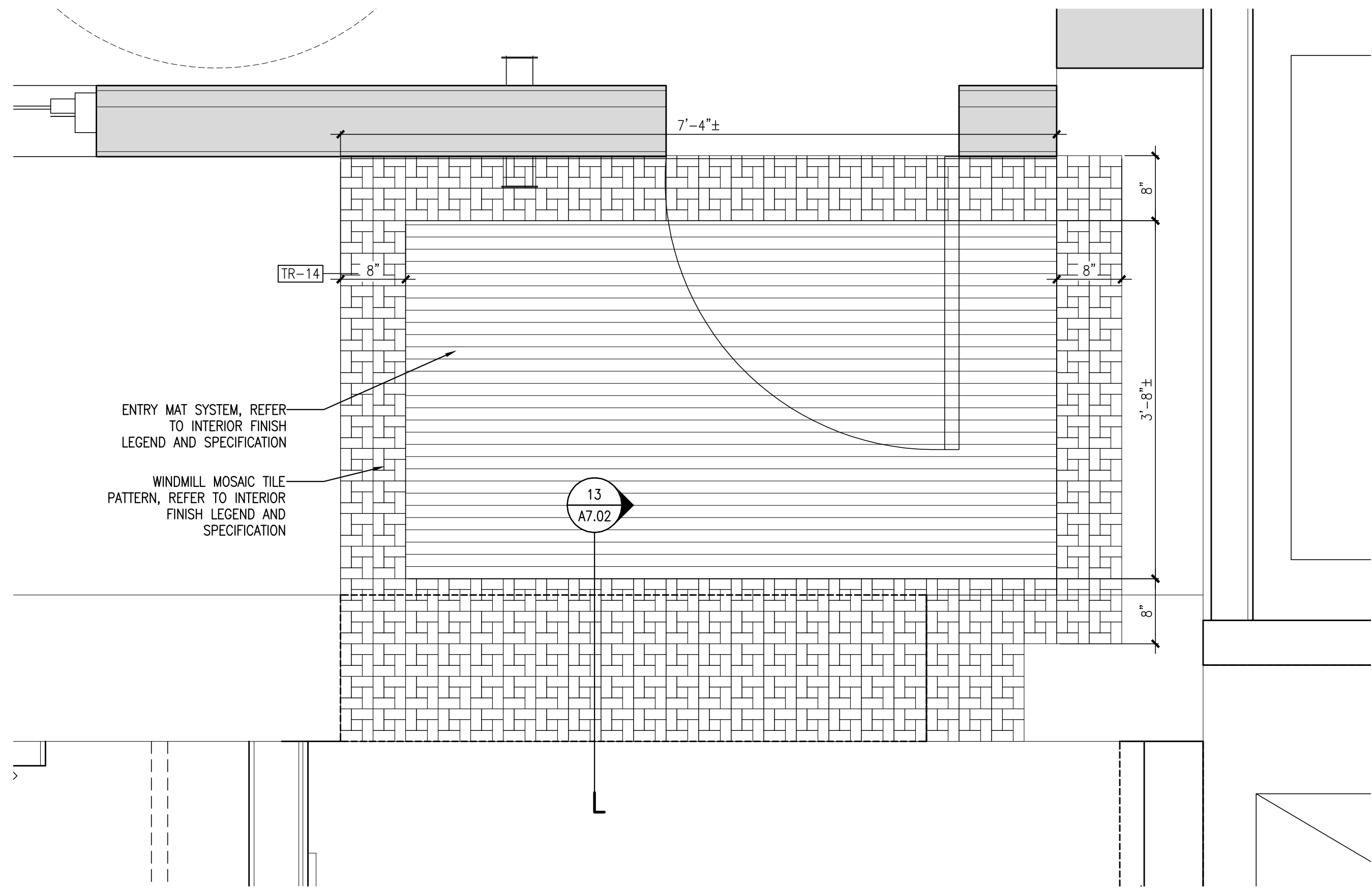
3 CORRIDOR 126 FLOOR PATTERN PLAN REFERENCED FROM: SCALE: 1" = 1'-0"
