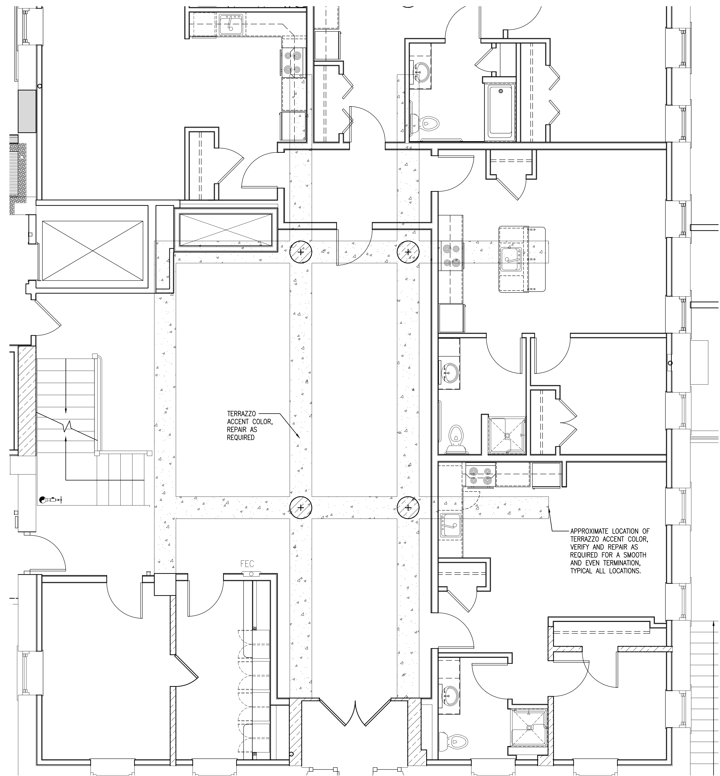
2 EXTENT OF EXISTING ACCENT TERRAZZO REFERENCED FROM: SCALE: 1/4" = 1'-0"
