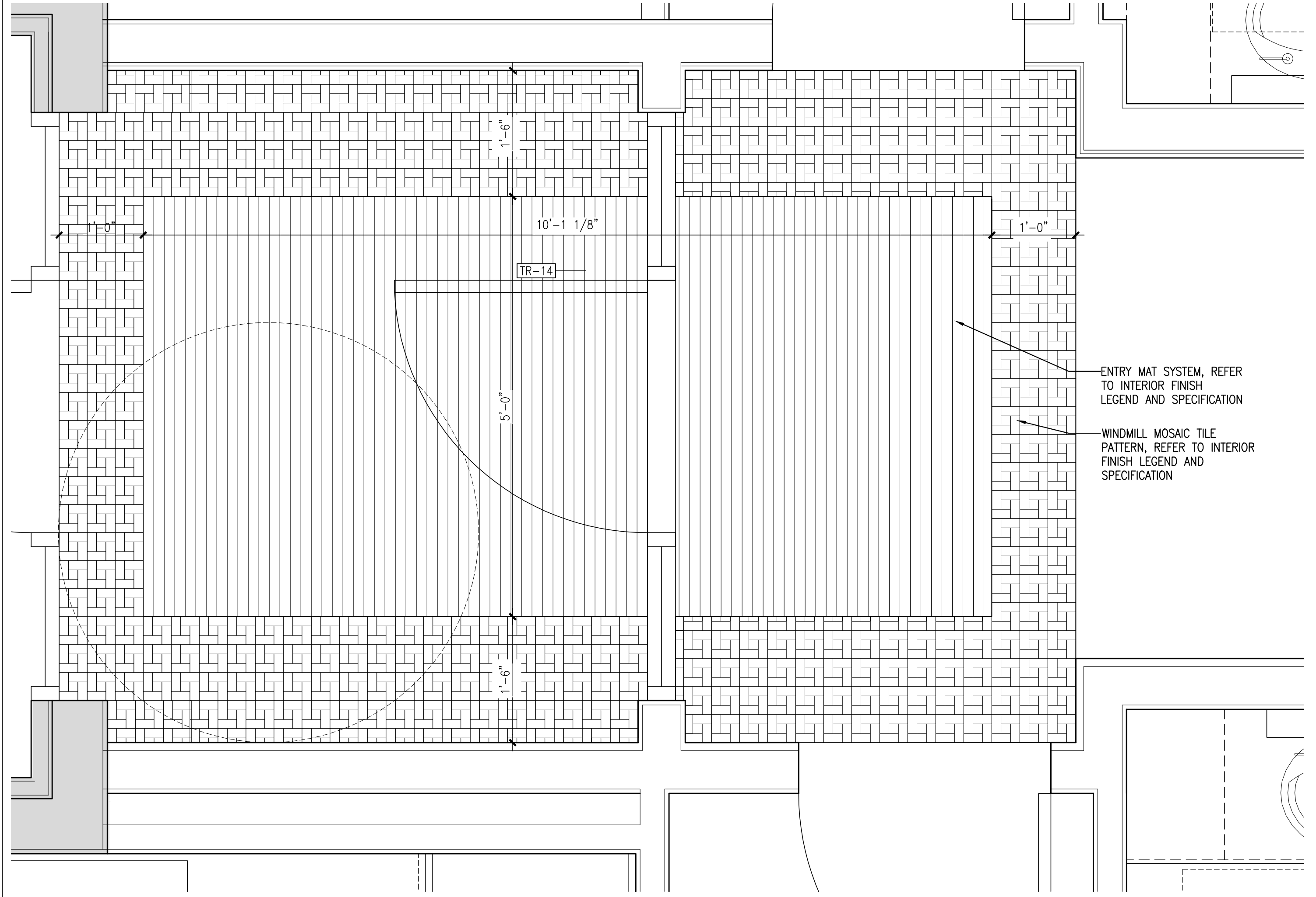
1 VESTIBULE 122 FLOOR PATTERN PLAN REFERENCED FROM: SCALE: 1" = 1'-0"
