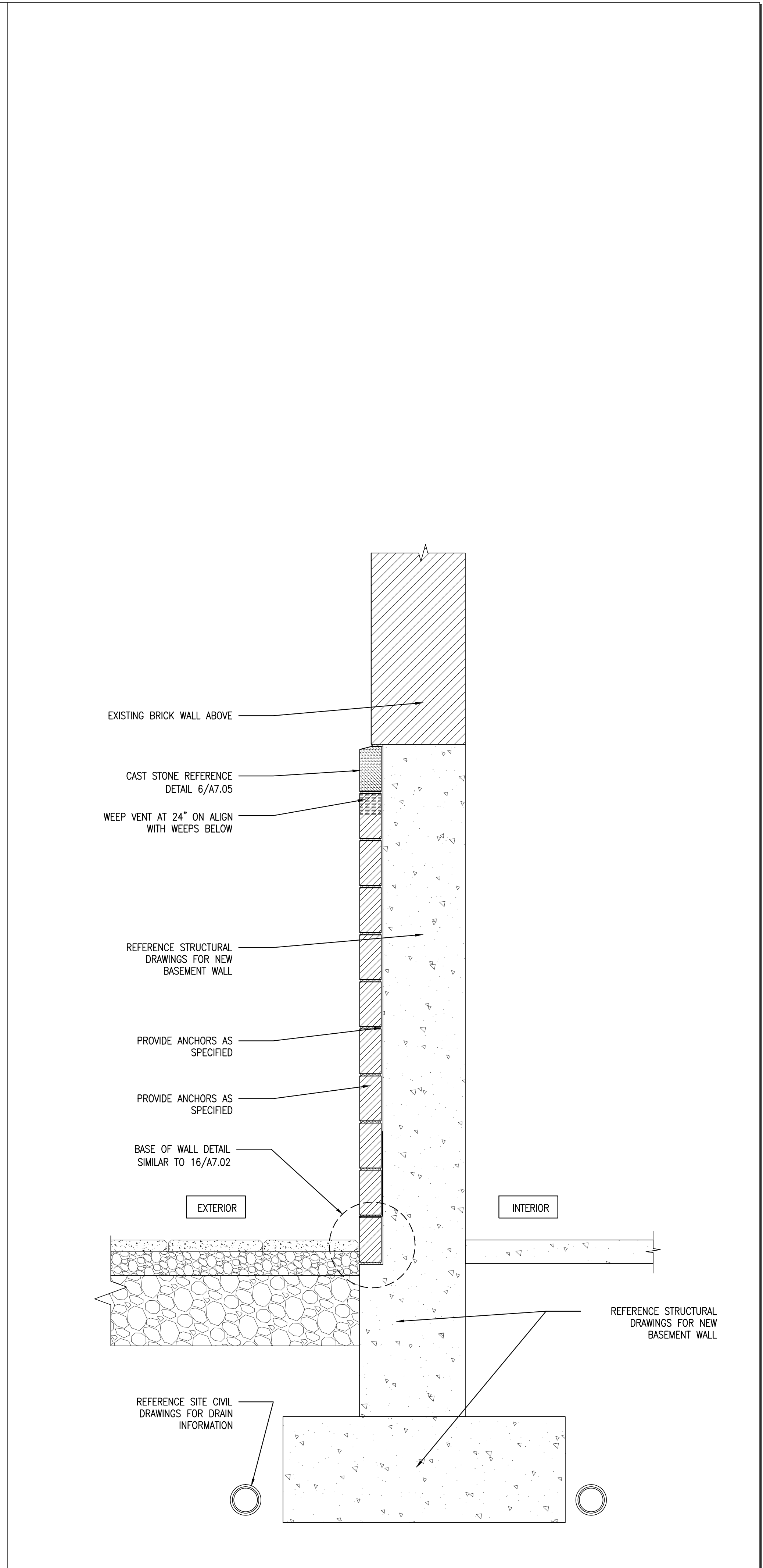
6 NEW BASEMENT WALL AT SOUTH SIDE REFERENCED FROM: SCALE:
