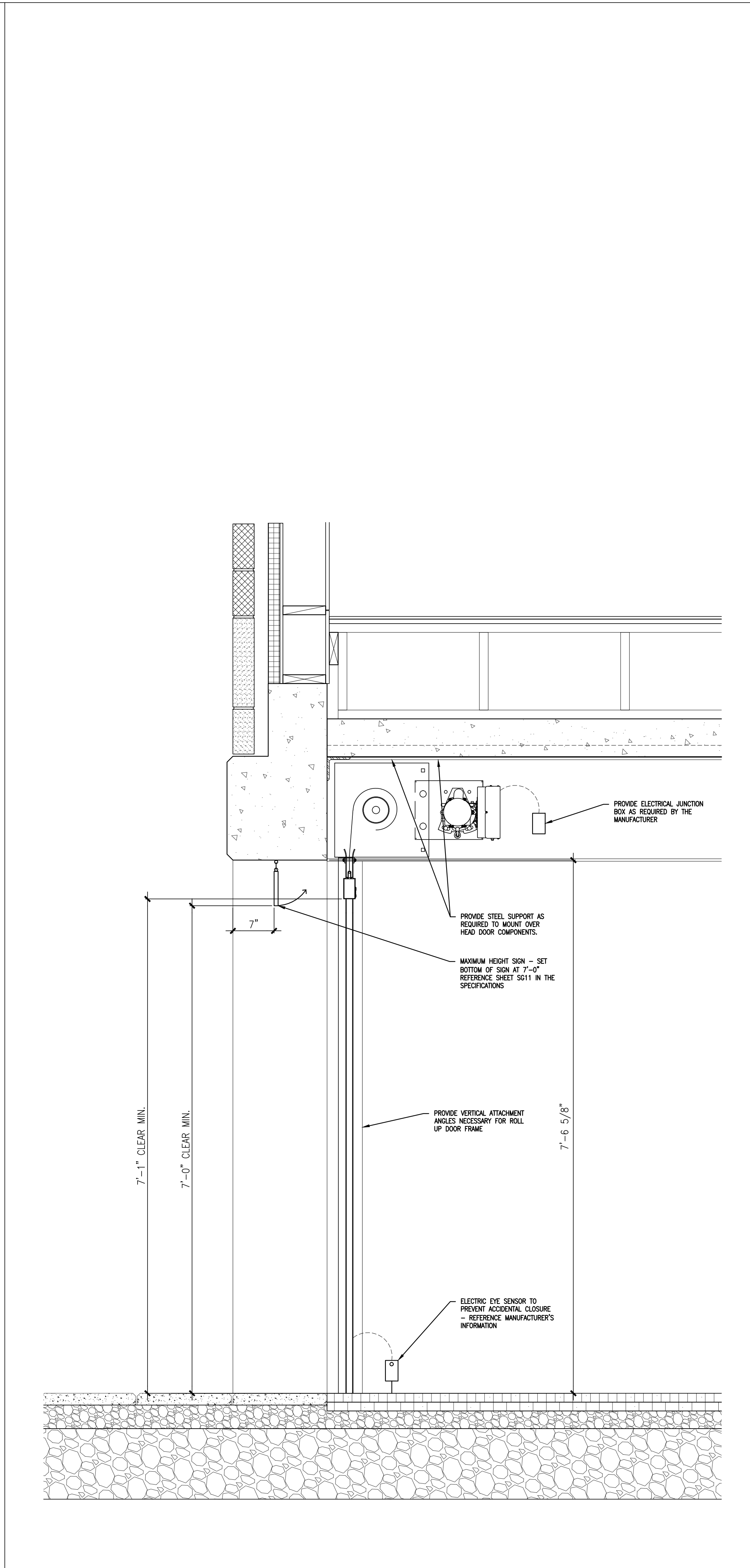
5 GARAGE ROLL UP DOOR REFERENCED FROM: SCALE:
