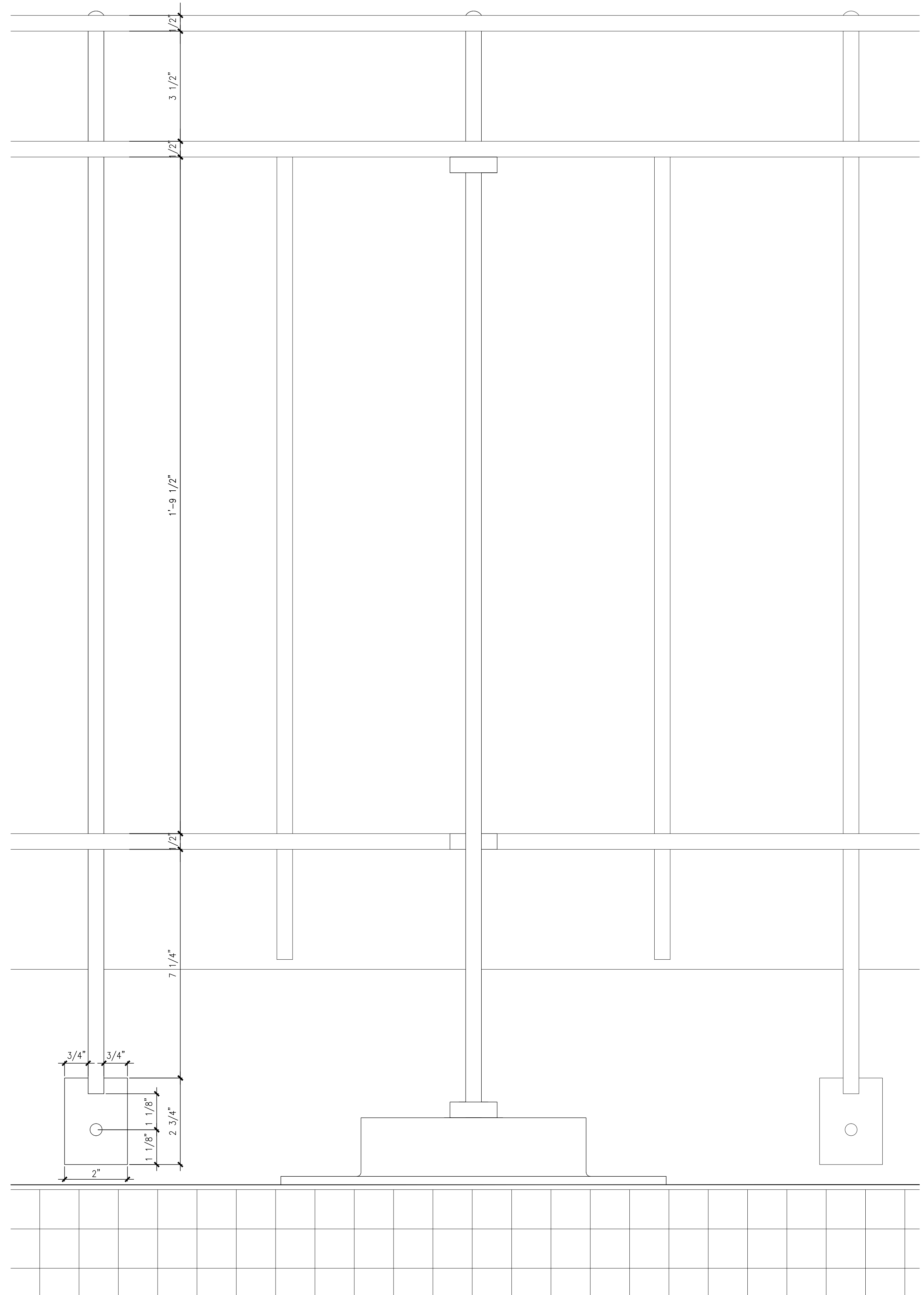
2 DETAIL @ FENCE SUPPORT REFERENCED FROM:
