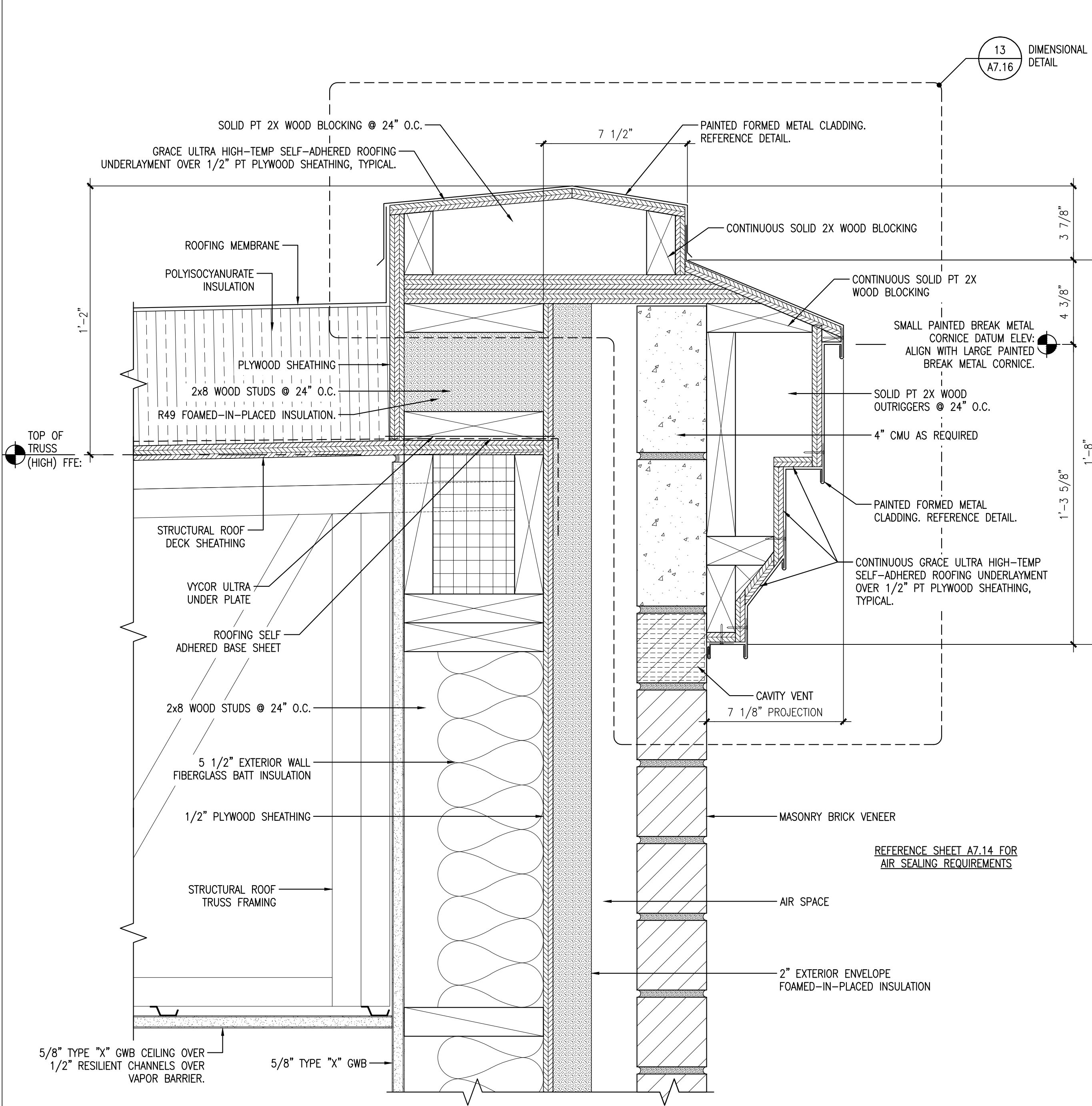
13 TOP OF WALL DETAIL @ SMALL BREAK METAL CORNICE REFERENCED FROM: SCALE: 3" = 1'-0"
