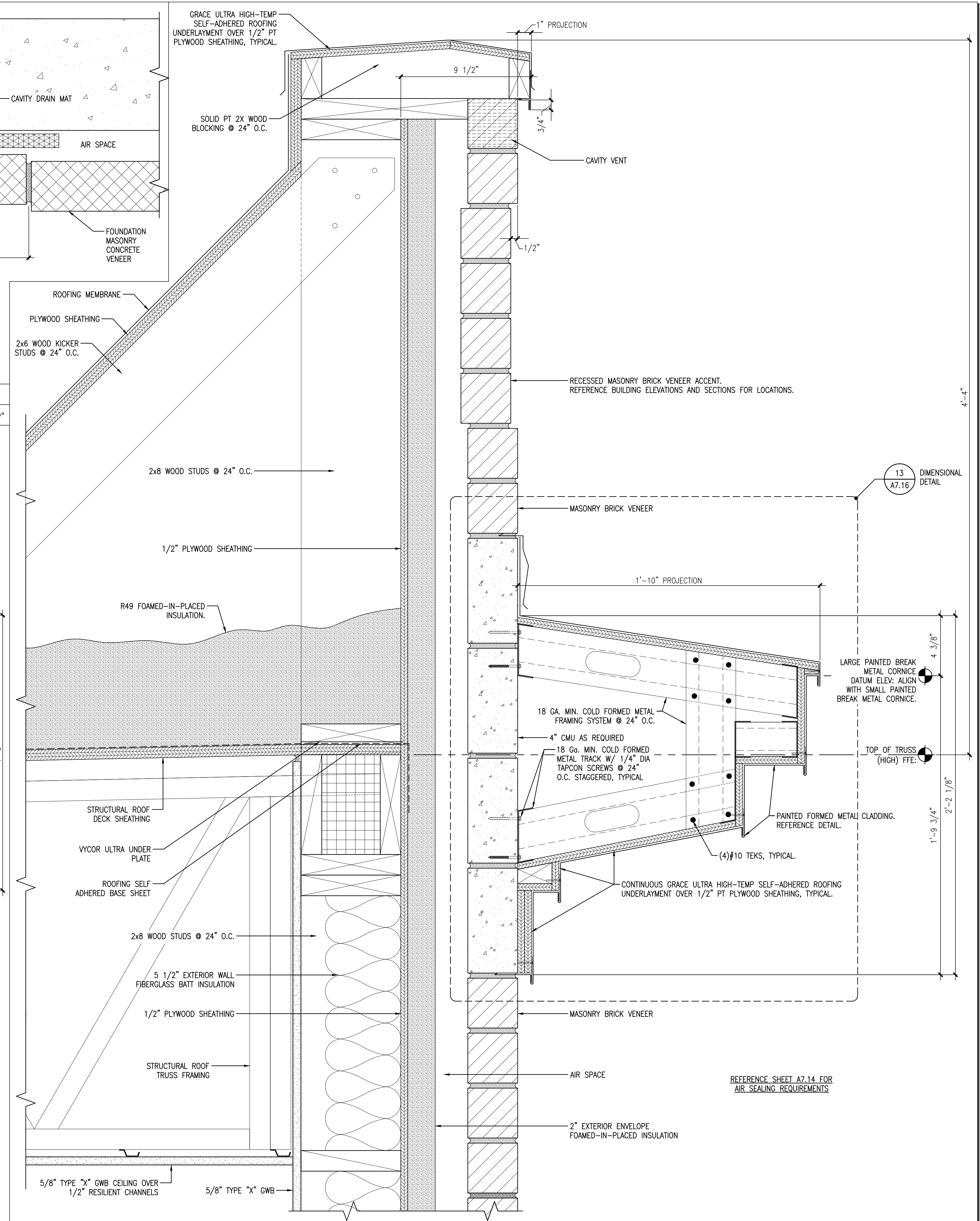
15 TOP OF WALL DETAIL @ LARGE BREAK METAL CORNICE WITH PARAPET WALL REFERENCED FROM: SCALE: 3" = 1'-0"
