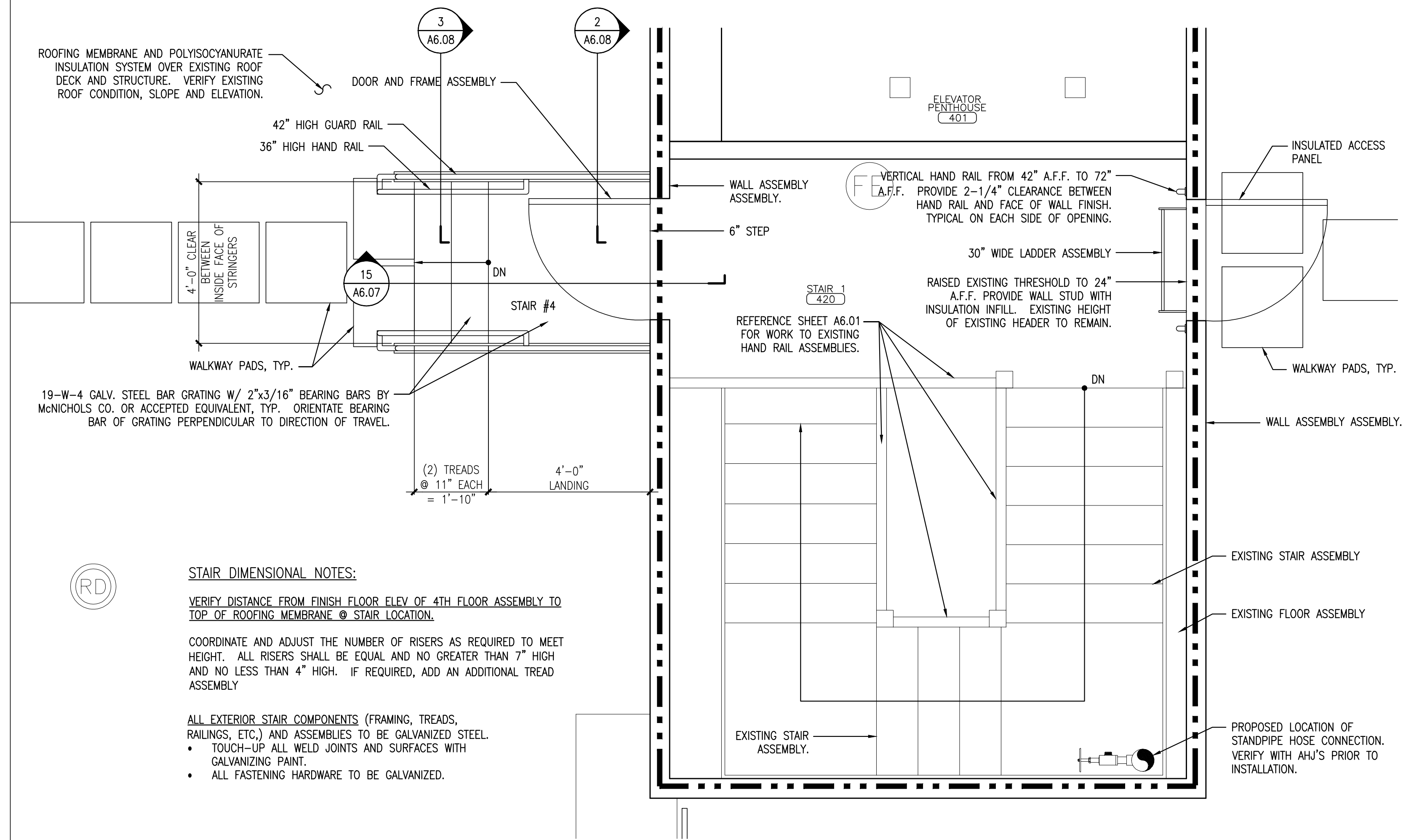
7 ENLARGED PLAN @ STAIR #4 AND 4TH FLOOR.
