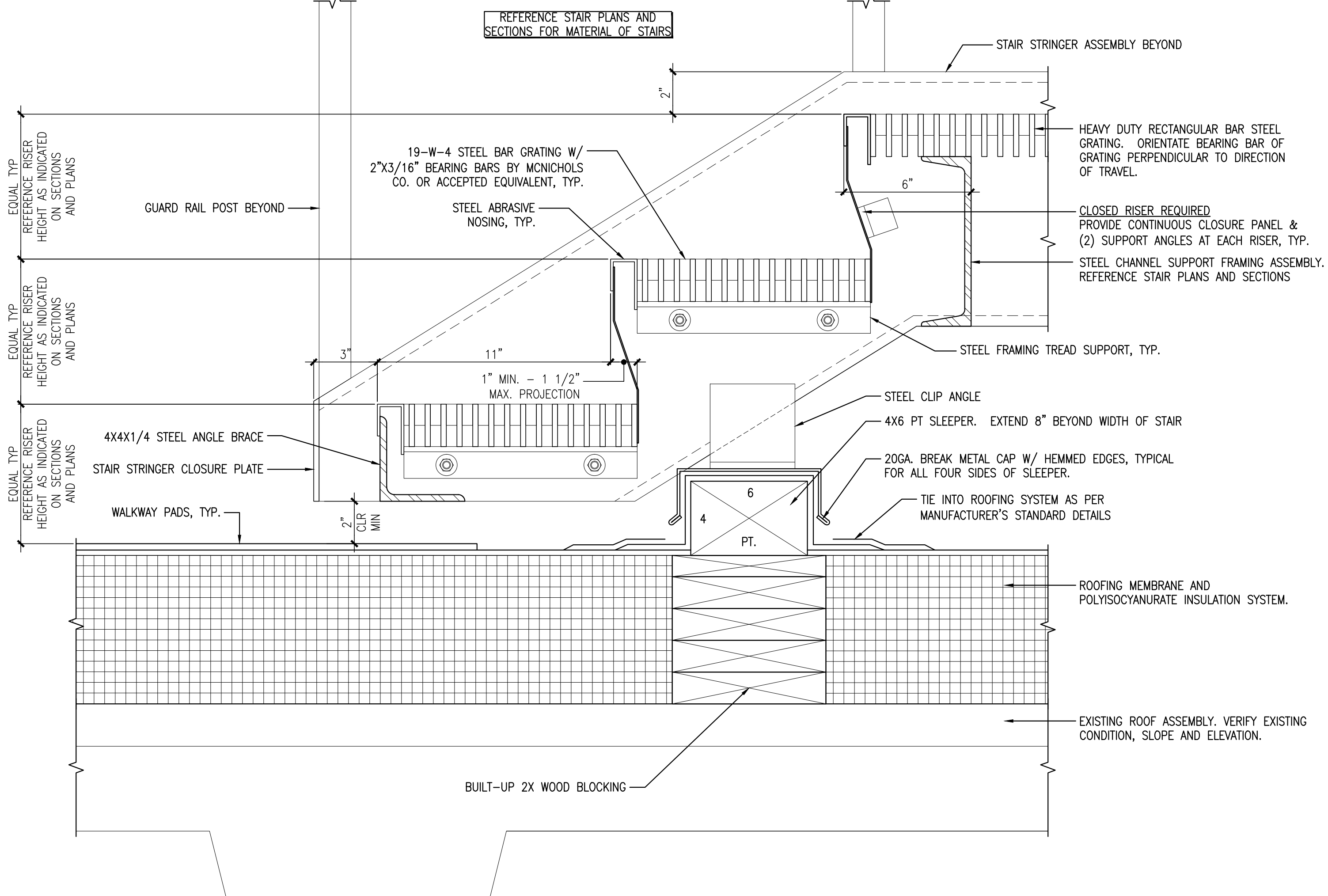
13 DETAIL @ STAIR #4
