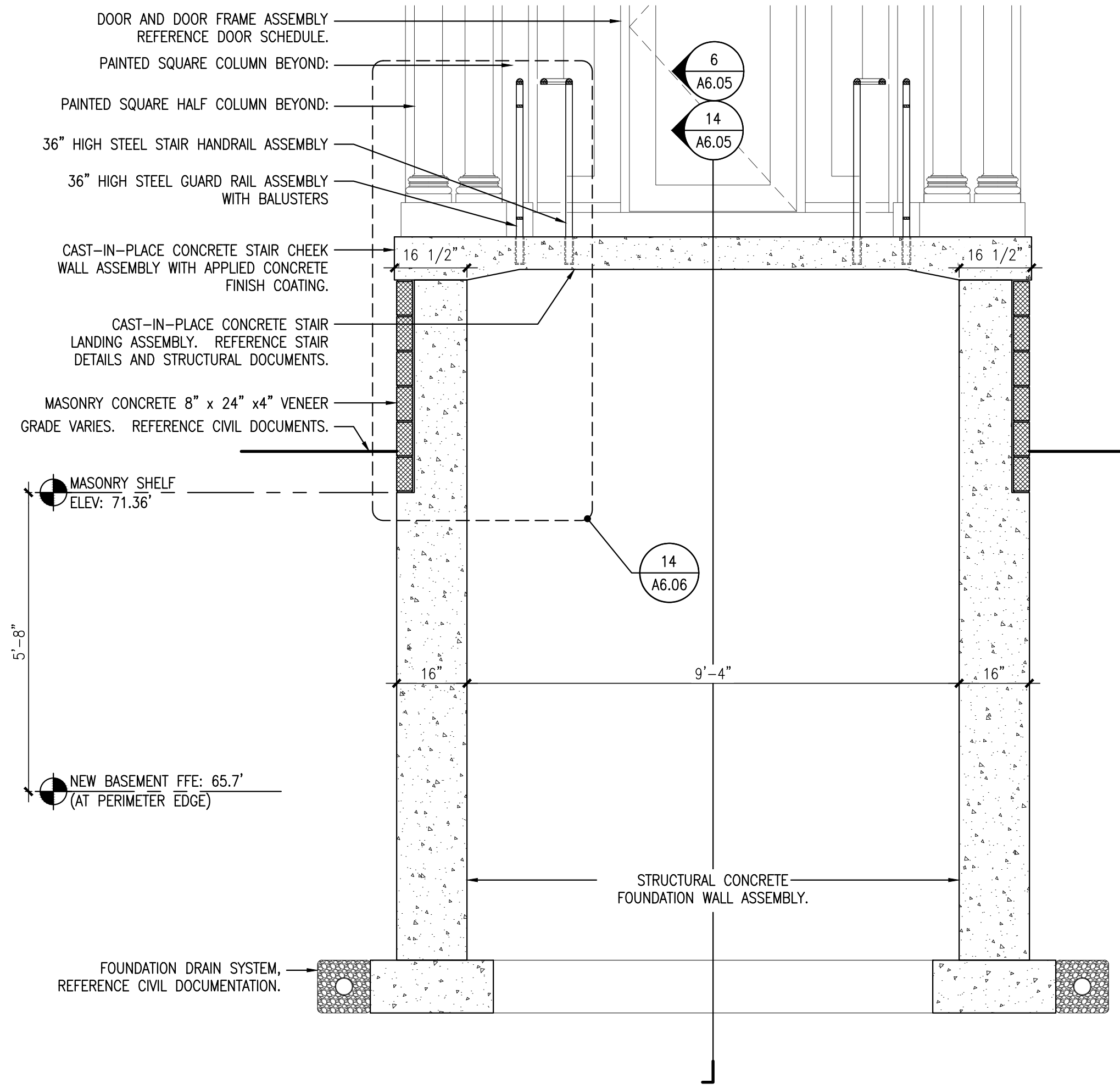
5 STAIR SECTION @ EXTERIOR STAIR #3 REFERENCED FROM: SCALE: 1/2" = 1'-0"
