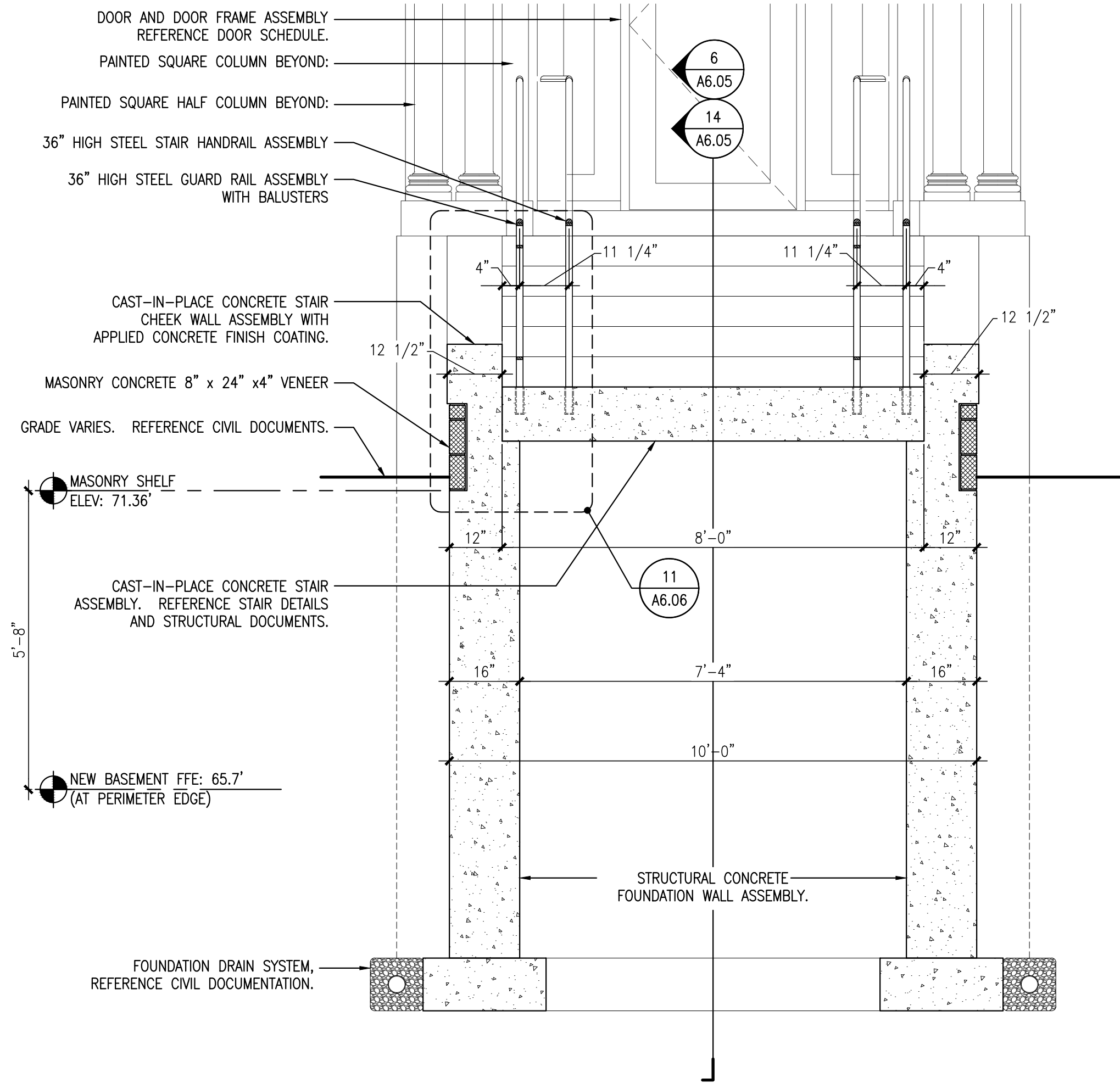
13 STAIR SECTION @ EXTERIOR STAIR #3 REFERENCED FROM: SCALE: 1/2" = 1'-0"
