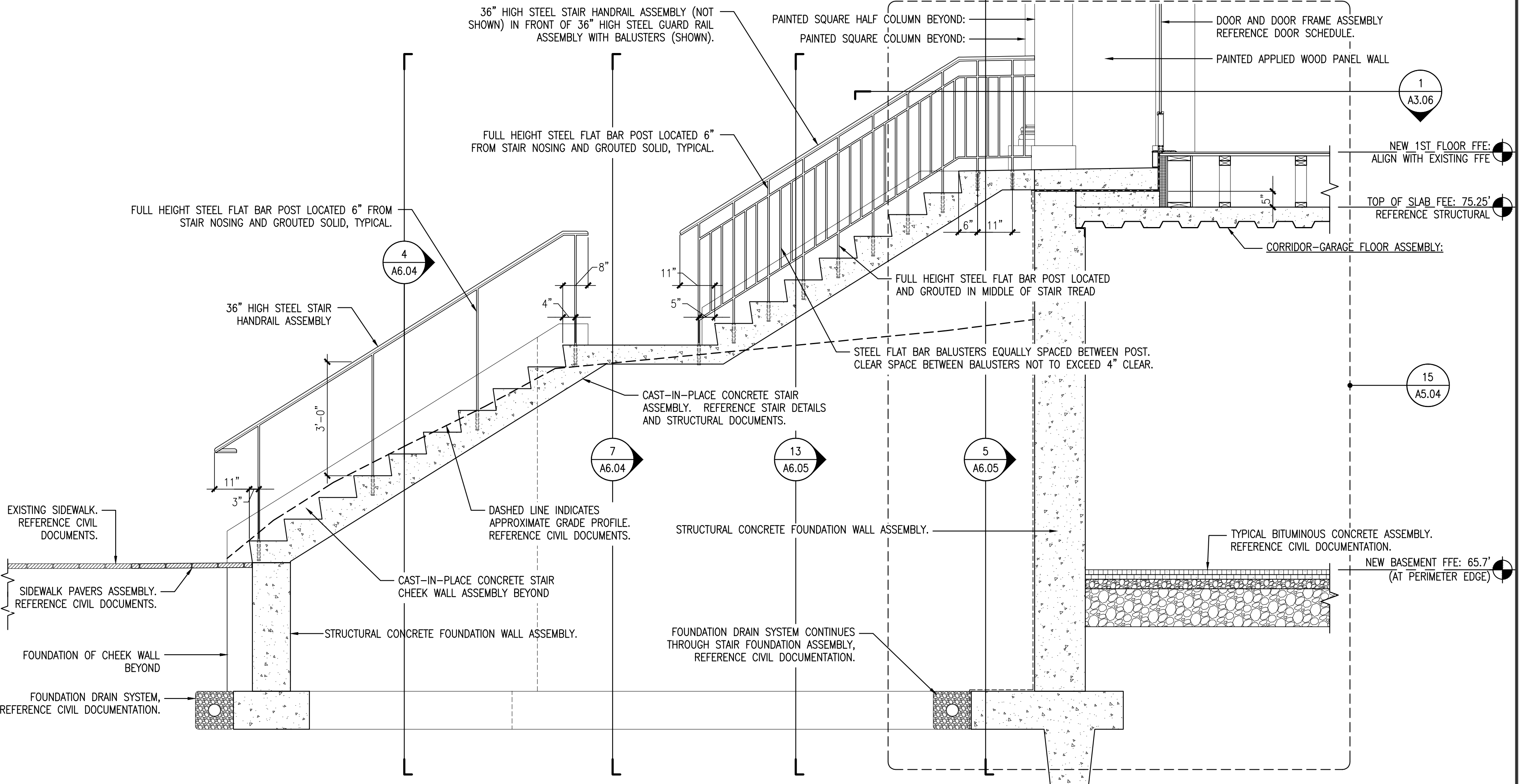
6 STAIR SECTION @ EXTERIOR STAIR #3 - HANDRAIL CONSTRUCTION REFERENCED FROM: SCALE: 1/2" = 1'-0"
