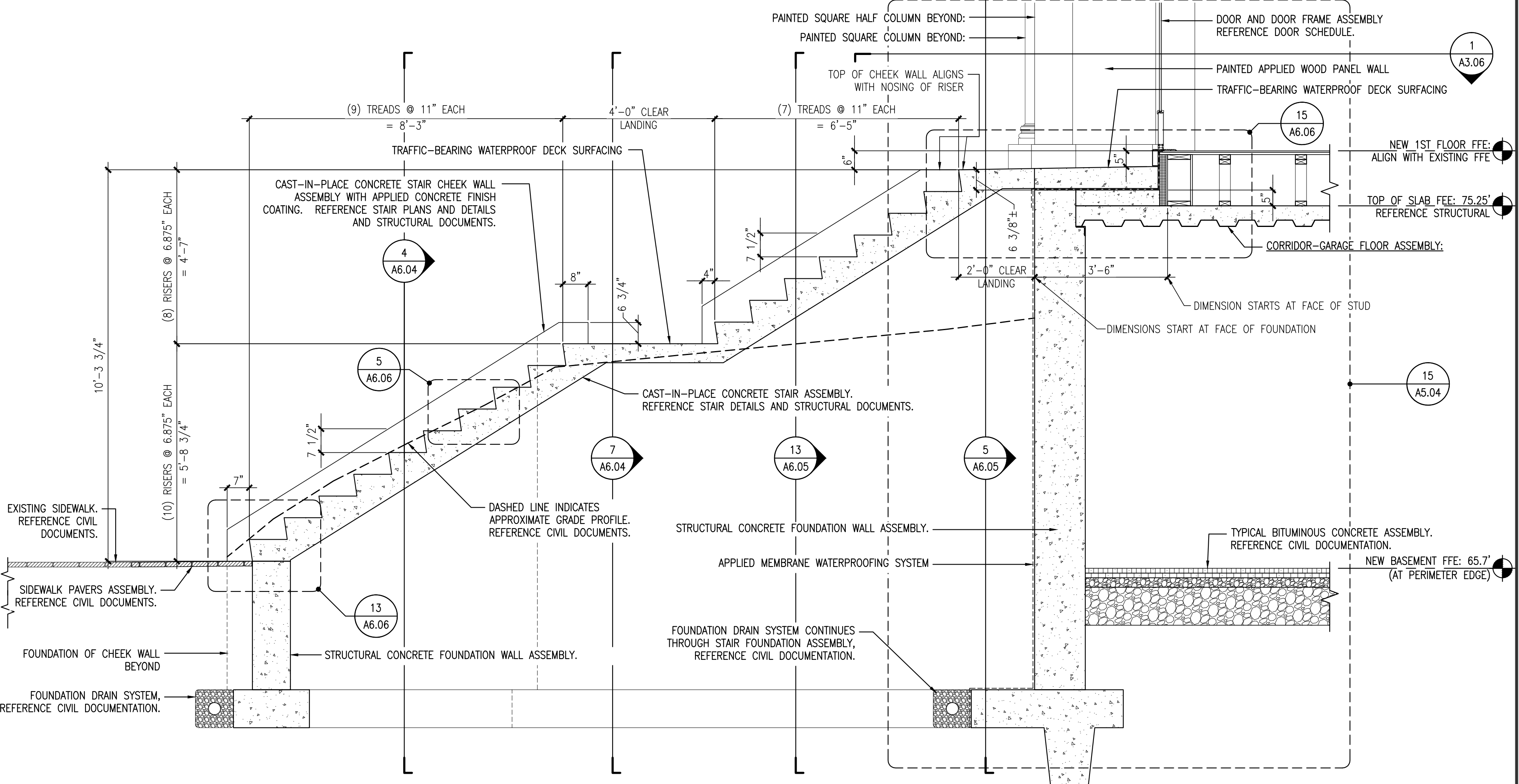
14 STAIR SECTION @ EXTERIOR STAIR #3 - STAIR CONSTRUCTION REFERENCED FROM: SCALE: 1/2" = 1'-0"
