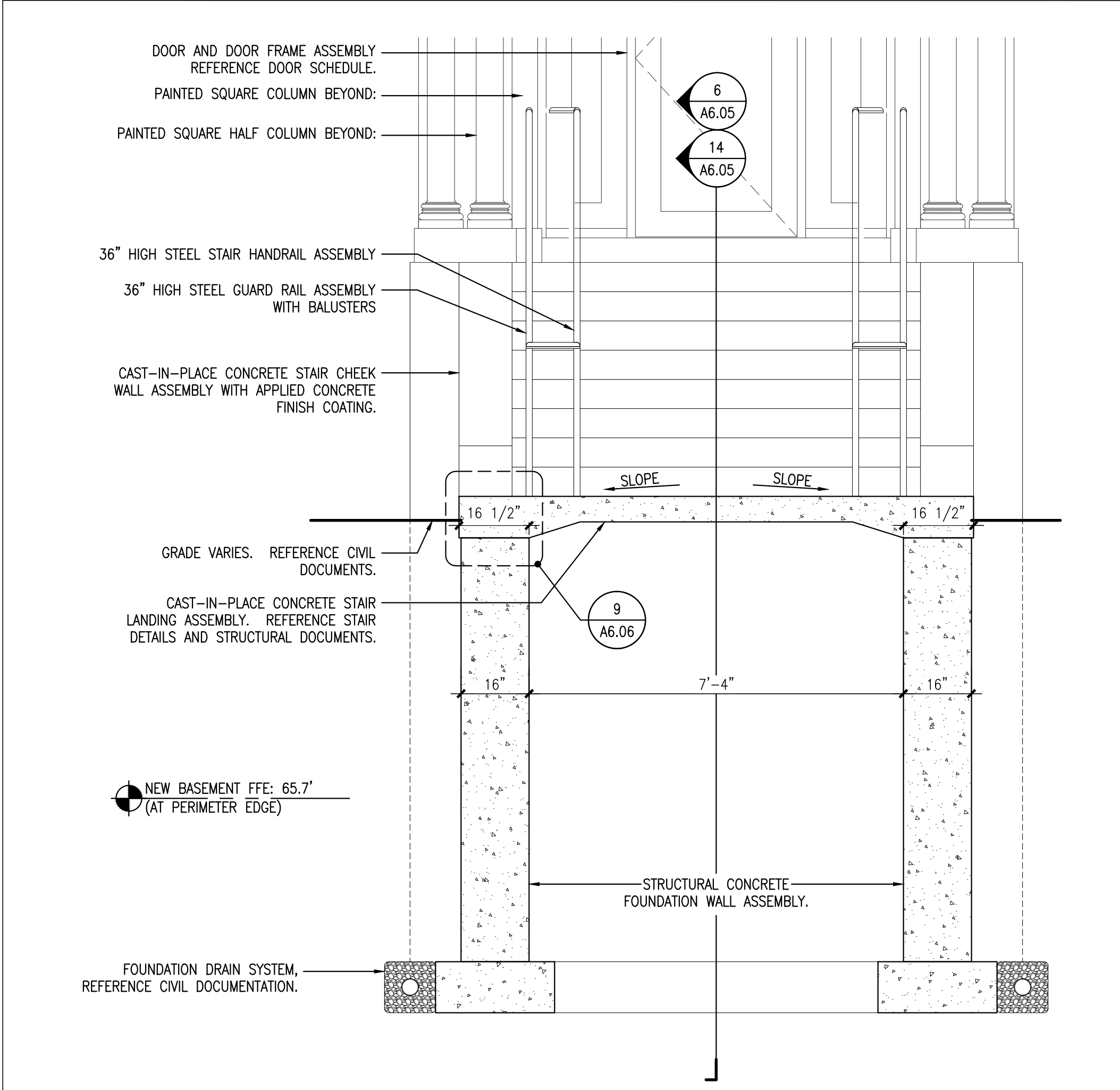
7 STAIR SECTION @ EXTERIOR STAIR #3 REFERENCED FROM: SCALE: 1/2" = 1'-0"
