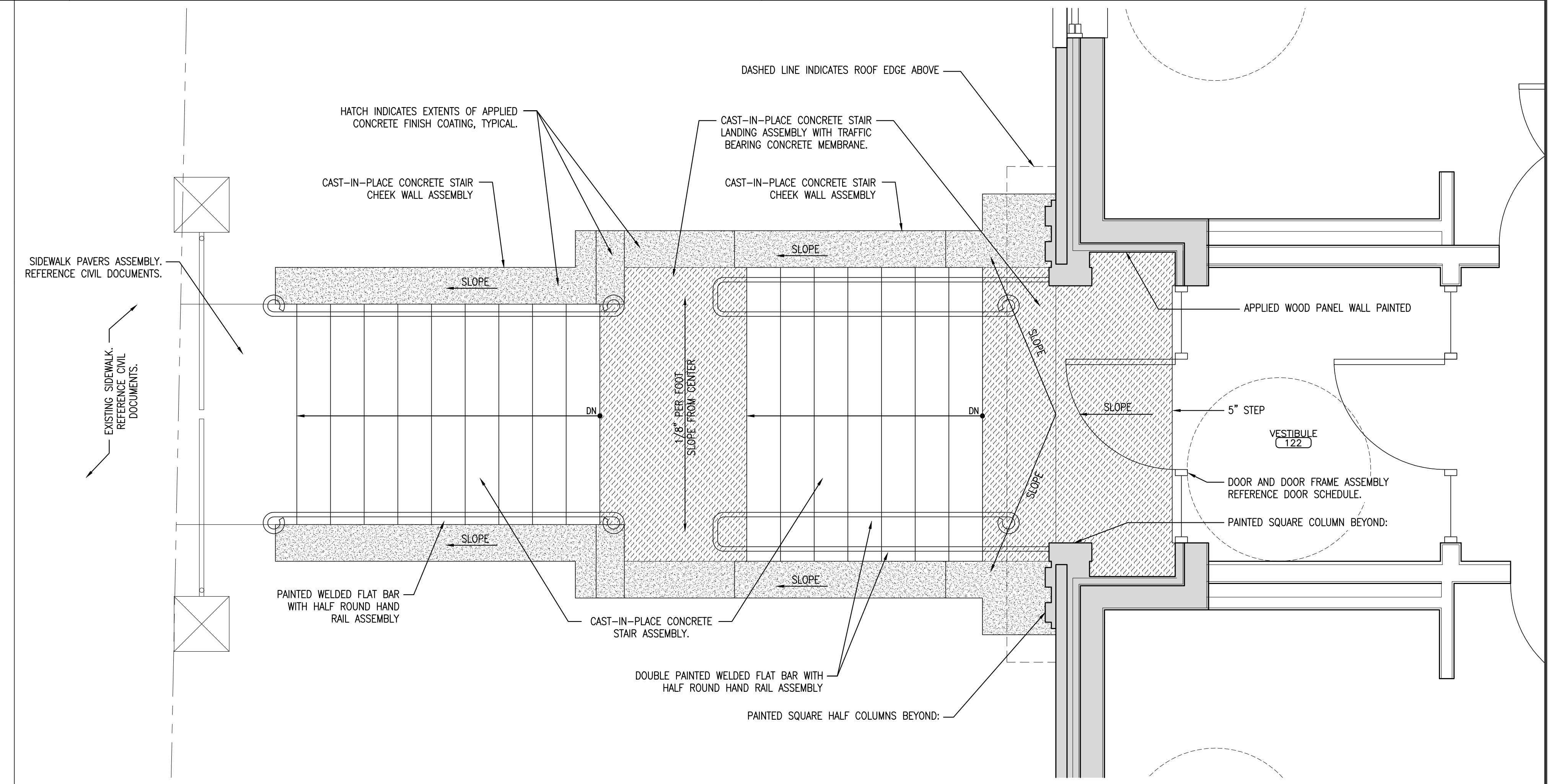
8 ENLARGE STAIR PLAN @ EXTERIOR STAIR #3 - LAYOUT REFERENCED FROM: SCALE: 1/2" = 1'-0"
