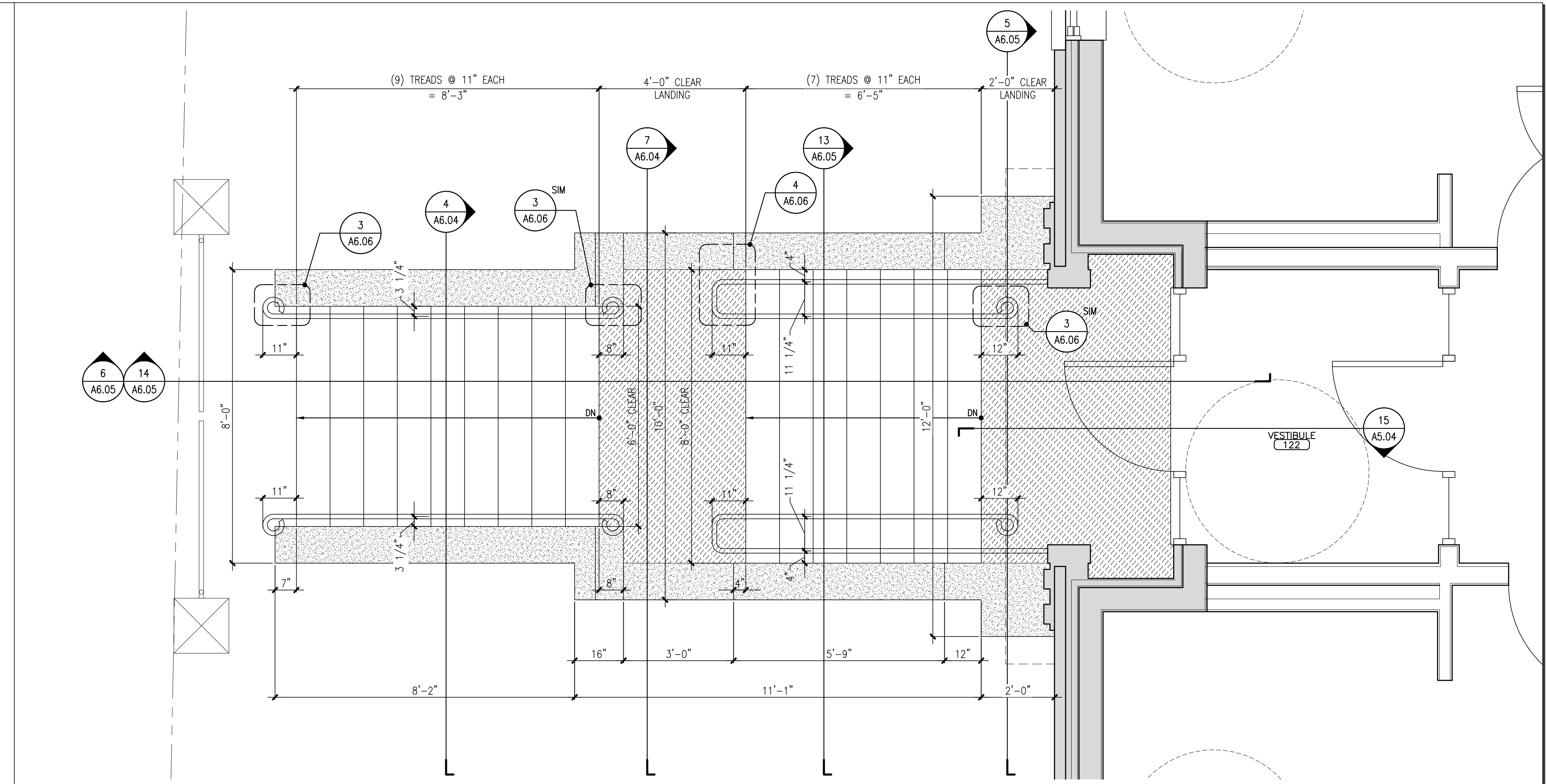
5 ENLARGE STAIR PLAN @ EXTERIOR STAIR #3 - DIMENSIONAL REFERENCED FROM: SCALE: 1/2" = 1'-0"
