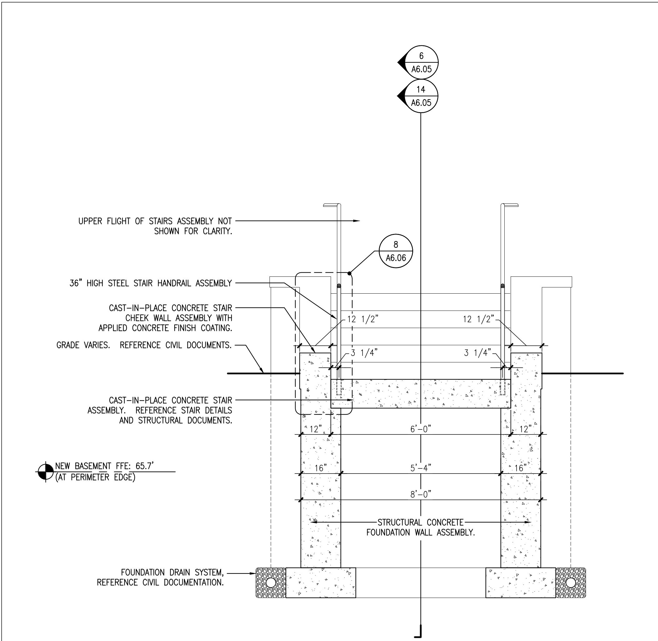
4 STAIR SECTION @ EXTERIOR STAIR #3 REFERENCED FROM: SCALE: 1/2" = 1'-0"
