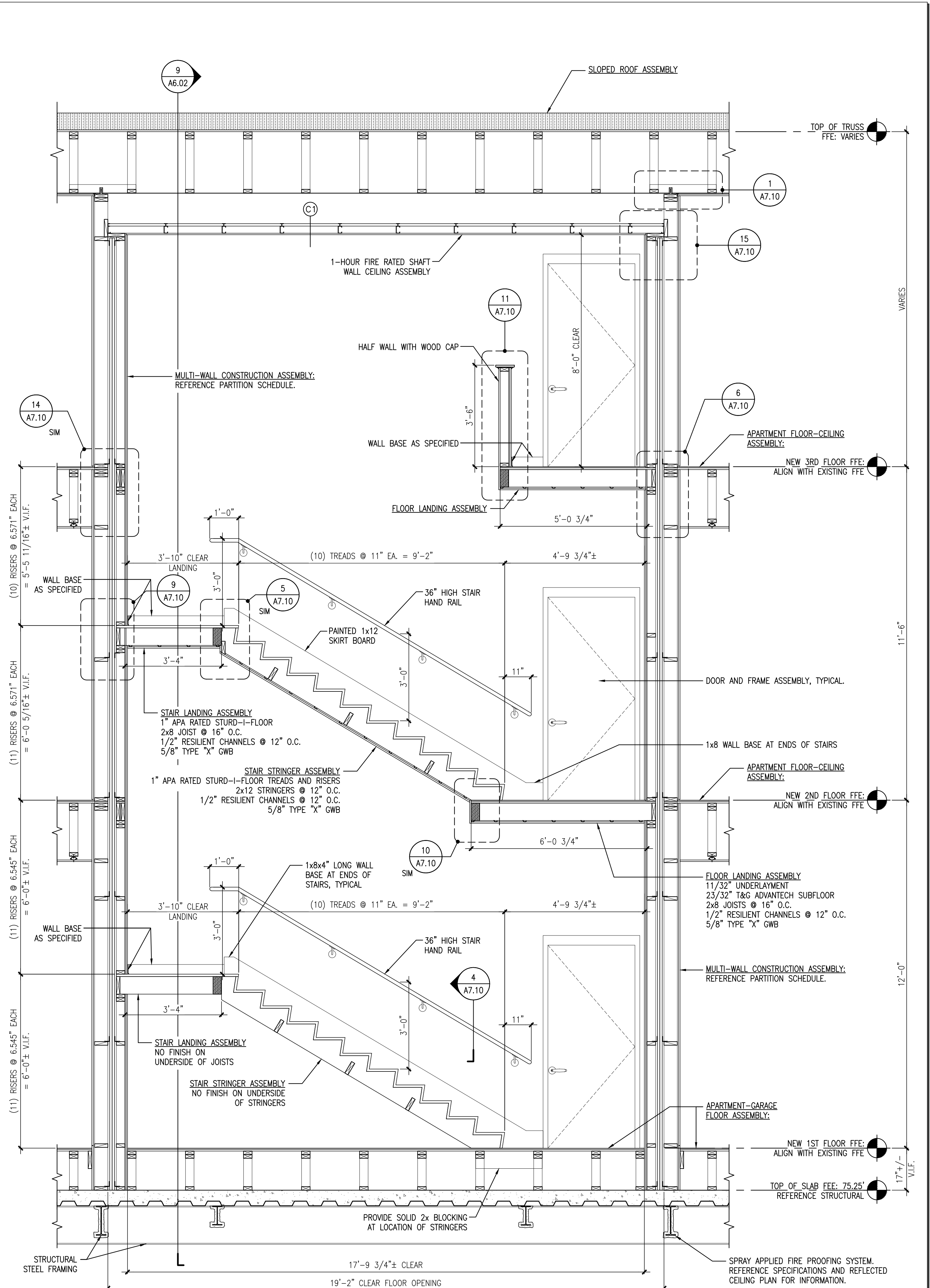
11 STAIR SECTION @ STAIR #2 REFERENCED FROM: SCALE: 1/2" = 1'-0"
