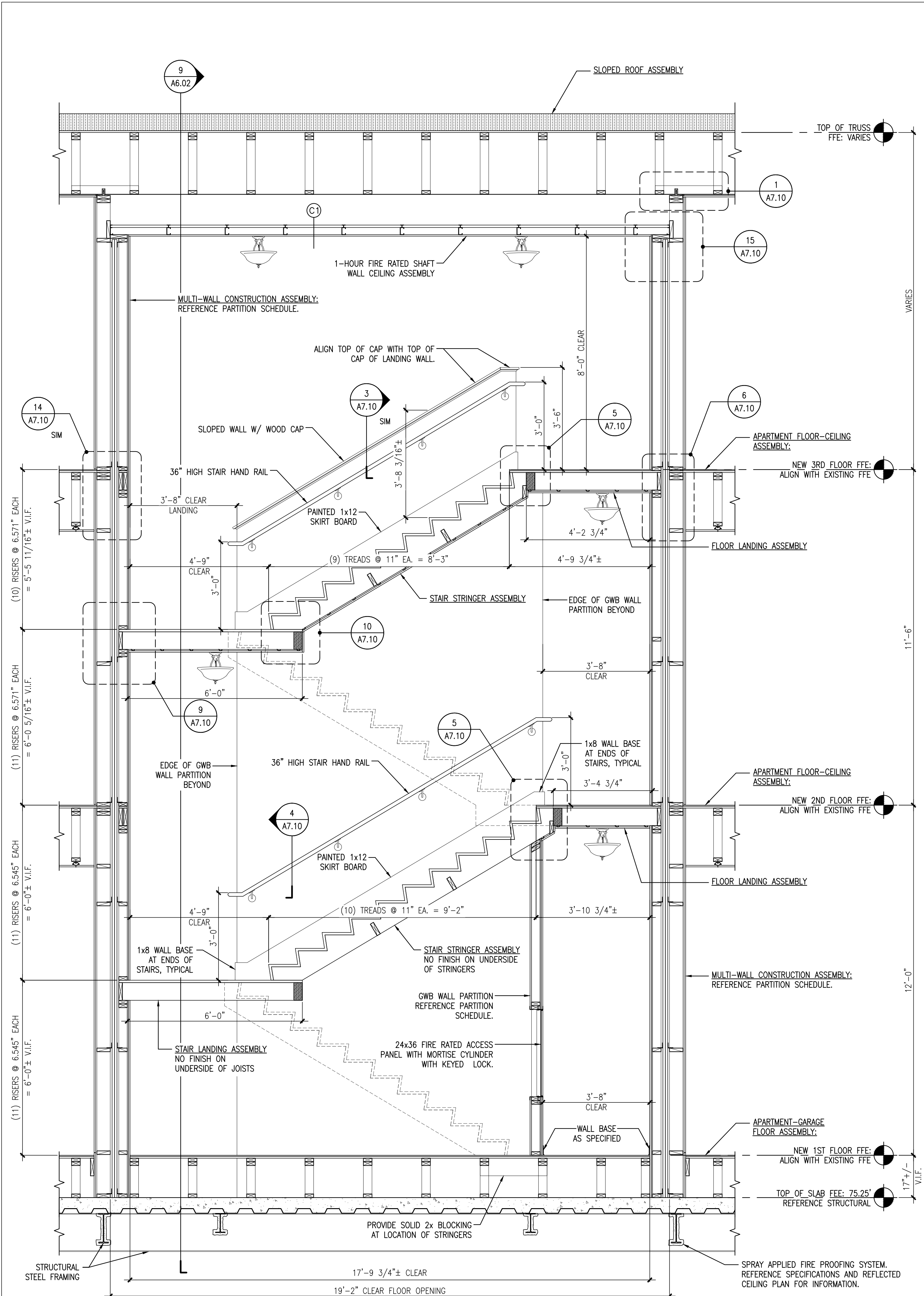
9 STAIR SECTION @ STAIR #2 REFERENCED FROM: SCALE: 1/2" = 1'-0"
