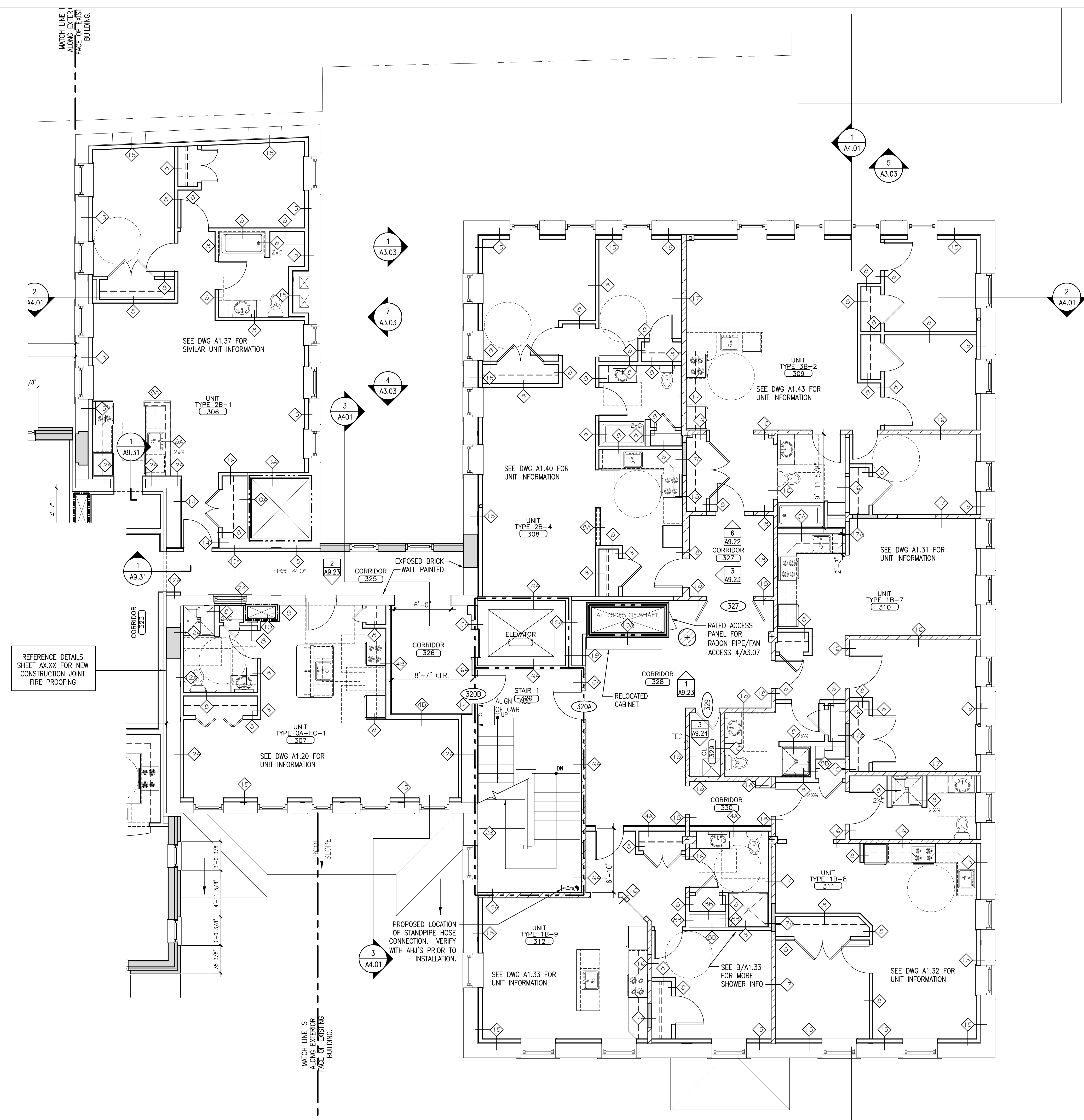
1 ENLARGED THIRD FLOOR PLAN - EXISTING BUILDING
