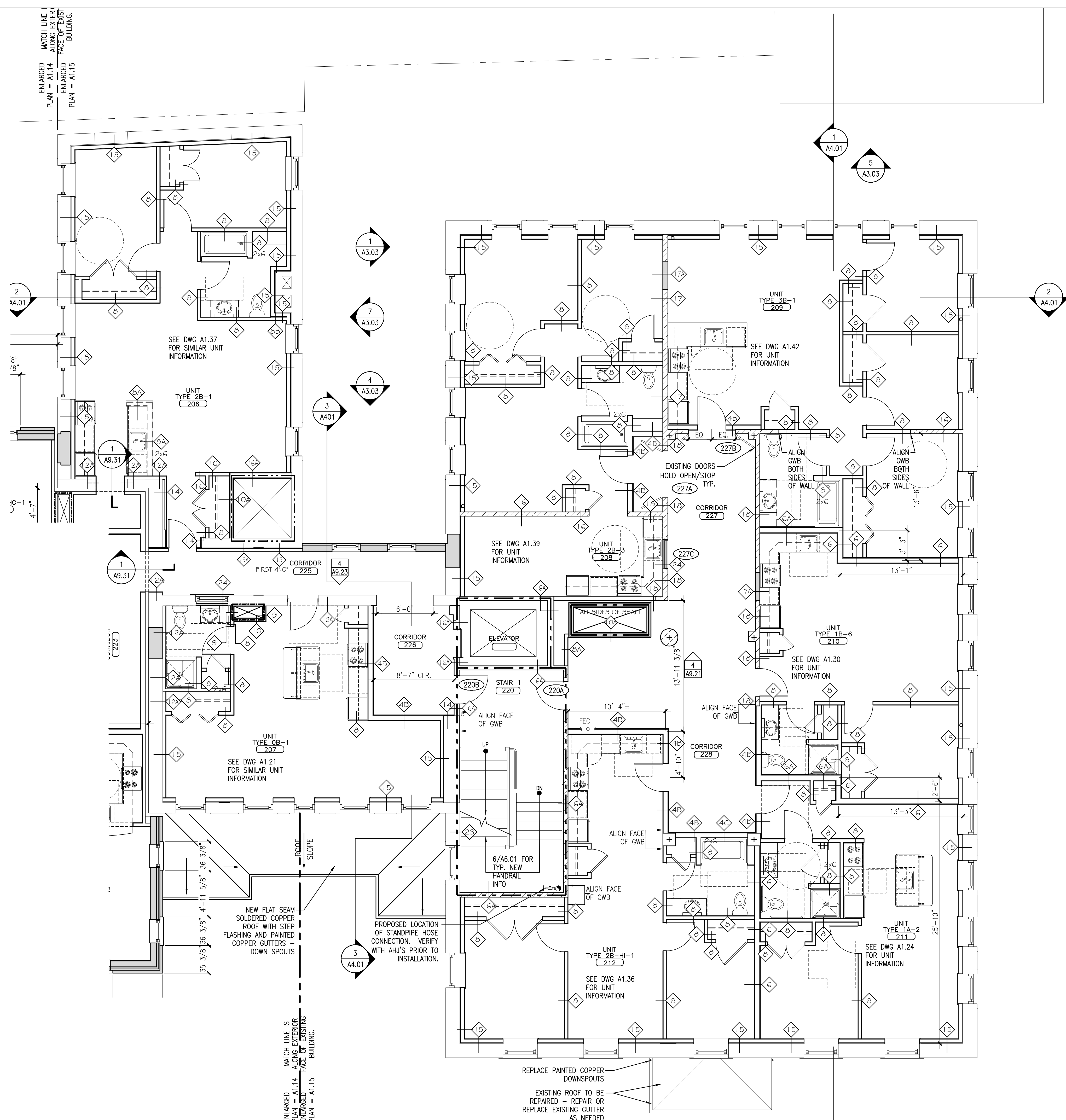
1 ENLARGED SECOND FLOOR PLAN - EXISTING BUILDING
