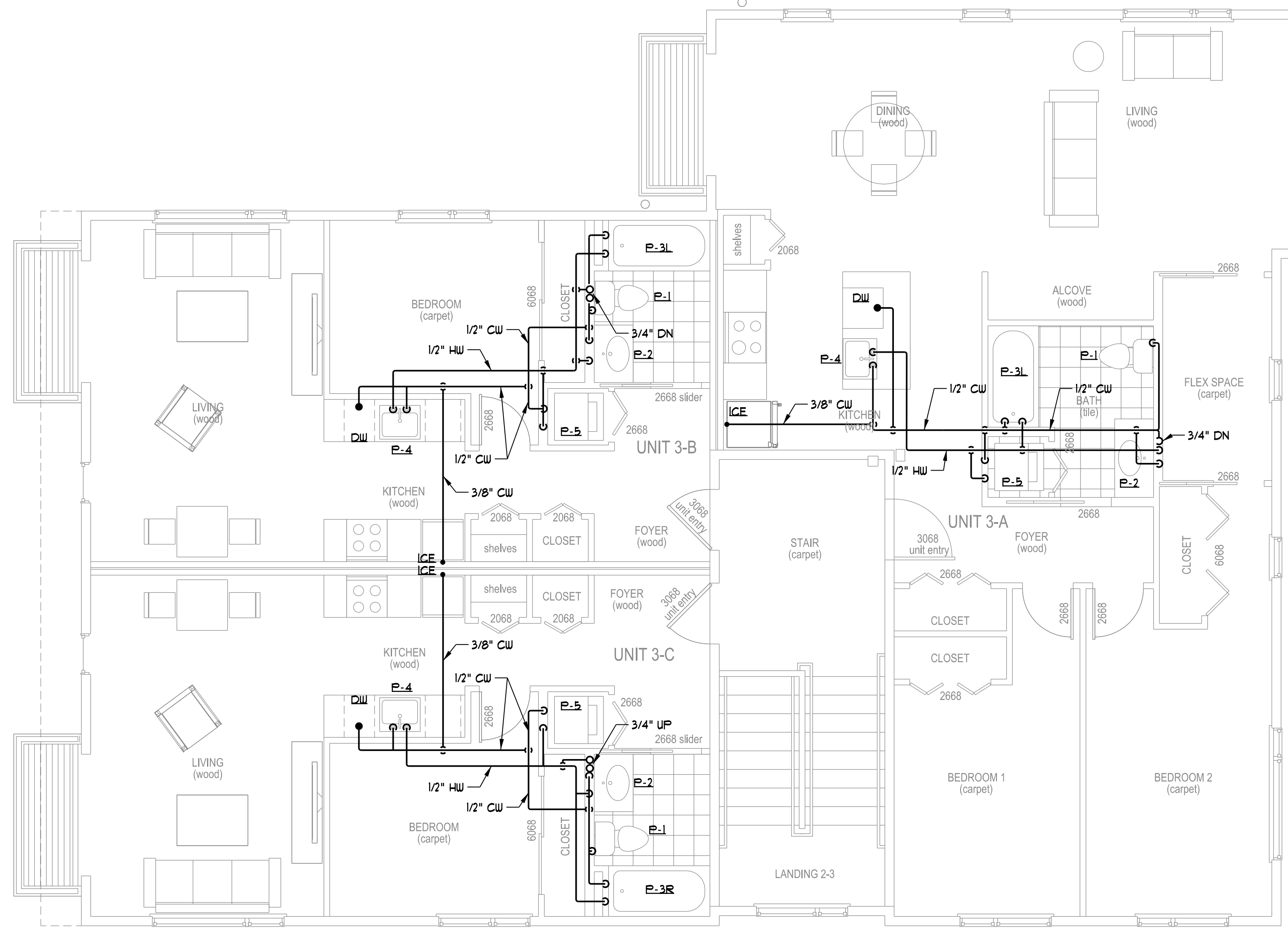
THIRD FLOOR PLAN SCALE 1/4" = 1'-0"
