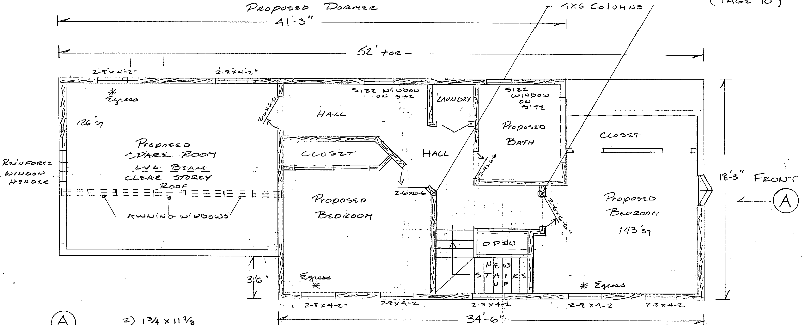
3RD FLOOR PROPOSED DORMER (OPTION #1) SCALE 1/4" = 1'
