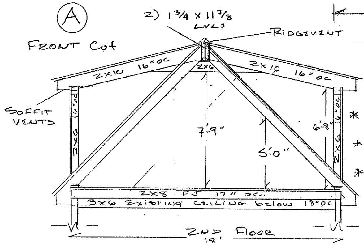
3RD FLOOR PROPOSED DORMER (OPTION #1) SCALE 1/4" = 1'
