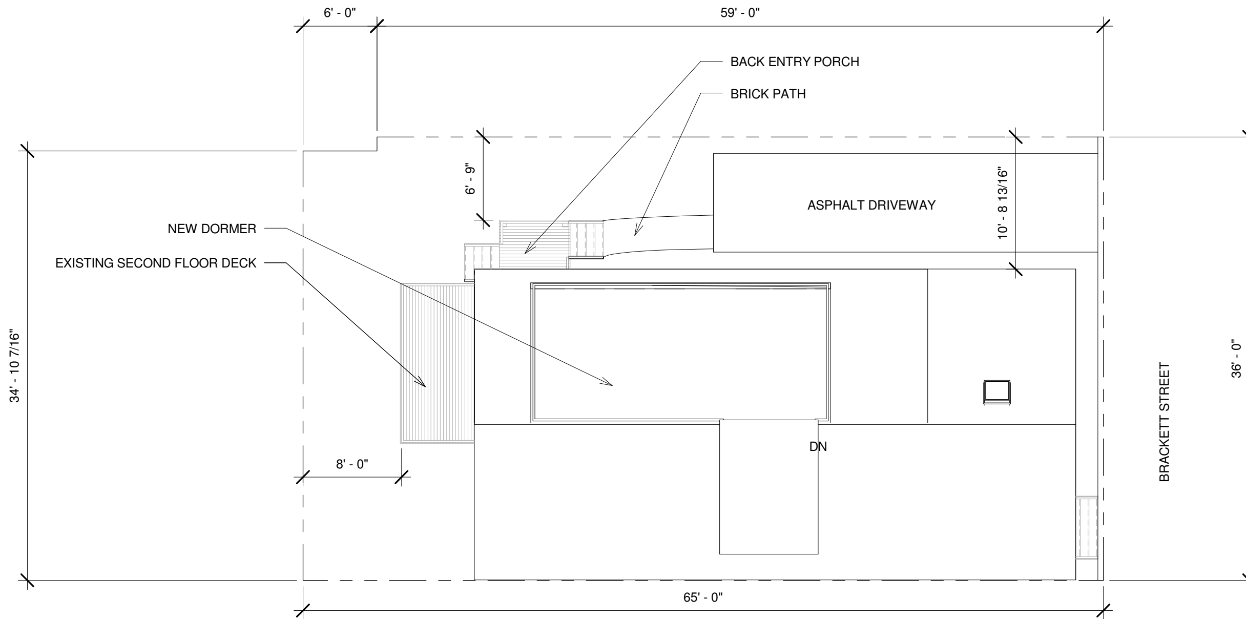
1 Site Plan 1/8" = 1'-0"
