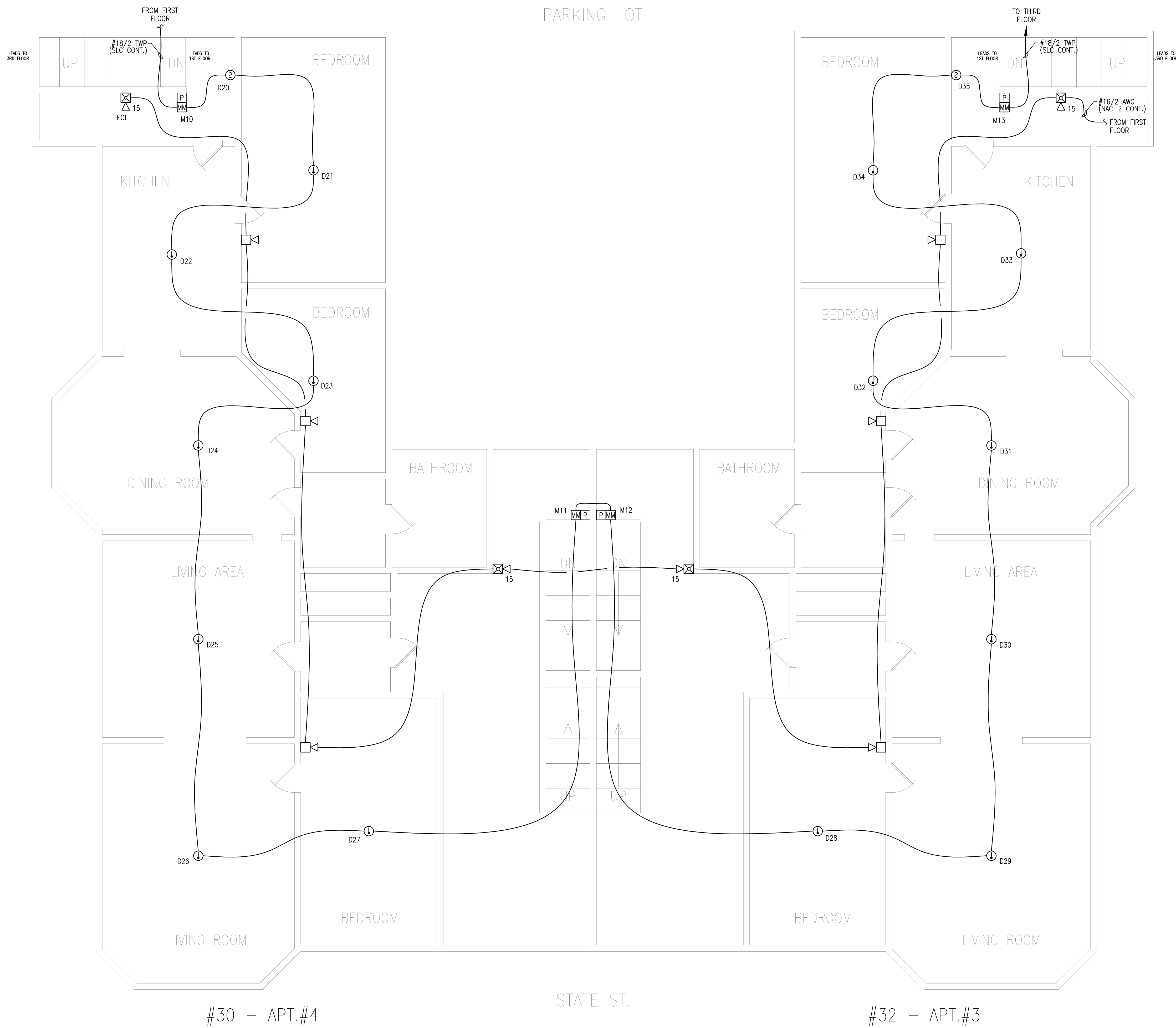
SECOND FLOOR FIRE ALARM PLAN SCALE: 1/4"=1'-0" FIELD VERIFY DIMENSIONS
