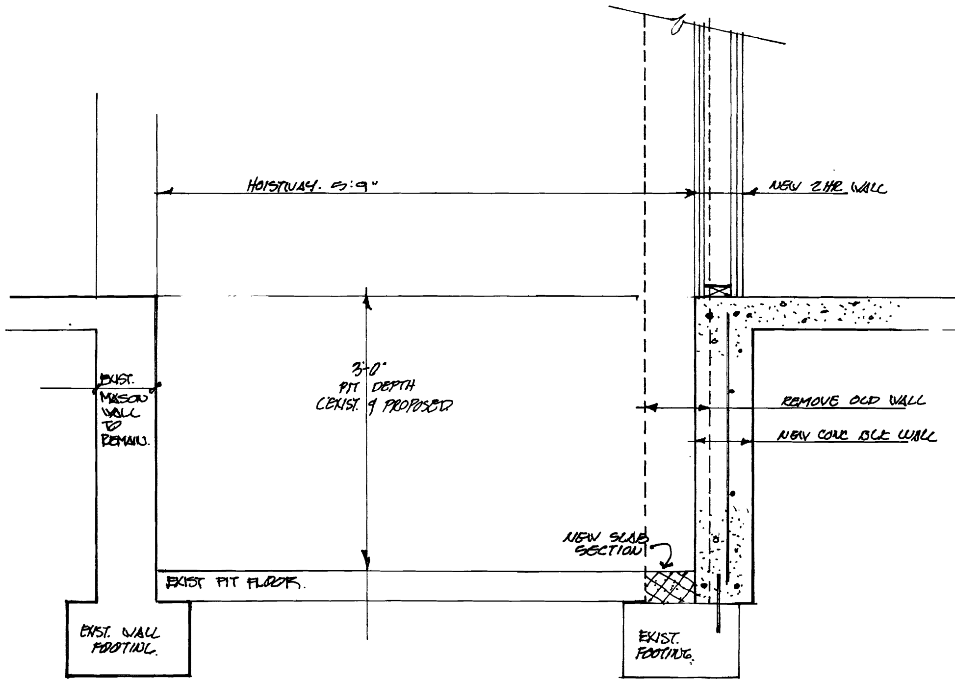
SECTION @ 1/2" = 1'-0"
